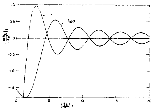
Fig. 18. The two kernels I_J and I_{qp0} in the time-domain formulation of the microscopic theory.
