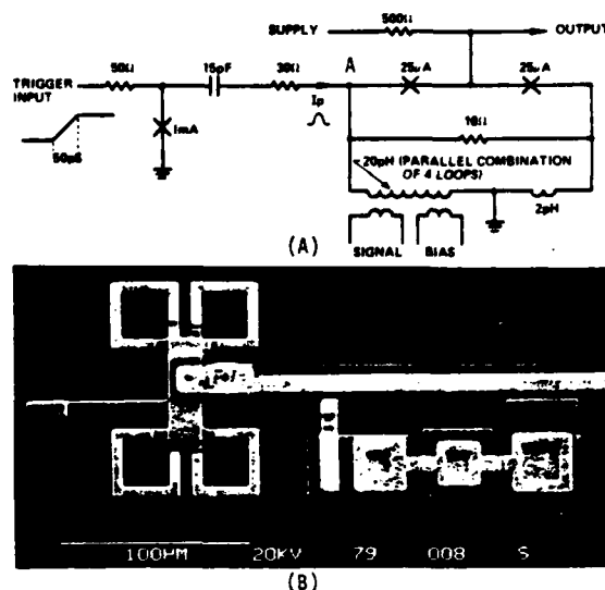
Fig. 4(a) The sampling circuit diagram and (b) a photograph of the circuit.
