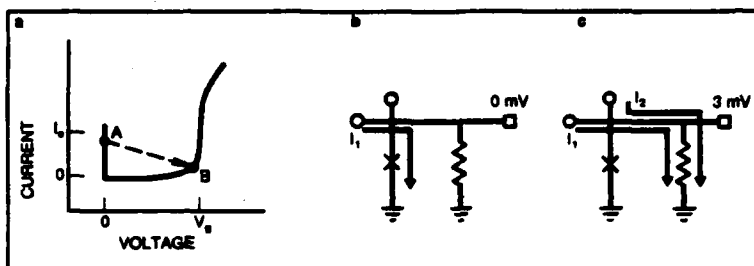
Switching of a simple AND gate. Initially only one current I_1 is present. It has a magnitude less than I_c ; also the Josephson junction is in state A of the current-voltage characteristic shown in part a. The path of this current in the AND circuit, shown in color in part b, is entirely through the junction, and the result is a zero voltage output. If a second current, I_2 , of comparable magnitude is also applied, the critical current of the junction is exceeded and it switches to the energy gap voltage V_g . In this situation the current in the junction after switching depends on the value of the load resistance. If the resistance is properly selected the junction will switch to point B of the characteristic (a), where the junction current is much less than in the zero voltage state. Thus, to a good approximation, both input currents are directed to the load resistance, as in part c, resulting in a 3-mV output. The circuit is reset to zero voltage by reducing I_1 and I_2 to zero.
