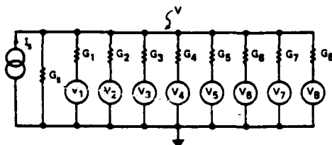
Fig. 9. Equivalent circuit for the A/D converter power supply.
