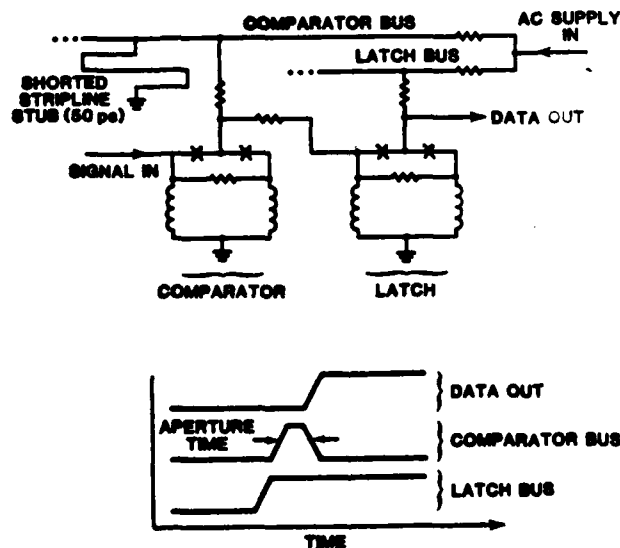
Fig. 3.1 (a) A circuit showing one bit of the A/D converter followed by a fast latch and (b) the timing diagram for this circuit.
