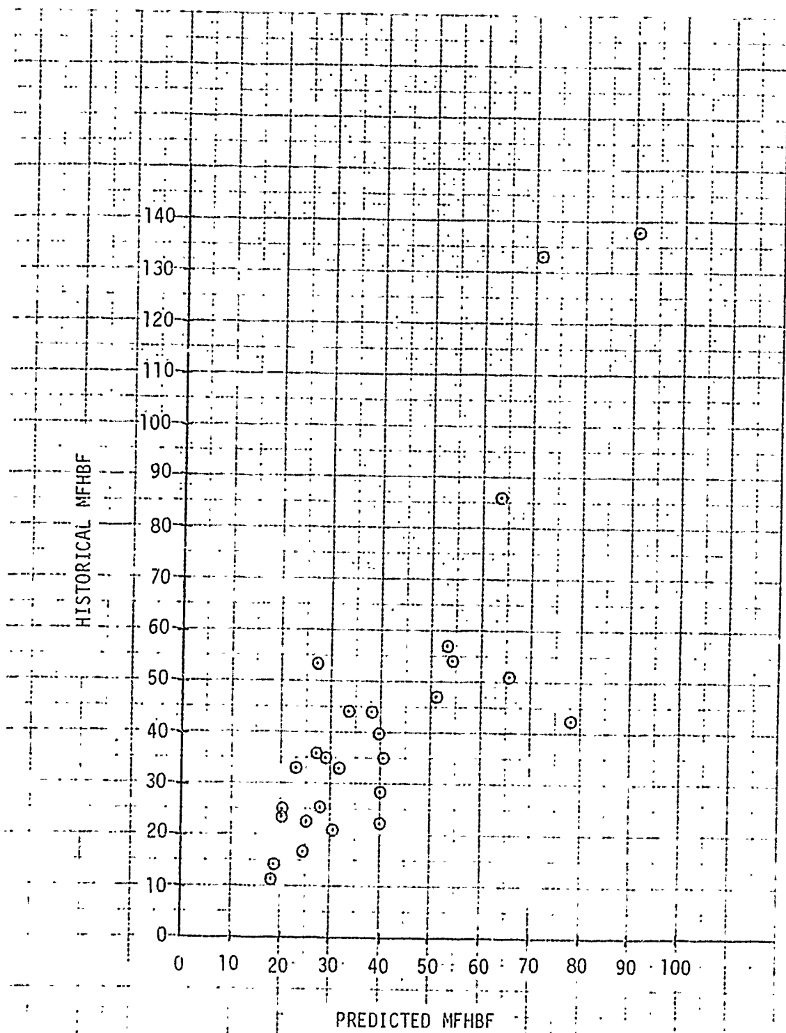
Figure 7-1 (Cont.). Predicted MFHBF vs Historical MFHBF For Fixed Wing Aircraft -- WUC 41000
