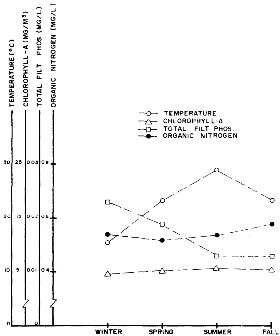
Figure 10. Correlation of selected parameters for sampling station 380455, Lake Conway East pool
