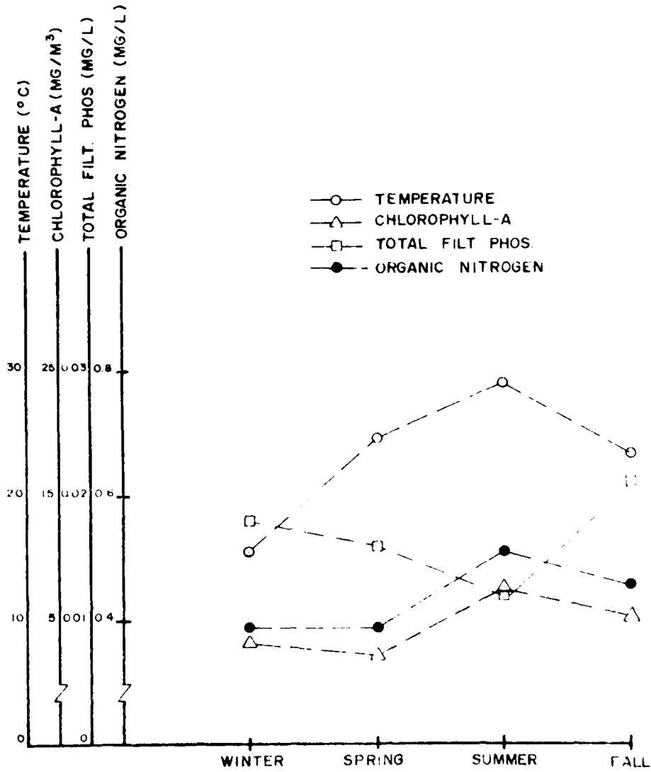
Figure 9. Correlation of selected parameters for sampling station 210302, Lake Conway Middle pool
