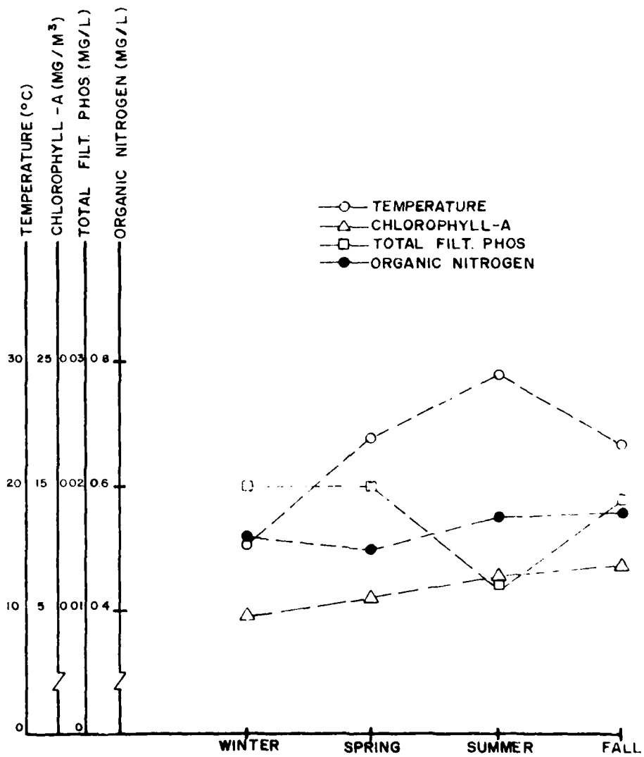
Figure 11. Correlation of selected parameters for sampling station 195382, Lake Conway West pool
