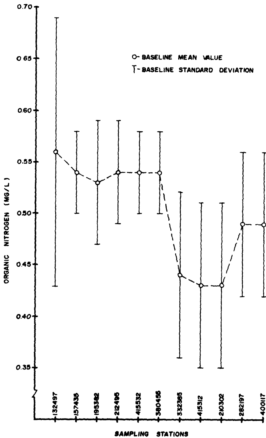
Figure 4. Trends in organic nitrogen concentrations
