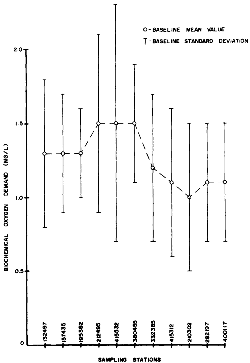
Figure 5. Trends in BOD concentrations
