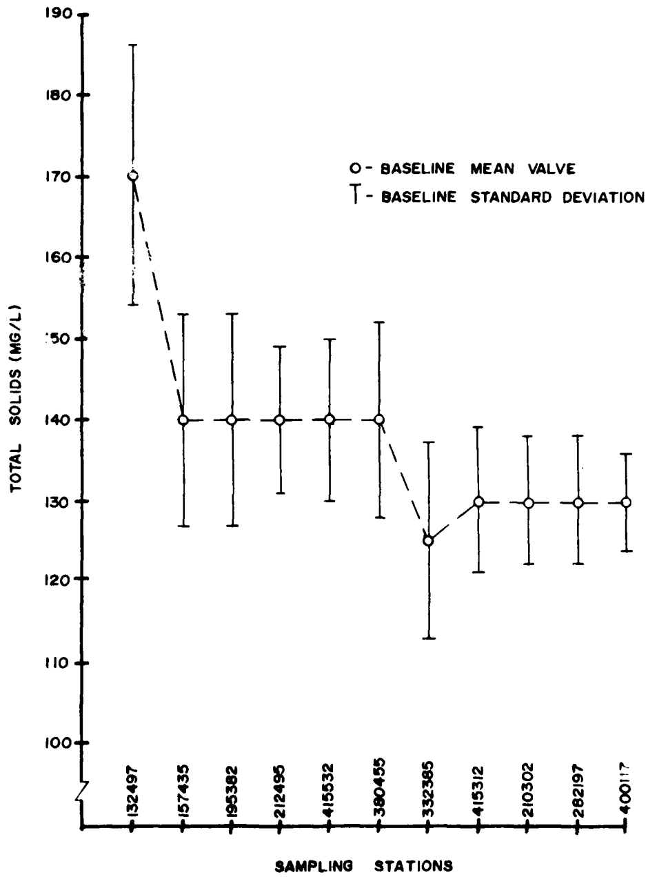
Figure 6. Trends in total solids concentrations
