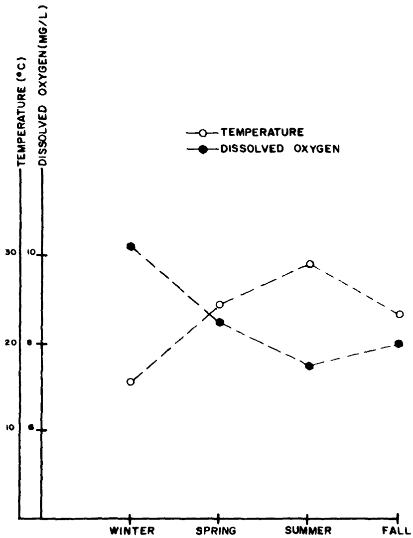
Figure 15. Comparison of dissolved oxygen versus temperature, Middle pool station 210302
