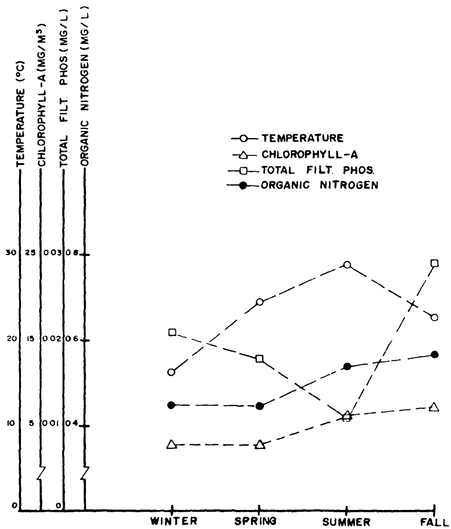
Figure 8. Correlation of selected parameters for sampling station 400117, Lake Conway South pool
