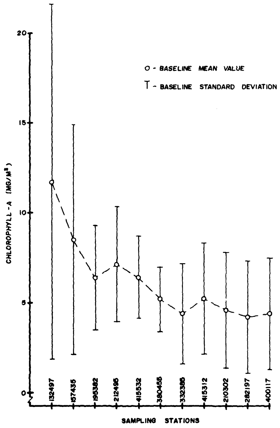
Figure 7. Trends in chlorophyll-a concentrations
