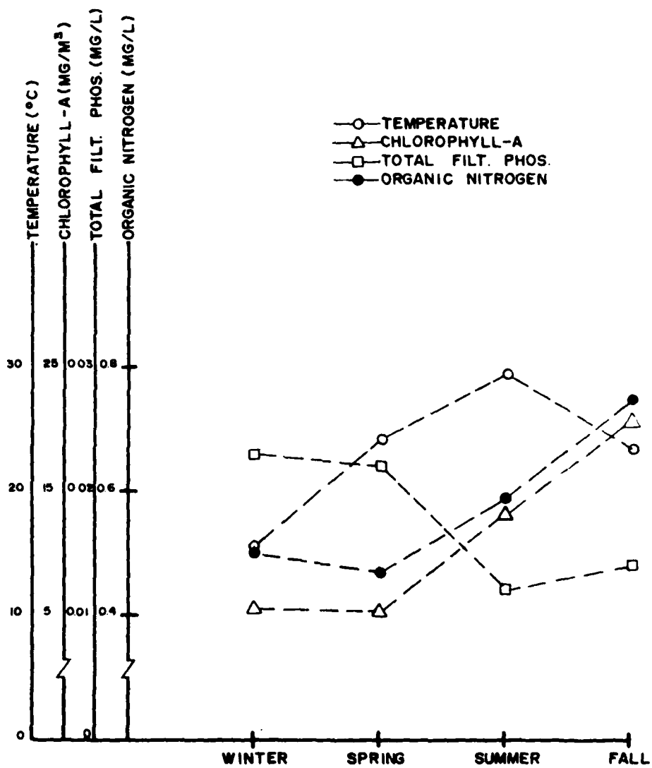
Figure 12. Correlation of selected parameters for sampling station 132497, Lake Gatlin
