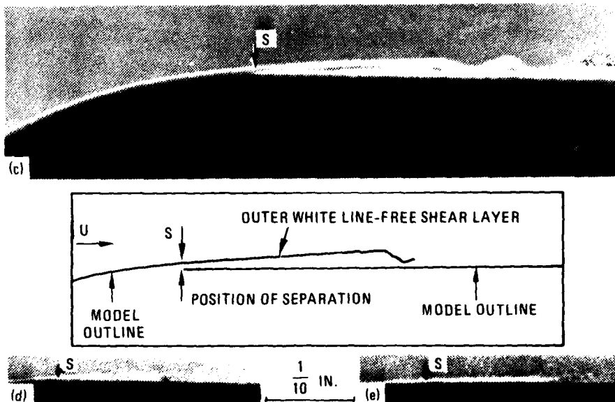
SILHOUETTE SCHLIEREN PHOTOGRAPHS, SHOWING LAMINAR SEPARATION UNDER NON-CAVITATING CONDITIONS. (c) 2 IN. HEMISPHERICAL NOSE MOUNTED IN THE FSWT ( R \sim 10^5 ). SOME DETAILS OF THE REATTACHMENT MECHANISM ARE ALSO OBSERVED. FLOW FROM LEFT TO RIGHT. ACTUAL LENGTH OF SEPARATED REGION \sim 0.25 \text{ IN.} (d) HEMISPHERICAL NOSE MOUNTED IN THE HSWT ( R = 6.04 \times 10^5 ). (e) SWEDISH HEADFORM MOUNTED IN THE HSWT ( R = 4.39 \times 10^5 ). SCALE SHOWN FOR (d), (e).
