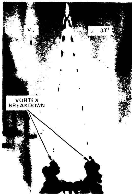
(b) PROGRESSION OF VORTEX BREAKDOWN ON AN ASPECT RATIO 0.71 WING
