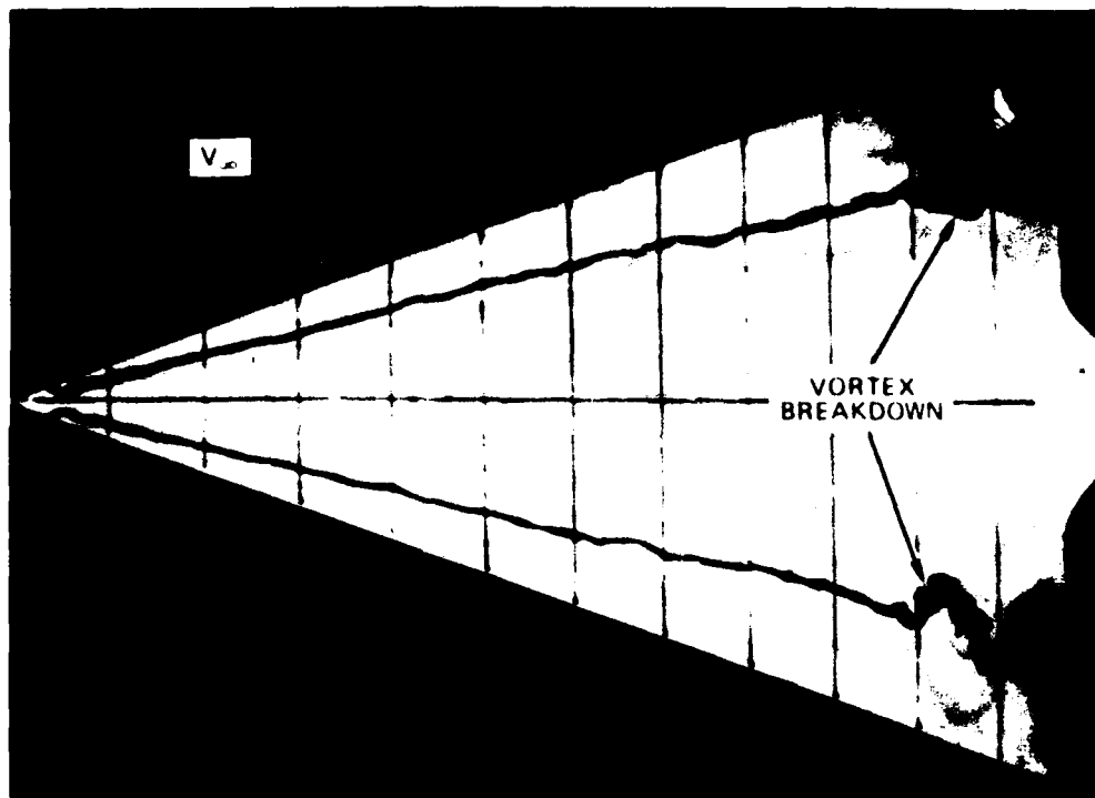
(a) TYPICAL VORTEX BREAKDOWN OVER AN ASPECT RATIO 1.46 WING
