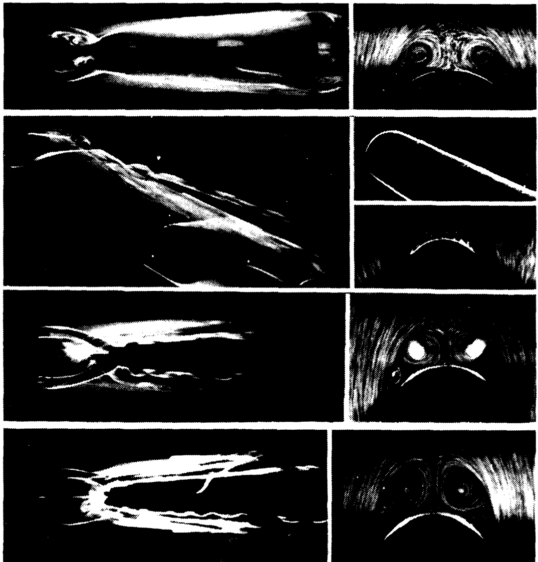
(b) FOREBODY VORTEX CHARACTERISTICS AT VARIOUS CROSS-SECTIONS.
