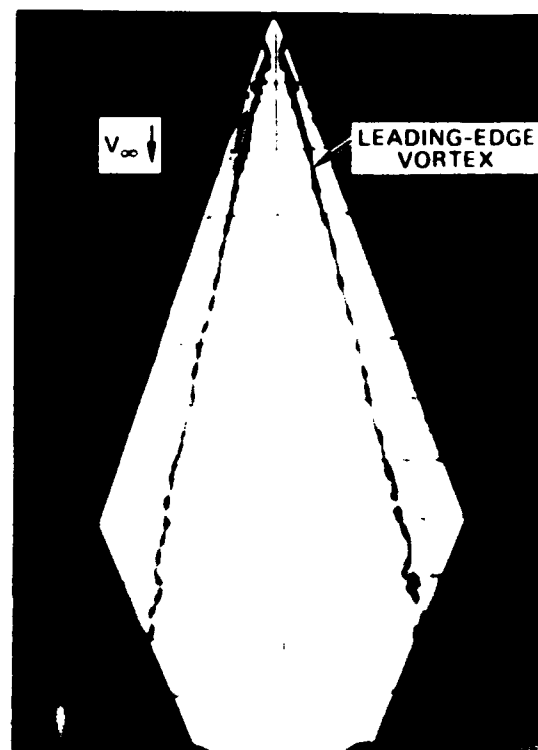
WATER TUNNEL
