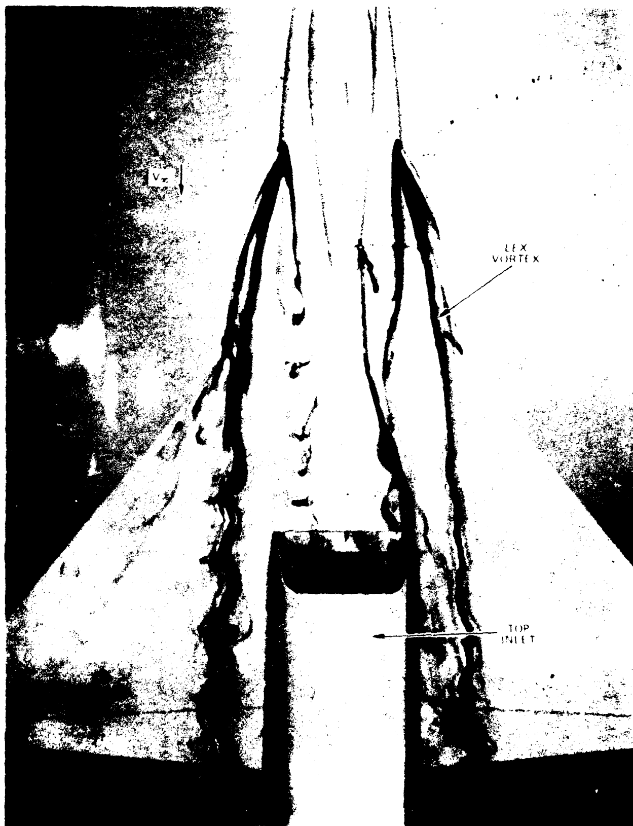
FIGURE 146. TOPSIDE INLET MODEL MOUNTED IN NORTHROP WATER TUNNEL AT LOW ANGLE OF ATTACK
