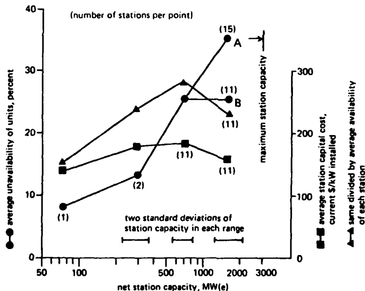
Figure 5.2: Average unavailability and specific capital cost vs. unit size in a nearly even-aged sample of 29 thermal power stations.
