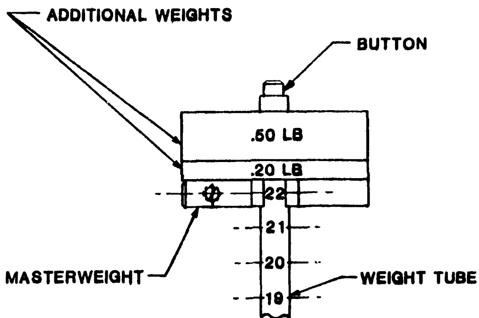
Figure 2. Appearance of weights loaded onto weight tube.
