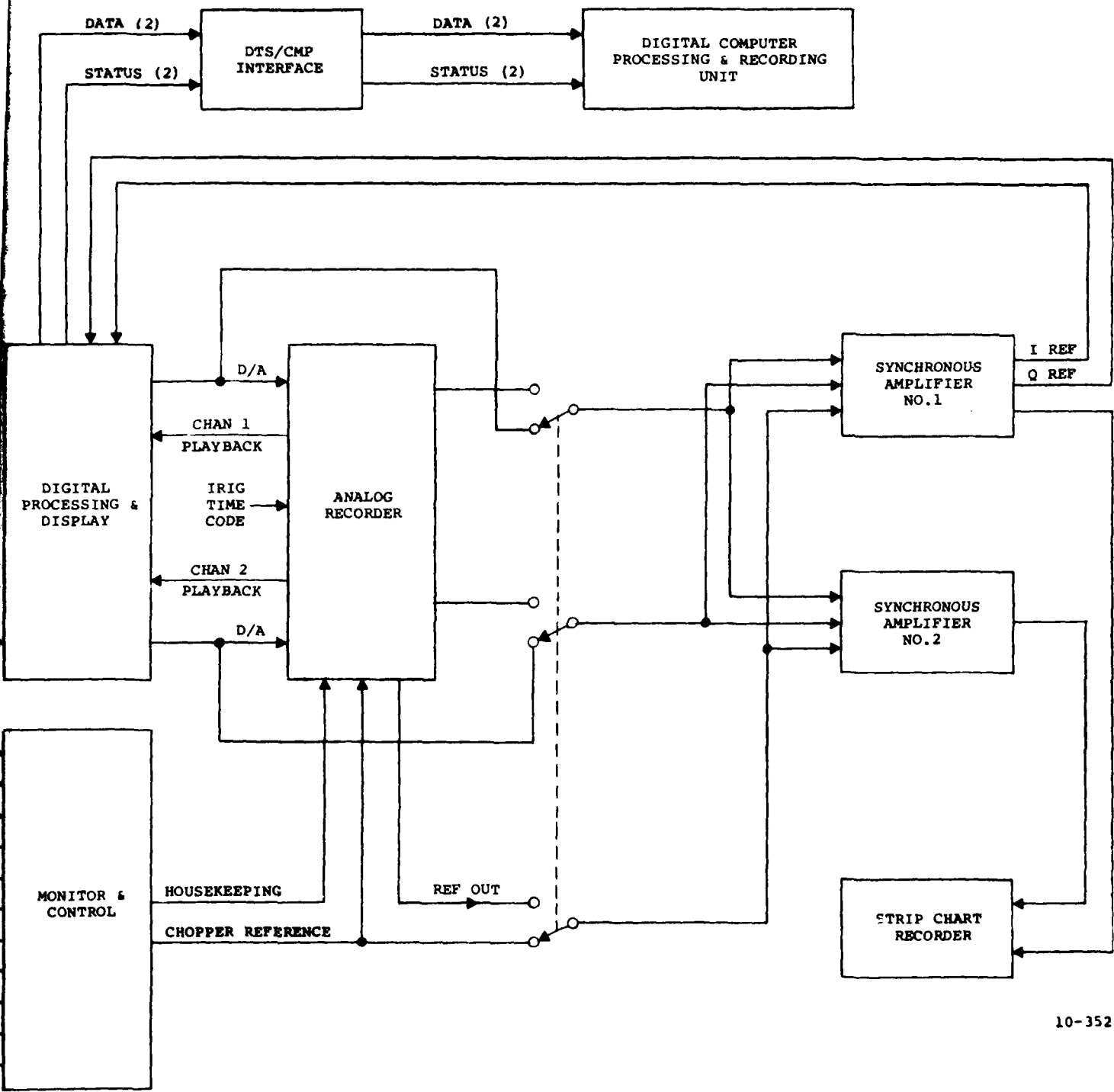
Figure 2-19. Contrast Mode Photometer functional block diagram.
