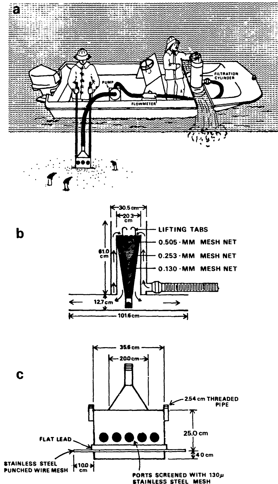
Fig. 7-1. Suction pump system utilized to quantitatively sample epibenthic zooplankton in shallow sublittoral and lower littoral habitats at Moon Island, Grays Harbor, Washington, May 27-28 1980; (a) system components in use, (b) filtration cylinder, and (c) sampling cylinder.
