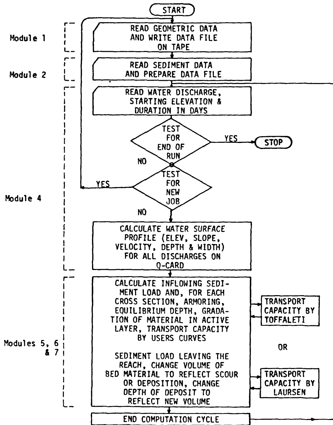
Figure 2 FUNCTIONAL FLOW CHART OF HEC-6
