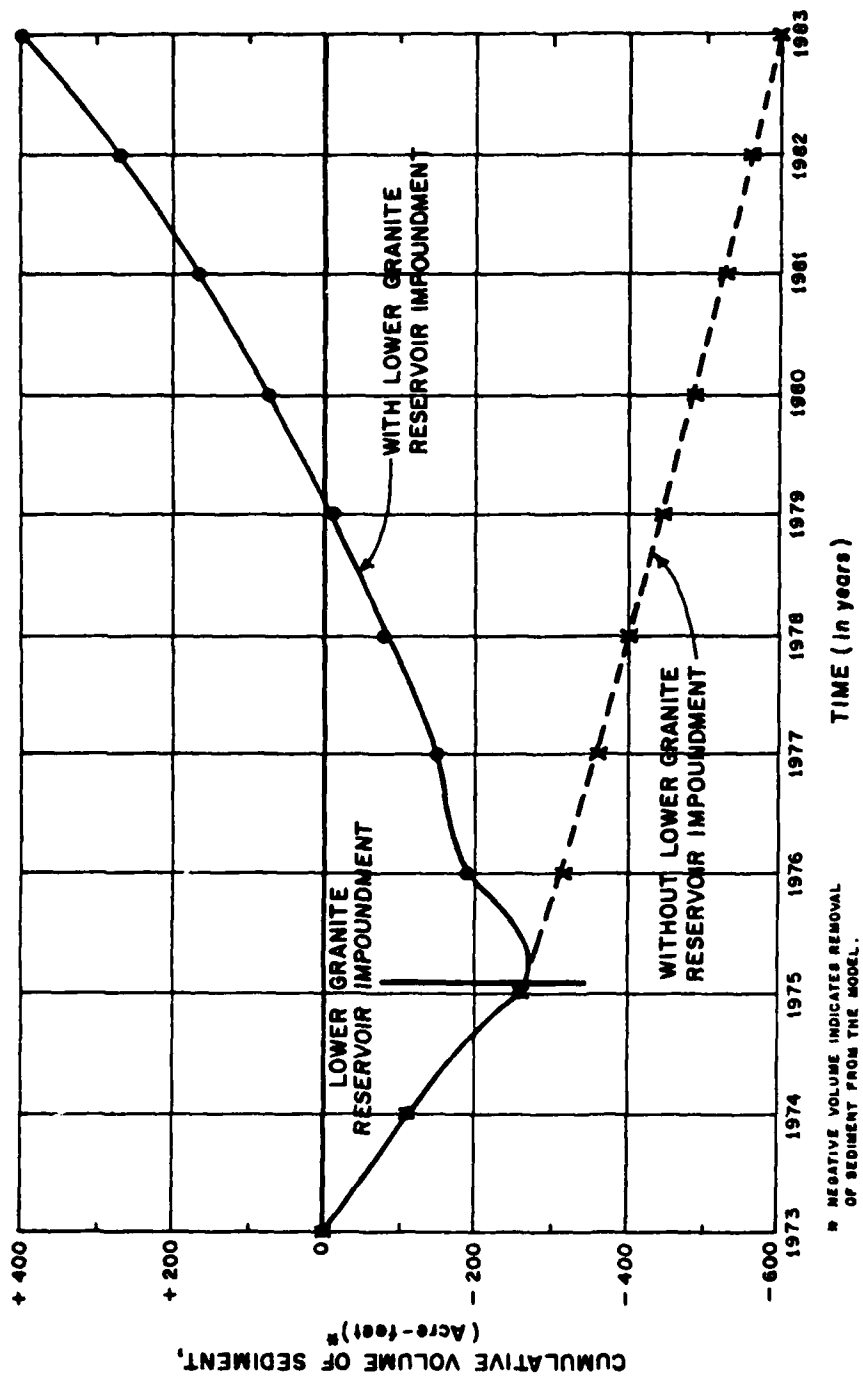
FIGURE 12 CALCULATED VOLUME OF SEDIMENTATION WASHINGTON POWER DAM REMOVED
