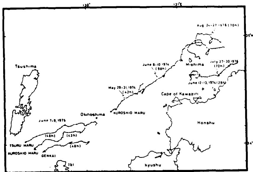
Trajectories of the current drogues in the Tsushima Straits and in the area east of the Straits (summer).
