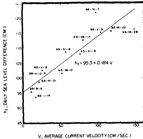
Relation between Izuhara-Pusan daily mean sea-level differences and average current velocities computed by Margules' equation in the western channel.
