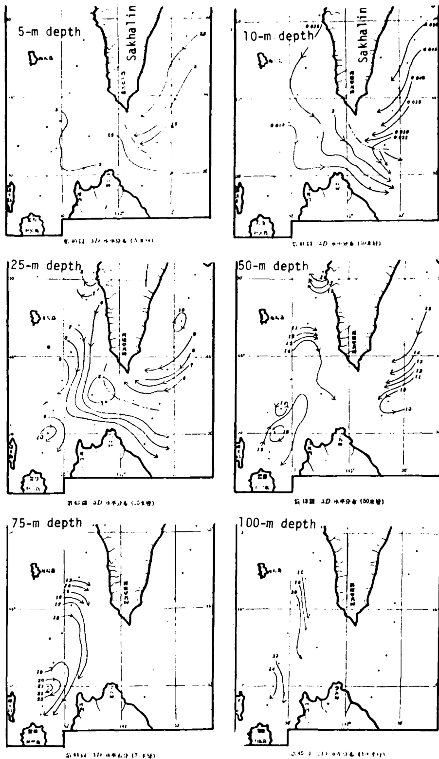
Figure 5. Dynamic topography at Soya Strait, August 1942. (Hakodate Marine Obs., 1944)
