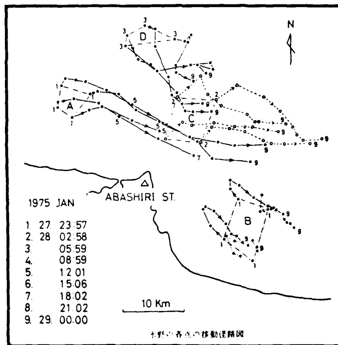
Figure 2. (Kawamura et al, 1975) Trajectories of drift ice.
