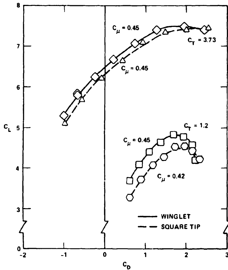
Figure 23b - Drag Polar
