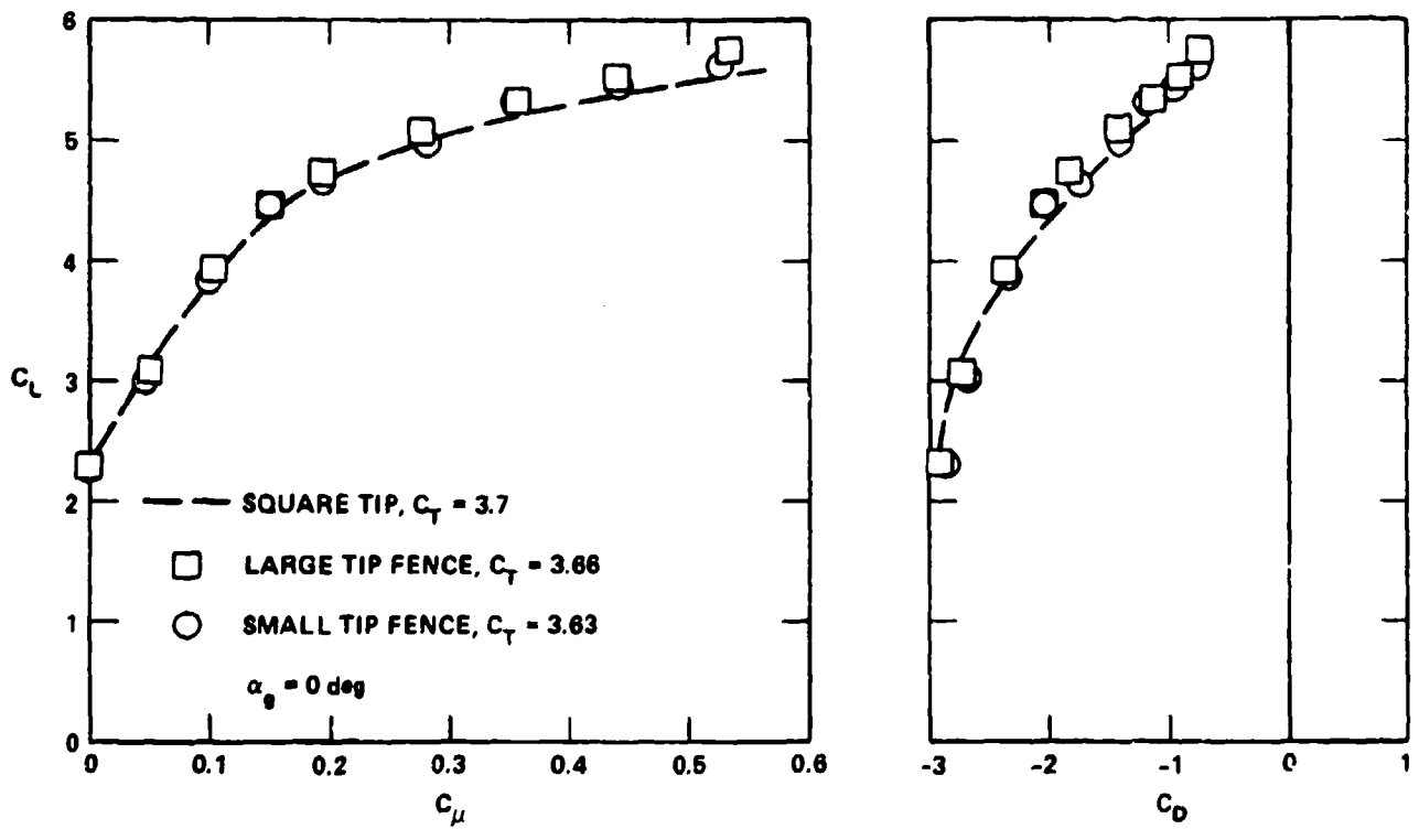
Figure 19a - Effect of Blowing Variation
