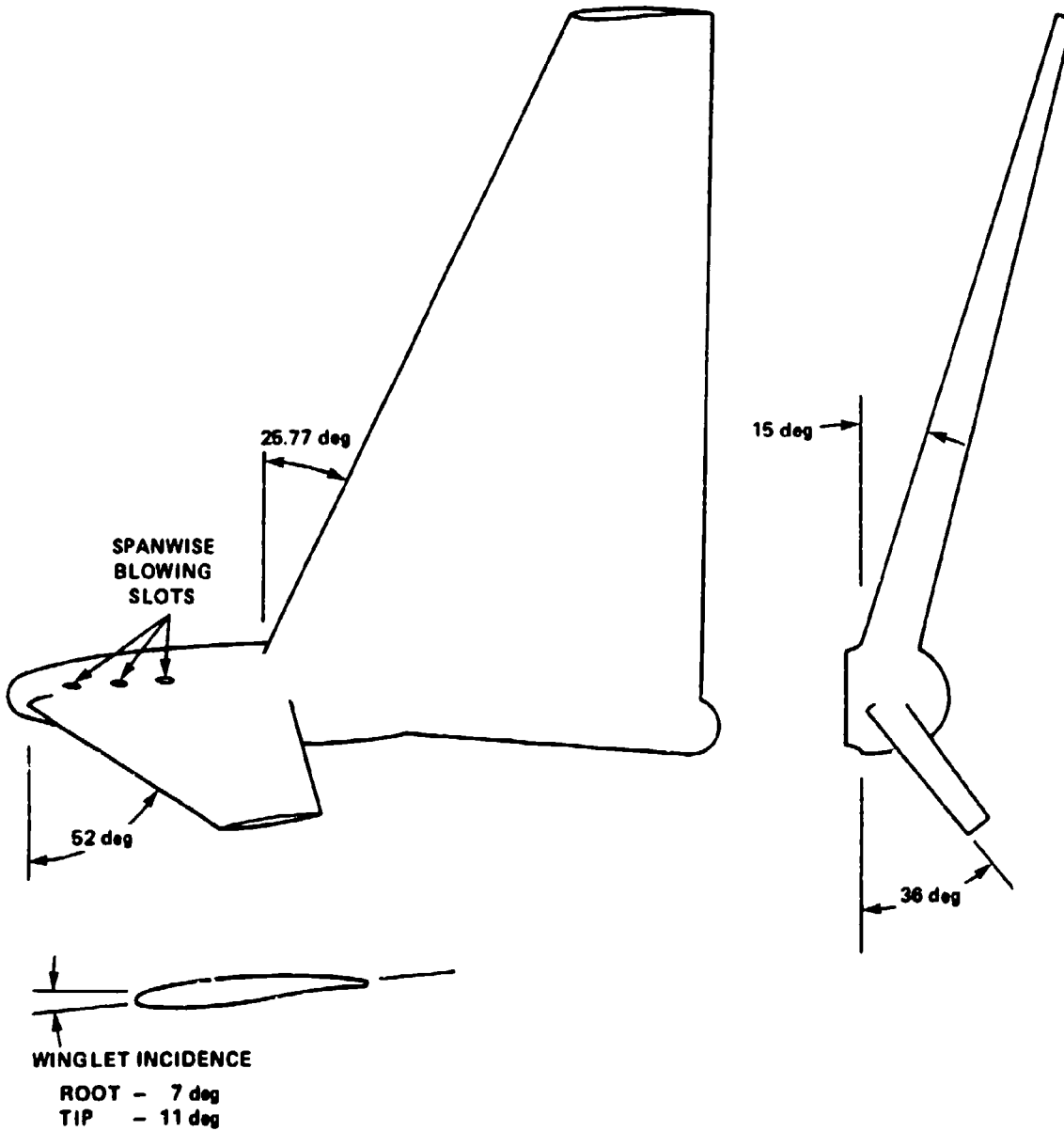
Figure 7a - Winglet with Small Lower Surface and Large Upper Surface
