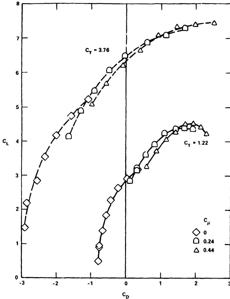
Figure 16b - Drag Polar
