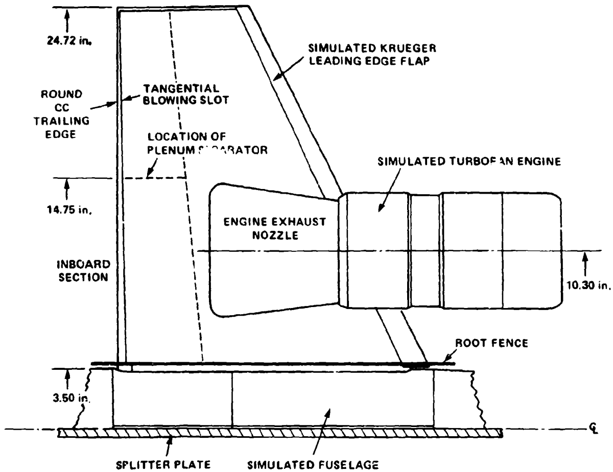
Figure 2 - Aspect Ratio 4 Circulation Control Wing/Upper Surface Blowing Semispan Model Platform
