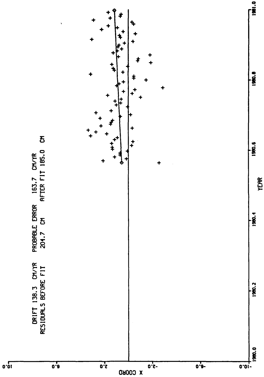
Figure 4a. Difference in X Component of Pole Position, GEOS-3 minus 1967 92A
