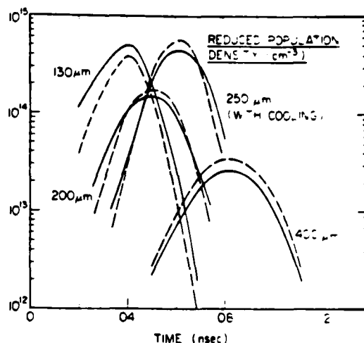
Fig. 6. Numerical code calculation of reduced population densities. Distances are from initial aluminum surface. The pair of curves at 250 \mu corresponds to a calculation with provision to simulate the cooling effect of the magnesium plate. The other three pairs correspond to a simple flat aluminum target.
