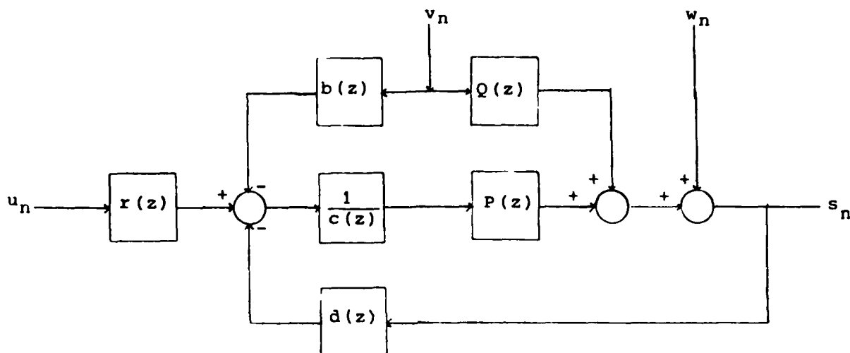
FIGURE 3 - Closed-loop system
