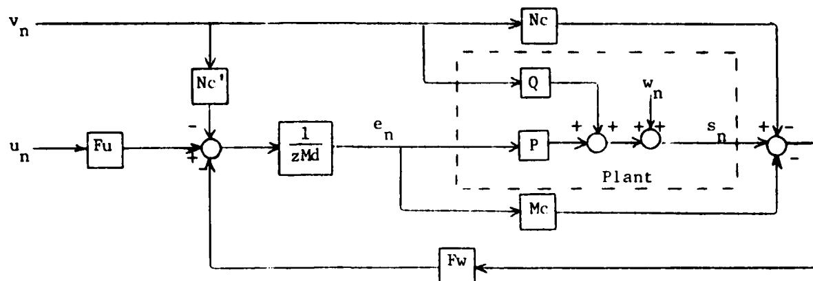
Figure 6. SISO AMAC Representation
