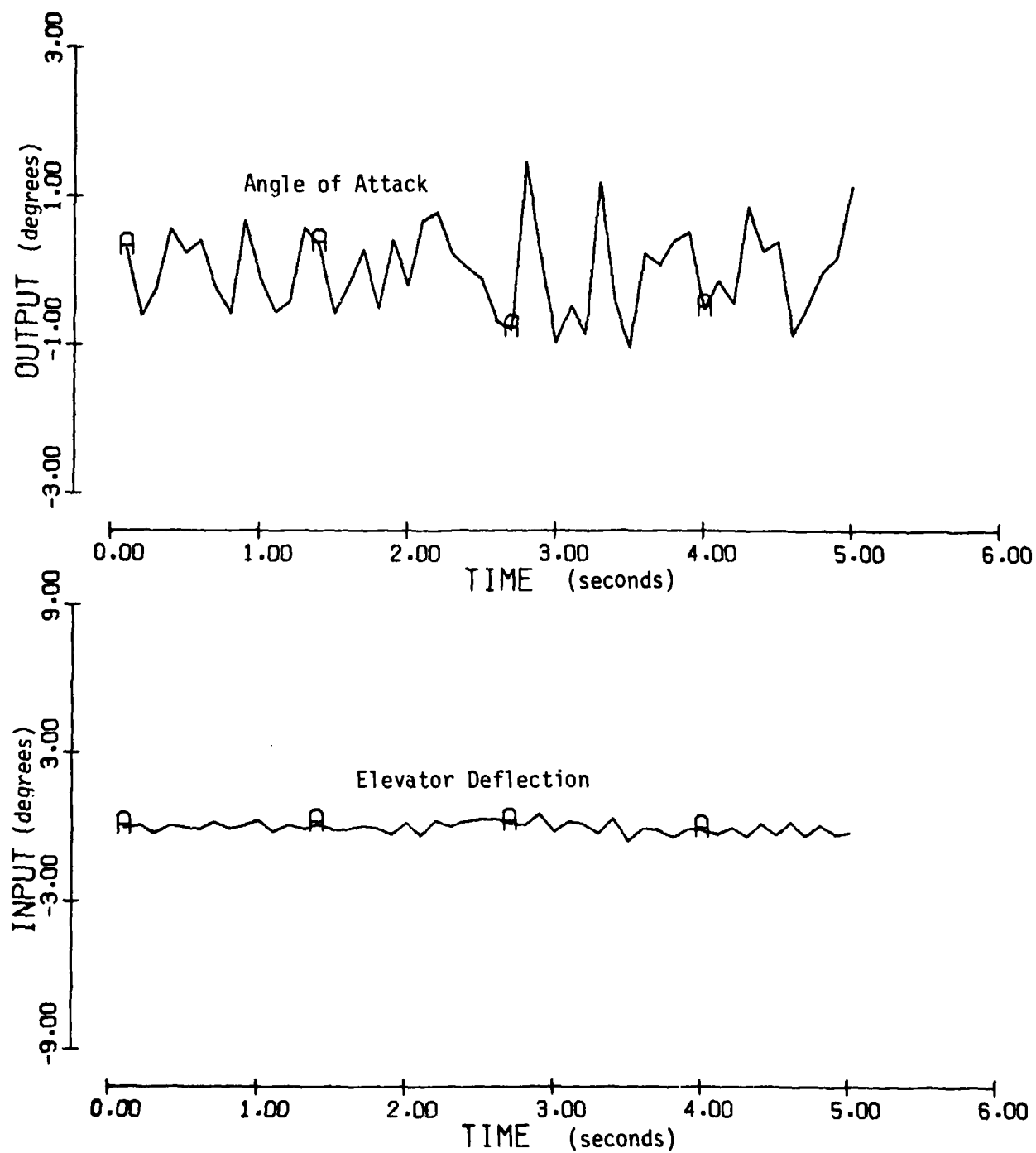
Figure 45a. Gradient algorithm with measurement noise.
