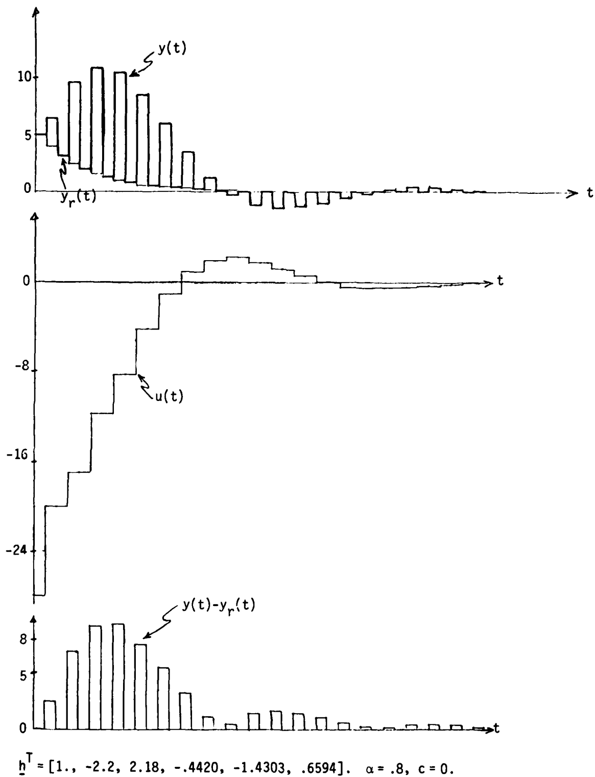
Figure 20. Two-step ahead prediction for the nonminimum phase.
