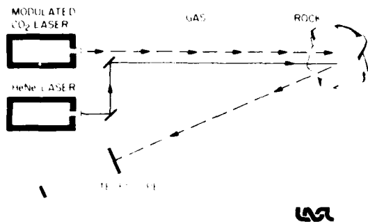
FIGURE 10. The apparatus used for quasi-single ended remote detection by thermal deflection. At the focus of the telescope is the dual photodiode which monitors deflection of the Helium Neon spot on the rock. In lab tests the sensitivity is similar to the apparatus of Figure 6.
