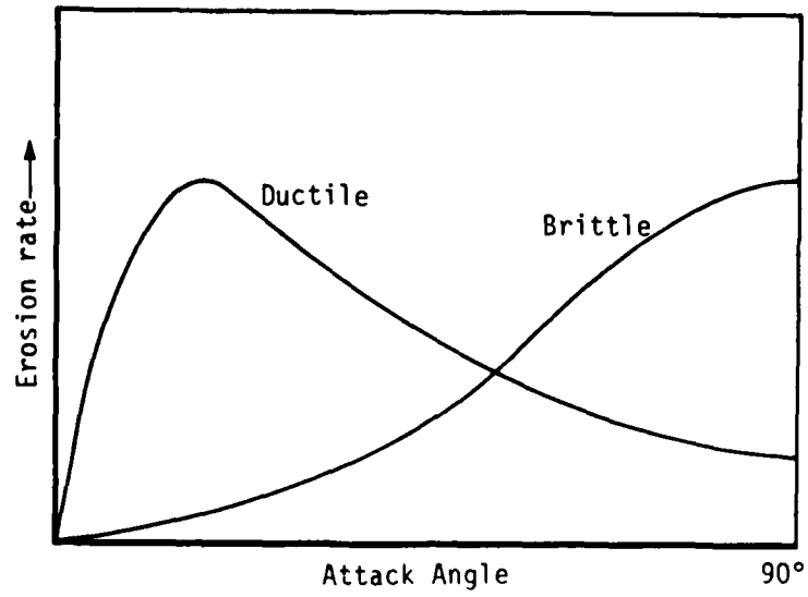
FIGURE 5. Erosion rate changes with varying attack angle.
