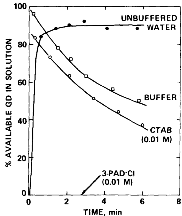
FIGURE 2. Behavior of GD (0.006 M) from the neat agent in aqueous solutions buffered at pH 9.6 (except for unbuffered water).
