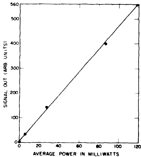
FIGURE 9. A plot of thermal deflection signal strength versus CO 2 laser power incident on the cell.
