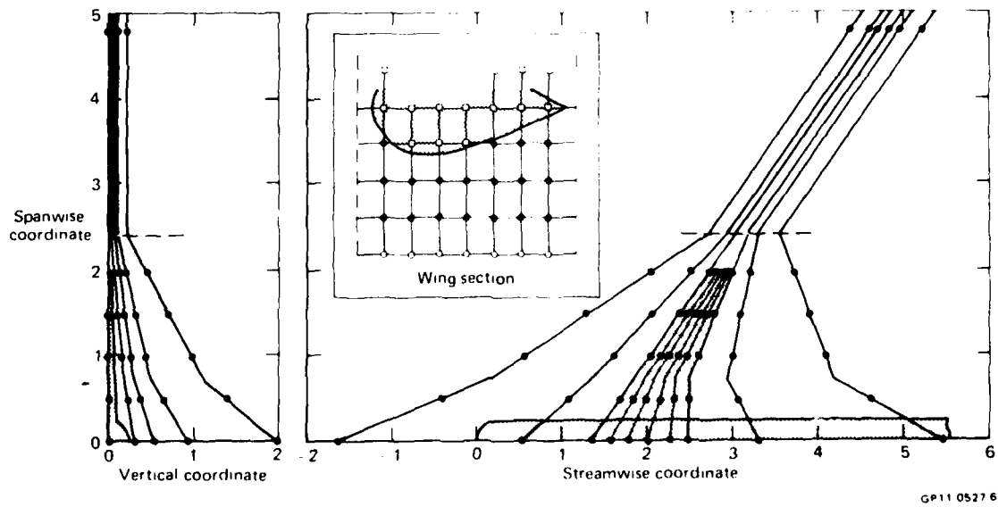
Figure 4. Schematic of a computation grid in the physical domain.
