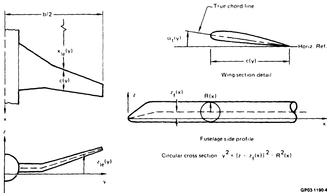
Figure 1. Wing/body geometry.
