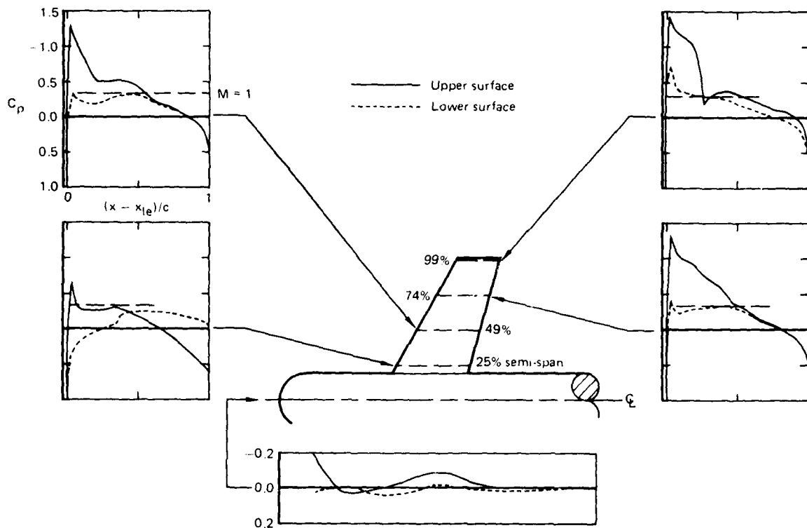
Figure 10. Calculated surface-pressure distributions on a configuration composed of ONERA Wing M6 attached at mid-height to a hemisphere-cylinder fuselage: M_\infty = 0.84 , \alpha = 3.06^\circ . Grid dimension: 49 \times 19 \times 25 . Every third spanwise station is shown.
