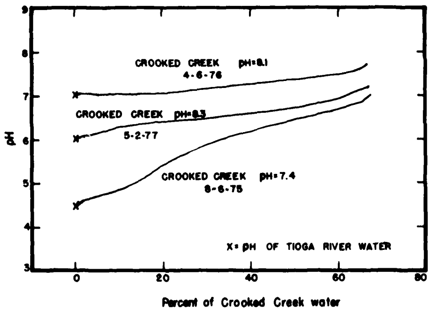
Figure 8.--Titration curve for Tioga River at Tioga with water from Crooked Creek at Tioga.
