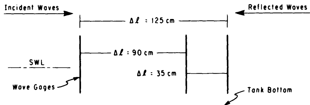
Figure 2. Wave gage array used to measure wave reflection.
