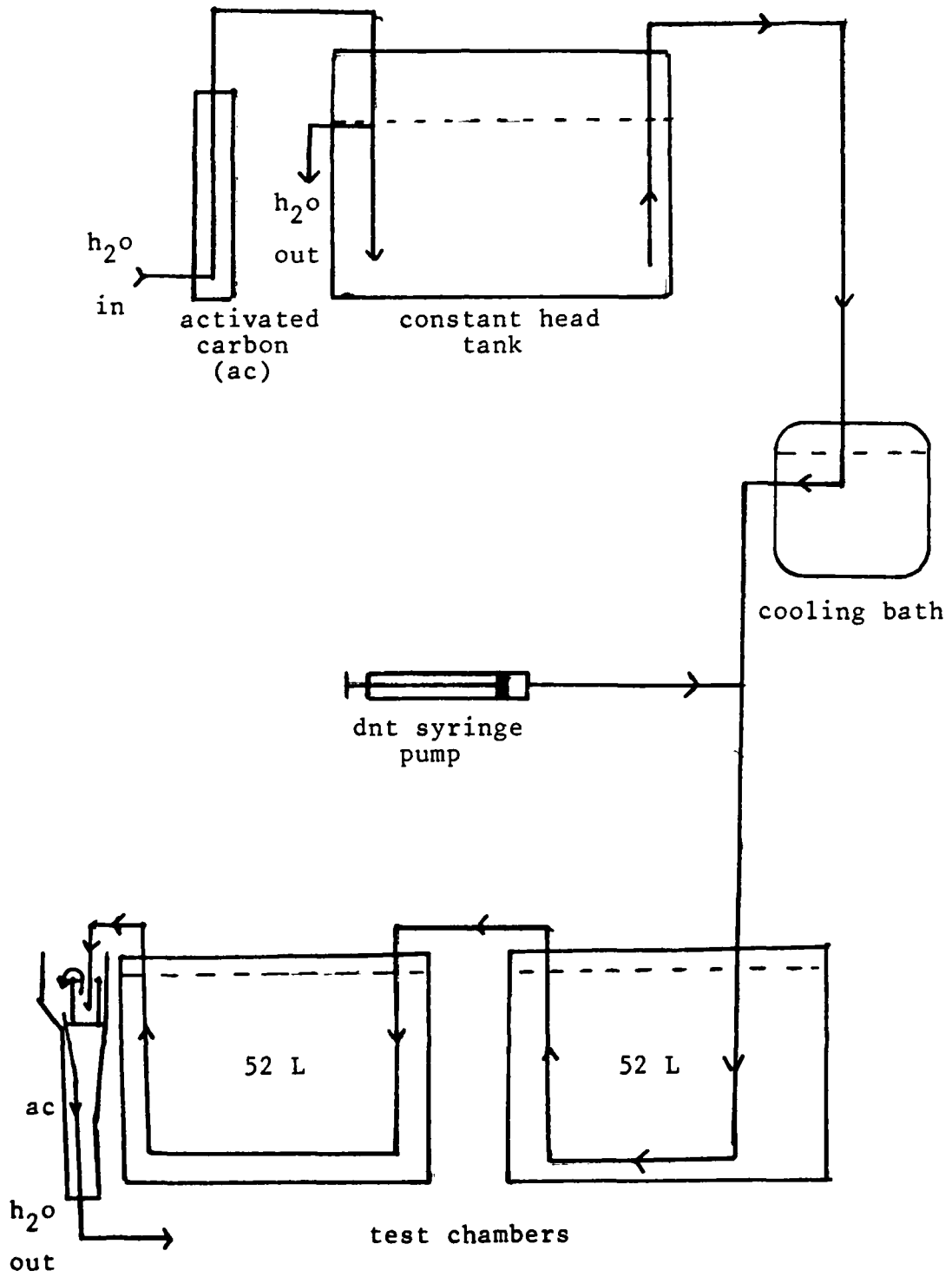
Figure 1. Unit Flow-Through System
