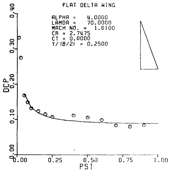
Figure A13. Pressure Distribution on a Flat Delta Wing; M = 1.61 , \alpha = 4.0 .
