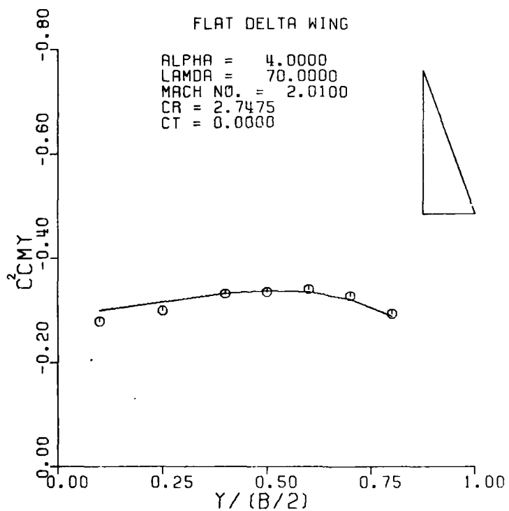
Figure 28. Sectional Normal Force and Pitching Moment for a Flat Delta Wing; M = 2.01 , \alpha = 4.0 .
