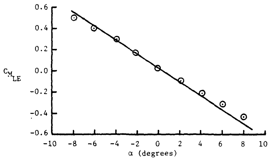
Figure 19. Characteristics of a Finite Wing that is Both Cambered and Twisted.
