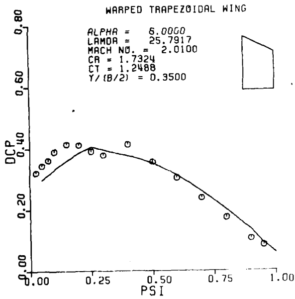
Figure A39. Pressure Distribution on a Warped Trapezoidal Wing; M = 2.01 , \alpha = 6.0 .
