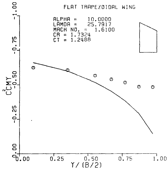
Figure A10. Sectional Normal Force and Pitching Moment for a Flat Trapezoidal Wing; M = 1.61 , \alpha = 10.0 .
