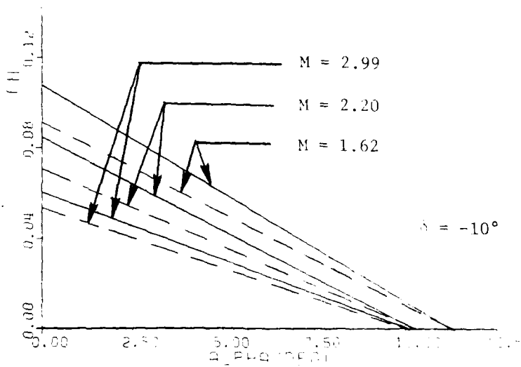
Fig. 43. Theoretical Normal Force and Hinge Moment Coefficients versus Wing Angle of Attack for Gap = 0.0 and 4.0", \delta = -10^\circ .
