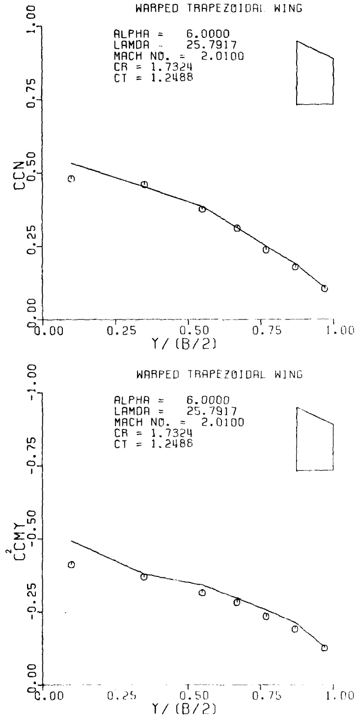
Figure 41. Sectional Normal Force and Pitching Moment for a Warped Trapezoidal Wing; M = 2.01 ; \alpha = 6.0 .
