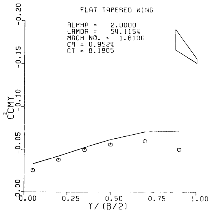
Figure 30. Sectional Normal Force and Pitching Moment for a Flat Tapered Wing; M = 1.61 , \alpha = 2.0 .
