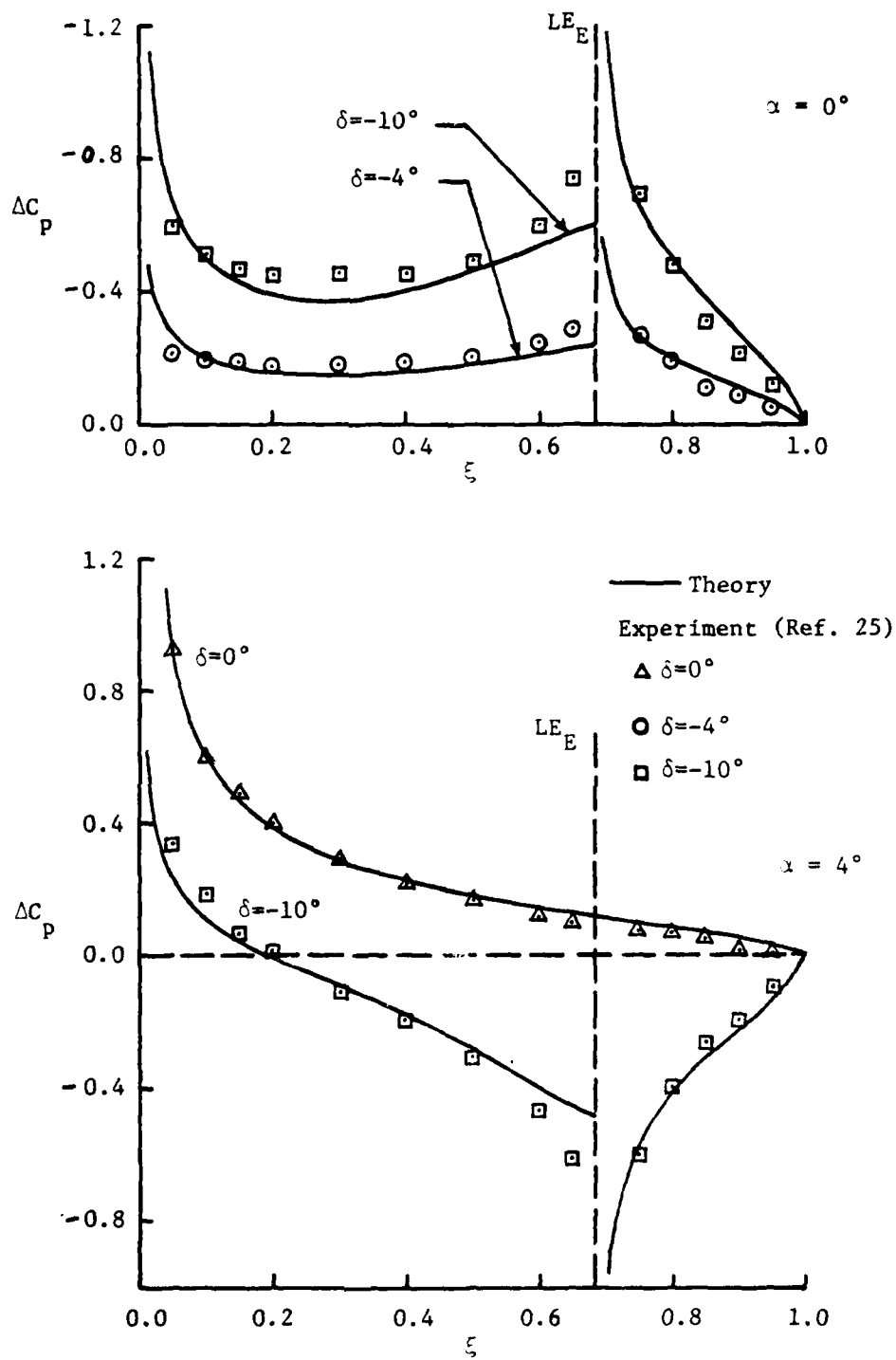
Figure 9. Chordwise Loading with a Deflected Elevon at \eta = 0.5 .
