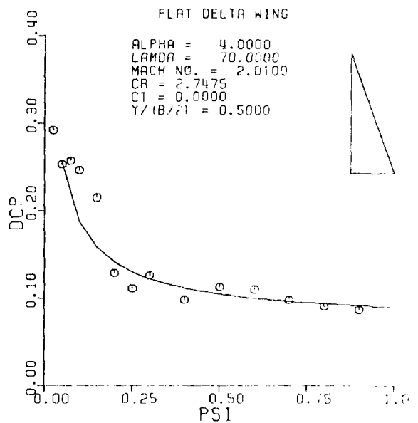
Figure 27. Pressure Distribution on a Flat Delta Wing; M = 2.01 , \alpha = 4.0 .
