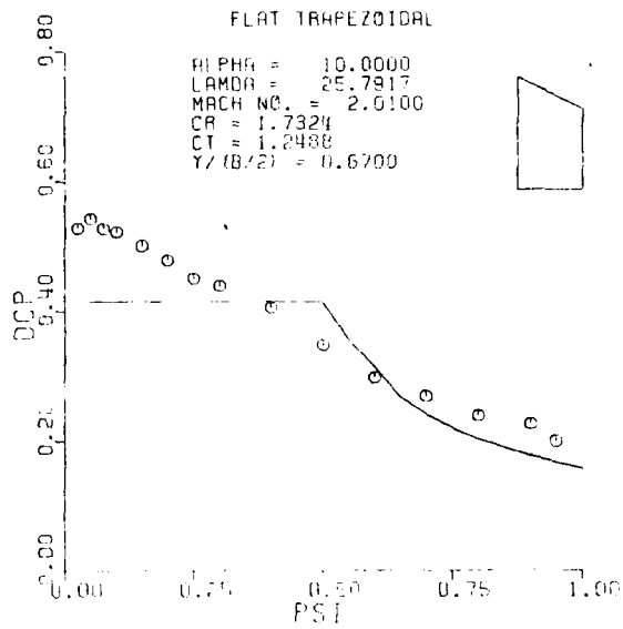
Figure A11. Pressure Distribution on a Flat Trapezoidal Wing; M = 2.01 , \alpha = 10.0 .
