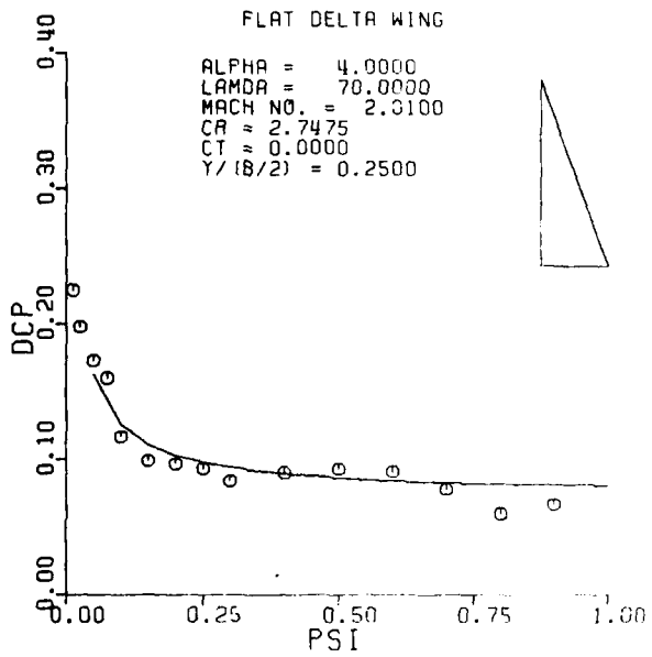
Figure A15. Pressure Distribution on a Flat Delta Wing; M = 2.01 , \alpha = 4.0 .
