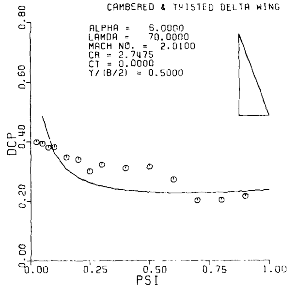
Figure A35. Pressure Distribution on a Cambered and Twisted Delta Wing; M = 2.01, \alpha = 6.0 .
