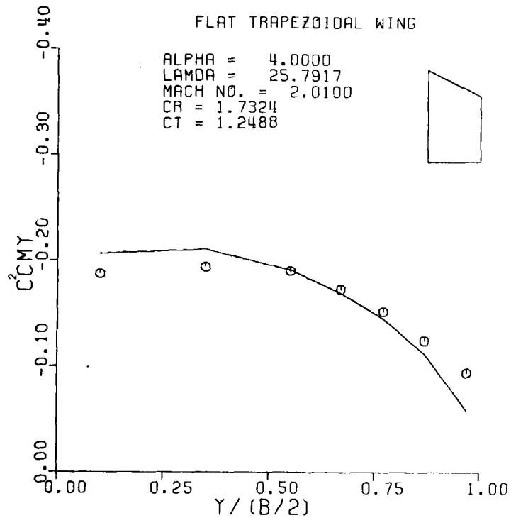
Figure 26. Sectional Normal Force and Pitching Moment for a Flat Trapezoidal Wing; M = 2.01 , \alpha = 4.0 .
