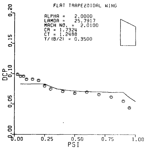
Figure A3. Pressure Distribution on a Flat Trapezoidal Wing; M = 2.01 , \alpha = 2.0 .
