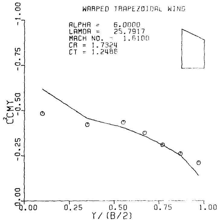
Figure A38. Sectional Normal Force and Pitching Moment for a Warped Trapezoidal Wing; M = 1.61 , \alpha = 6.0 .
