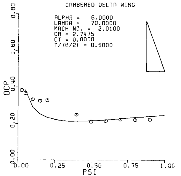
Figure A31. Pressure Distribution on a Cambered Delta Wing; M = 2.01 , \alpha = 6.0 .
