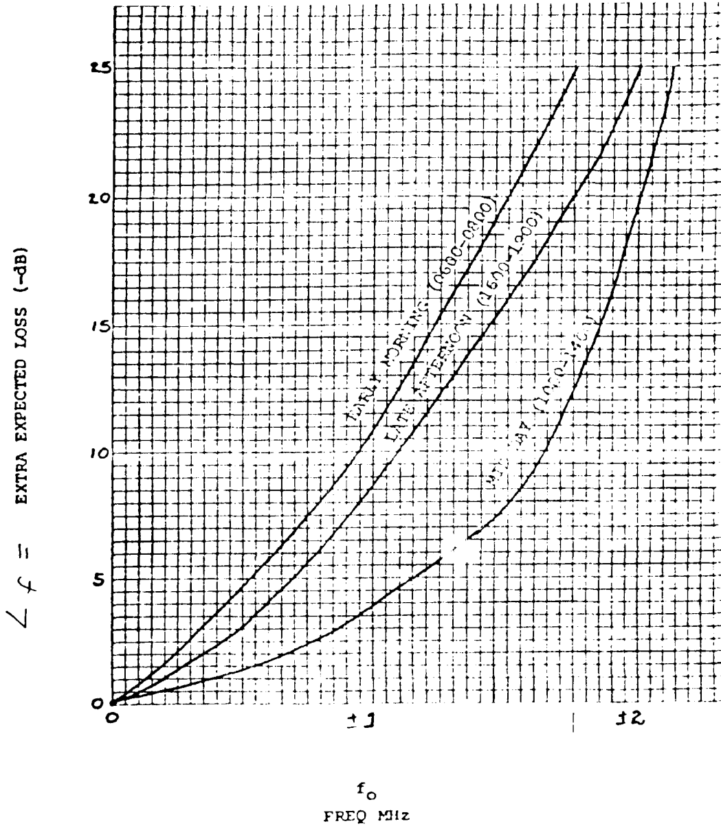
FIGURE 4-16. LOSS DUE TO NOT OPERATING EXACTLY AT f_0
