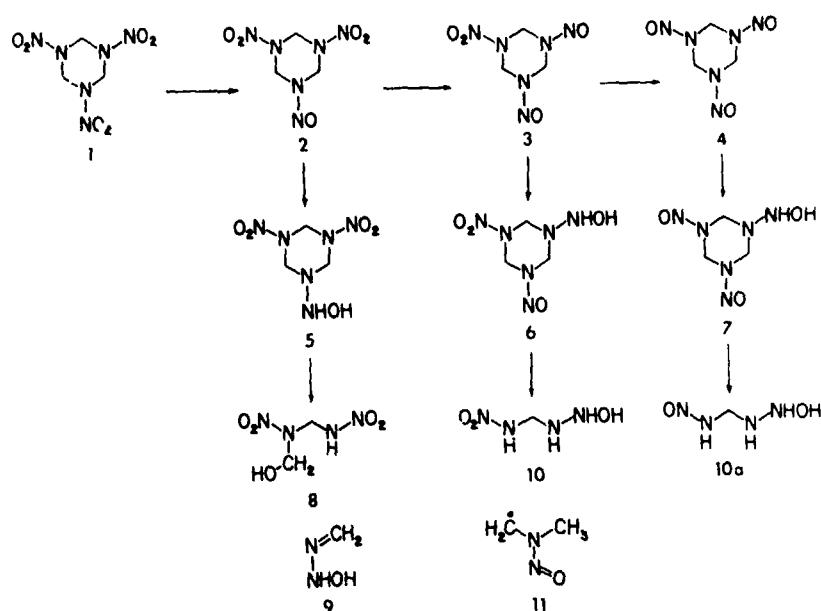
Figure 6. Proposed RDX biodegradation pathway. 1, RDX; 2, MNX; 3, DNX; 4, TNX; 5, 1-hydroxyl-amino-3,4-dinitro-1,3,5-triazine; 6, 1-hydroxyl-amino-3-nitroso-5-nitro-1,3,5-triazine; 7, 1-hydroxylamino-3,5-dinitroso-1,3,5-triazine; 8, N-hydroxymethylmethylenedinitramine; 9, N-hydroxymethylmethylenedinitramine radical; 10, N-hydroxyl-amino-N'-nitro-methylenediamine; 11, dimethyl-nitrosamine radical.
