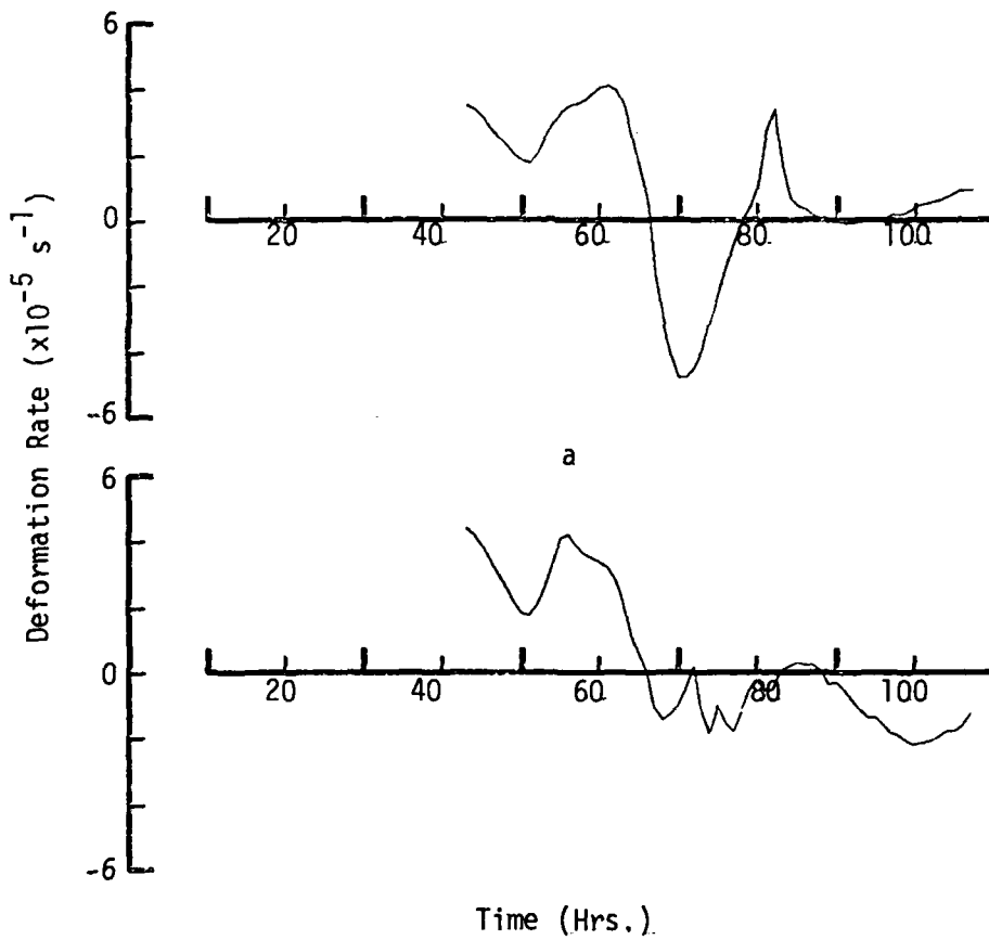
Fig. 2 Normal deformation rates for the large-scale cluster (without corrections for position errors). a is for a geographic coordinate system, and b is for a natural coordinate system.
