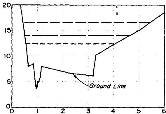
CROSS SECTION NO. 4 MILE 1.86
