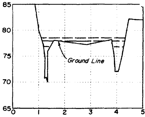
CROSS SECTION NO. 14 MILE 5.37
