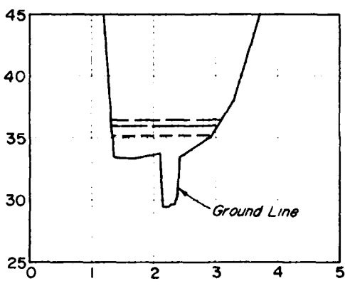
CROSS SECTION NO. 7 MILE 2.85
