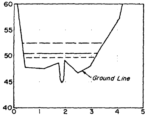
CROSS SECTION NO. 11 MILE 5.30
