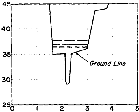
CROSS SECTION NO. 9 MILE 4.22
