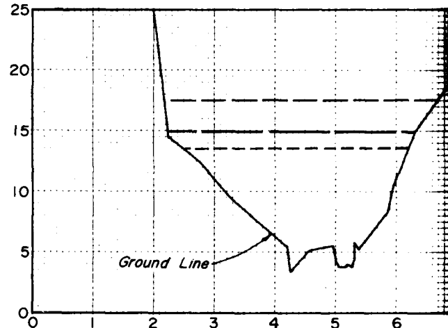
CROSS SECTION NO. 15 MILE 10.47
