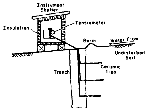
Figure 7. Field installation using flexible tube tensiometers.
