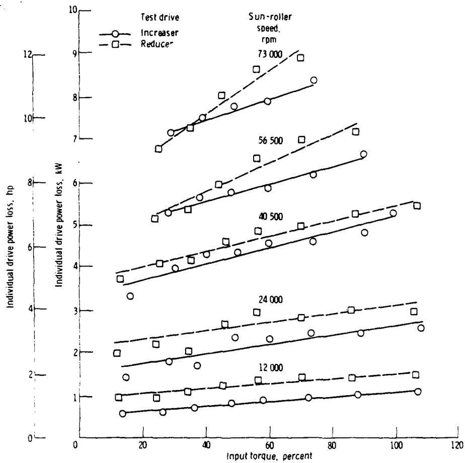
Figure 3. - Test-drive power loss as function of input torque for five input speeds. Design traction coefficient, 0.048; 100-percent input torque: 258 N-m (2520 in-lb) for incraser, 19 N-m (168 in-lb) for reducer.
