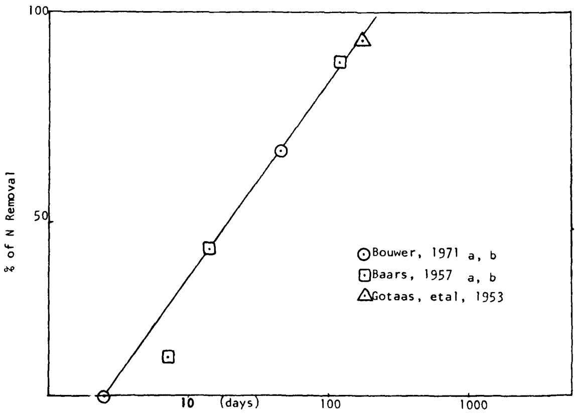
EFFECT OF LENGTH OF INUNDATION PERIOD ON DENITRIFICATION AND N REMOVAL IN RAPID INFILTRATION PONDS Figure IX-3
