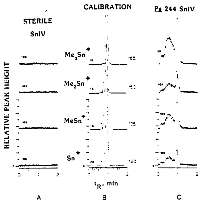
Fig. 1. Selected ion chromatograms obtained with GC-MS data system for (A) Headspace above sterile Nelson's agar slant media containing inorganic SnIV; (B) Calibration mixture of Me_2SnH_2 , Me_3SnH , and Me_4Sn ; (C) Respirant atmosphere above Ps. 244 inoculated Nelson's media containing with inorganic SnIV.
