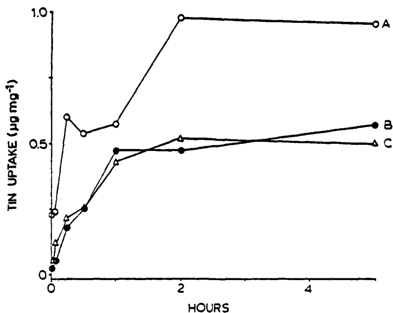
Fig. 3. Accumulation of tributyltin by Ps. 244. At time zero, tin (as \text{Bu}_3\text{SnCl} ) was added (10 mg/L final conc.) to flasks containing 50 mL 5 mM PIPES buffer (pH 7.4) plus (A) Boiled cells (10 min), (B) Starved cells (10 hr, 22 °C in 5 mM PIPES buffer), (C) Starved cells plus glucose (10 mM final conc.)
