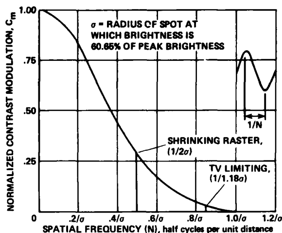
Fig. 33 Relative modulation transfer function
