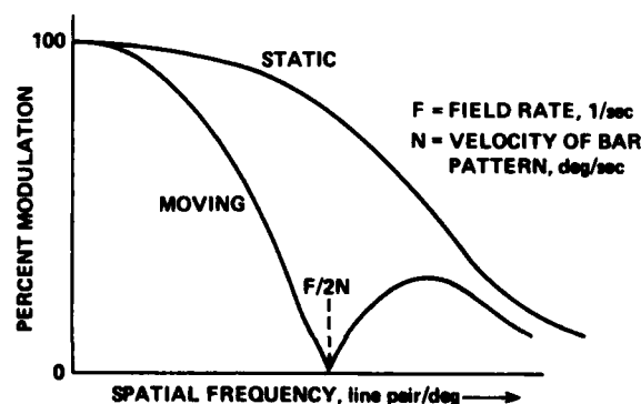
Fig. 37 MTF curve for a moving bar pattern on a television display
