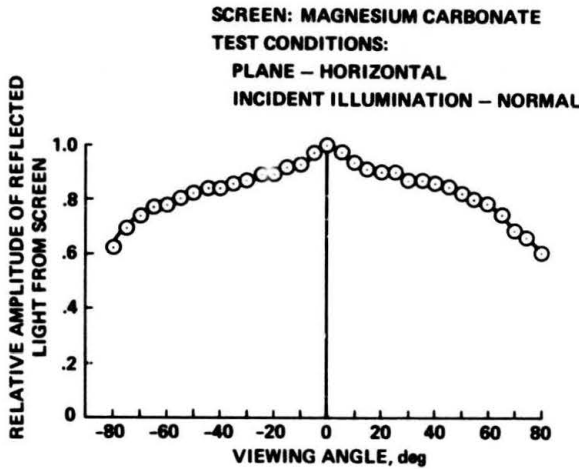
Fig. 48 Test data, magnesium carbonate screen
