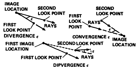
Fig. 6 Collimating descriptors
