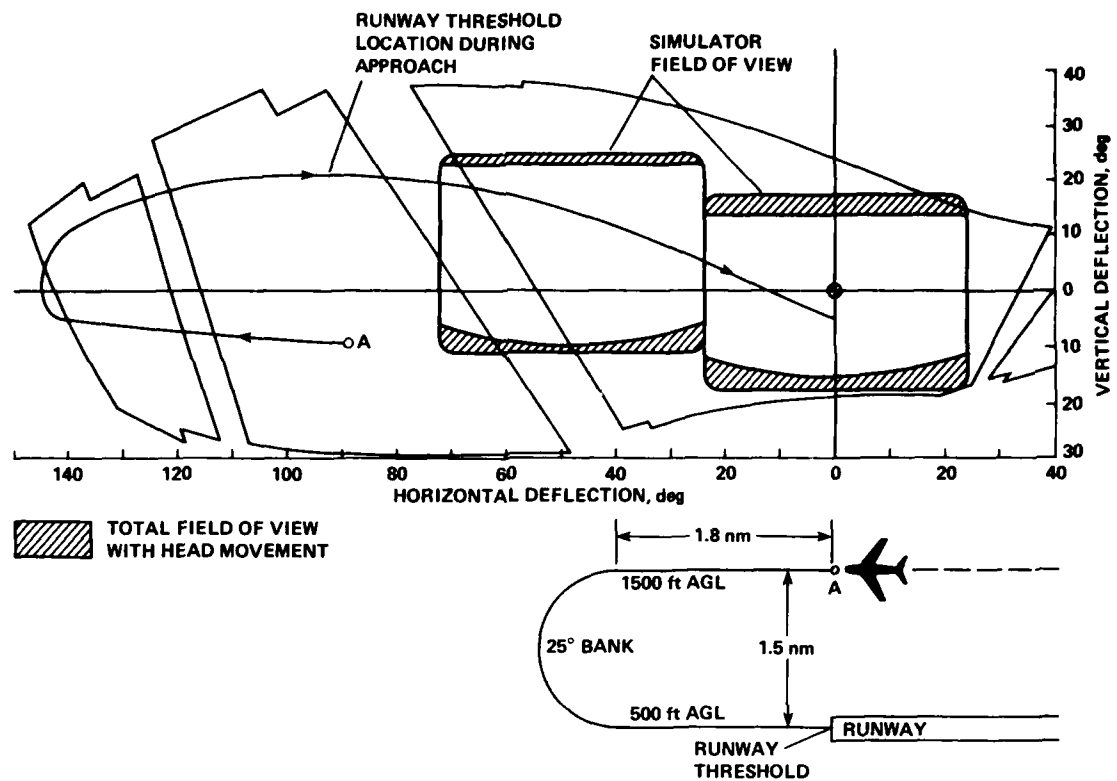
Fig. 72 Captain's vision envelope: 747
