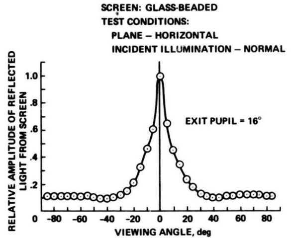
Fig. 49 Test data, glass-beaded screen
