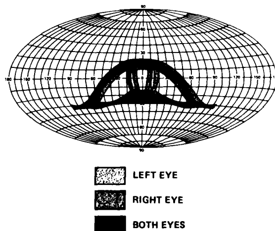
Fig. 66 Military strike aircraft (Panavia Tornado) binocular vision plot
