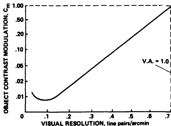
Fig. 26 Object contrast modulation, \Delta B/2B_{av} , necessary for eye to resolve a pattern of alternating dark and bright bars of equal width ( B_{av} = 35 \text{ cd/m}^2 )
