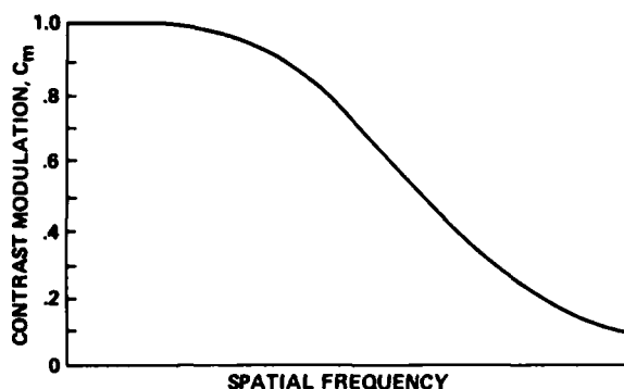
Fig. 32 Typical MTF curve
