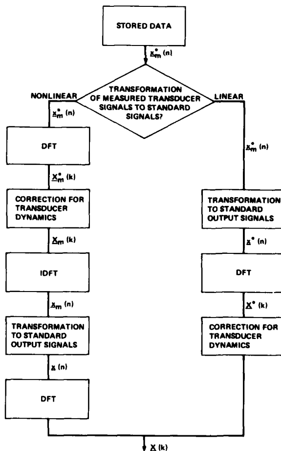
Fig. 76 Computation of discrete Fourier transform of the standard signals
