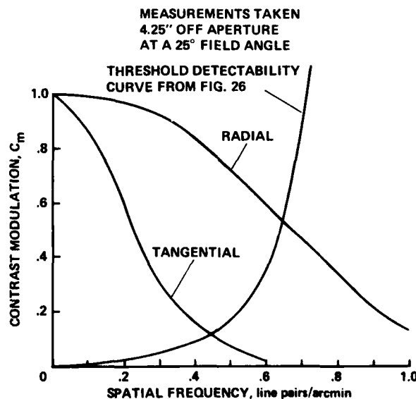
Fig. 35 Contrast modulation curve for a wide-field pupil-forming display
