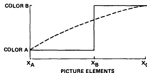
Fig. 58 Smooth shading technique
