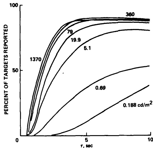
Fig. 14 Average target acquisition curves for 10 subjects for 100% contrast at the luminance shown
