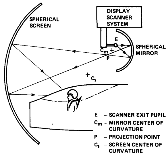
Fig. 63 Visual simulation display utilizing scanned laser projector
