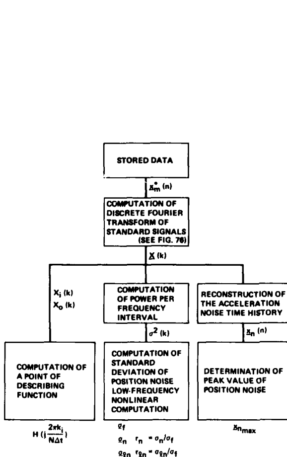
Fig. 75 Data analysis
