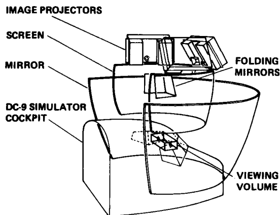
Fig. 5 Multiviewer display showing viewing volume (adapted from Ref. 2)
