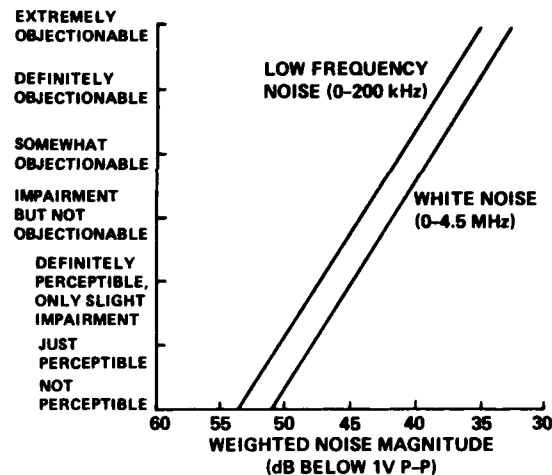
Fig. 44 The aesthetic opinion ratings of broadcast signals impaired by video (base band) weighted values
