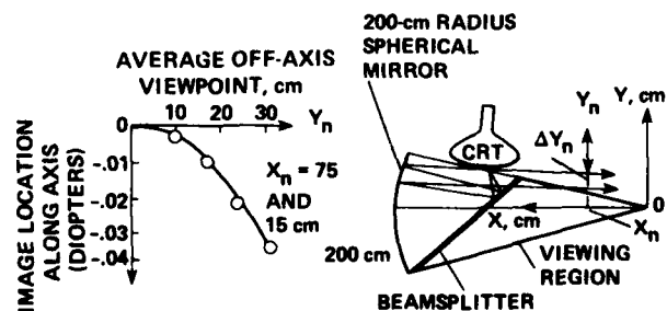
Fig. 8 Off-axis collimating performance of a spherical mirror/beam-splitter collimator (sampled points are 70 mm apart, \Delta Y_n = 70 mm)
