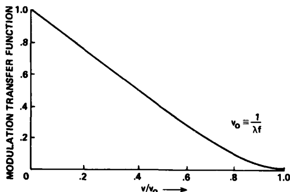
Fig. 34 The maximum modulation transfer function of a diffraction-limited system. Note that the curve is based on diffraction effects for a circular aperture and that the abscissa is the ratio of the frequency to the limiting frequency, v_0 .
