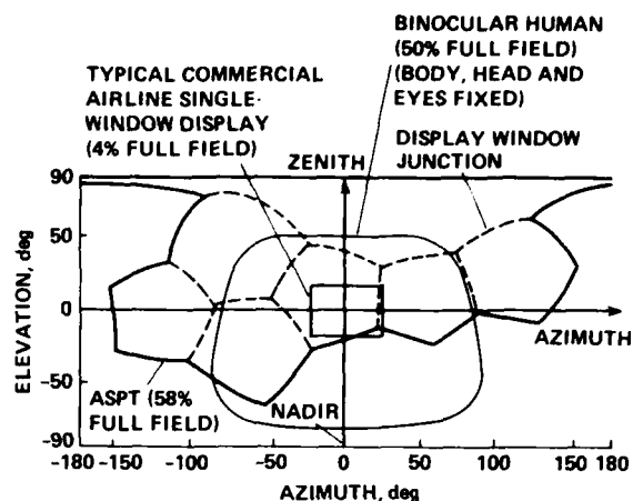
Fig. 2 Typical field plots
