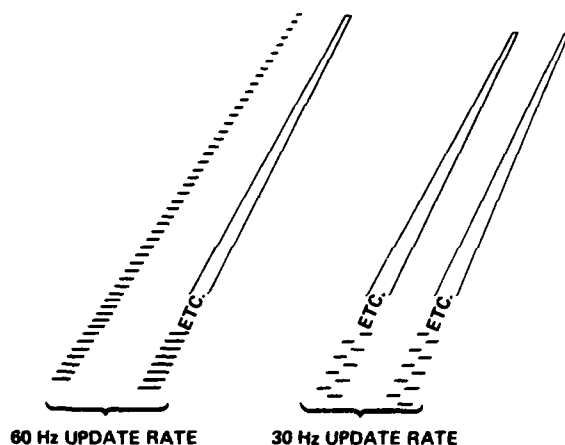
Fig. 54 Effect of high turning rates and two update rates on the appearance of high-contrast runway edge and center lines
