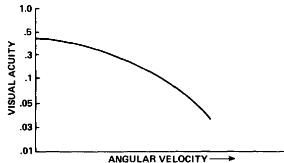
Fig. 38 Typical resolution curve using V.A. as a metric
