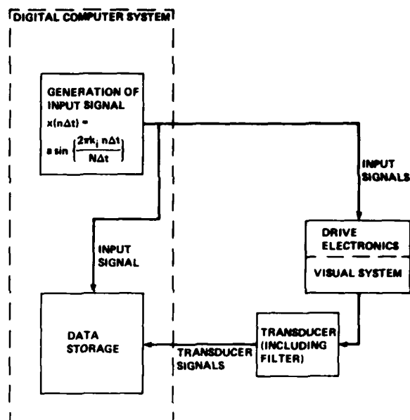
Fig. 74 Signal generation and data logging
