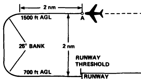
Fig. 71 Captain's vision envelope: A300
