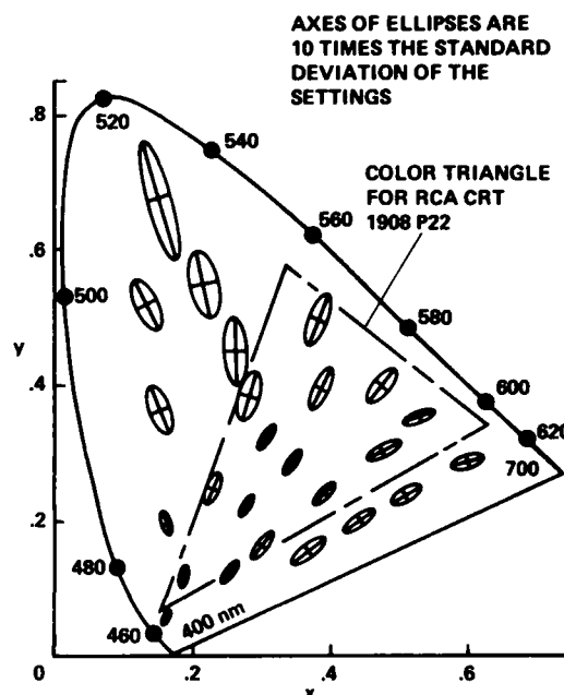
Fig. 43 Chromaticity matching under ideal conditions. The MacAdam ellipses illustrate the adjustment precision possible when chromaticity matches are made by a single observer under ideal conditions.
