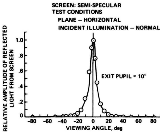
Fig. 50 Test data, semi-specular screen
