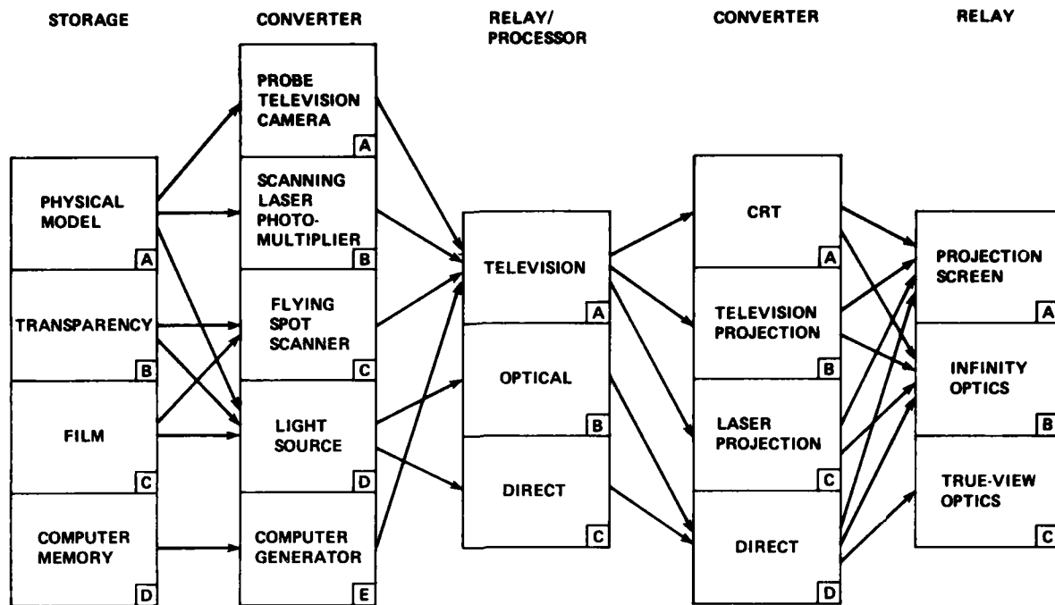
Fig. 47 Typical visual system components and some of the various combinations
