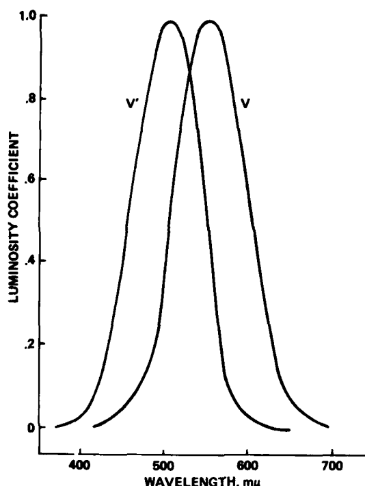
Fig. 13 The scotopic (V') and photopic (V) curves of relative spectral luminosity
