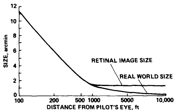
Fig. 15 Representation of light sizes in night scene
