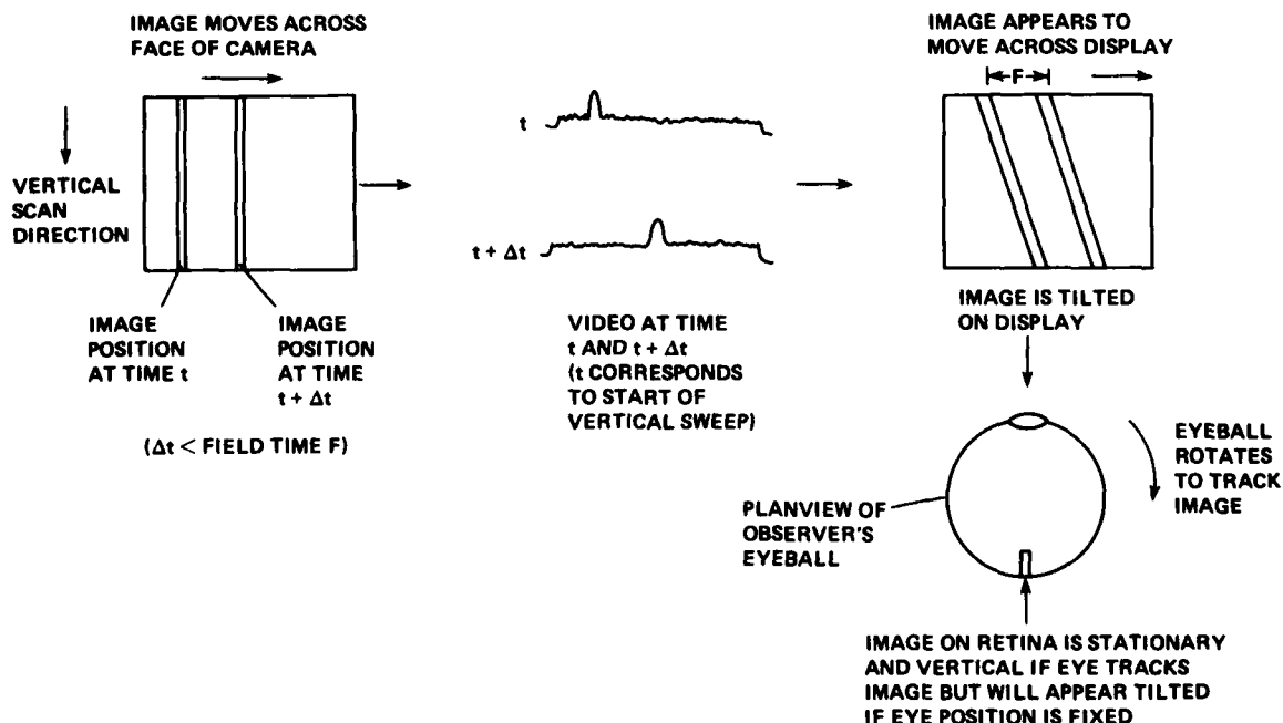
Fig. 55 Illustration of tilted image phenomena
