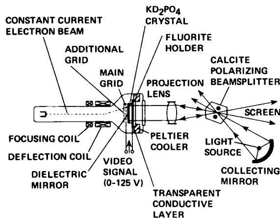
Fig. 62 Principle of operation, Titus tube-light valve projector
