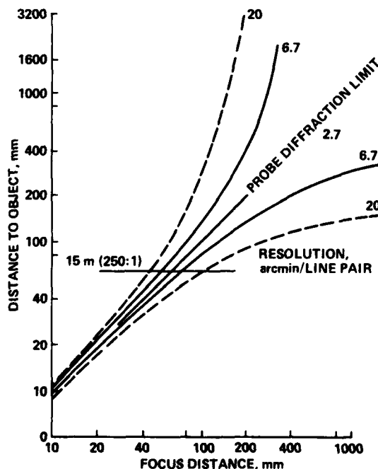
Fig. 7 Probe depth of field vs focus distance
