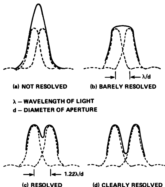
Fig. 31 Resolving power. (The dashed lines represent the diffraction patterns of two point images at various separations. The solid line indicates the combined diffraction pattern.)
