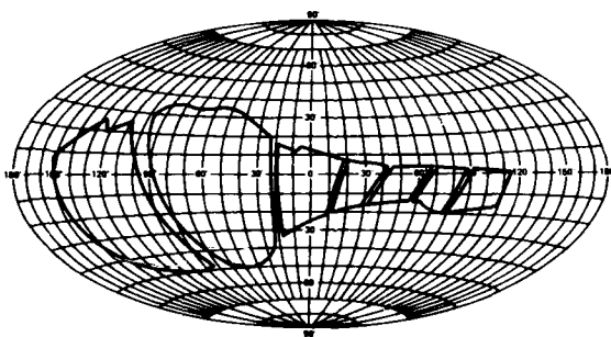
Fig. 69 Small jet transport (Falcon 20C)
