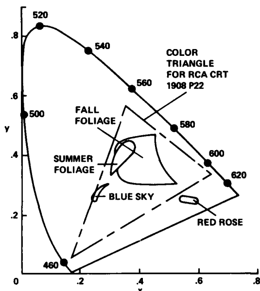
Fig. 42 Chromaticity of common materials
