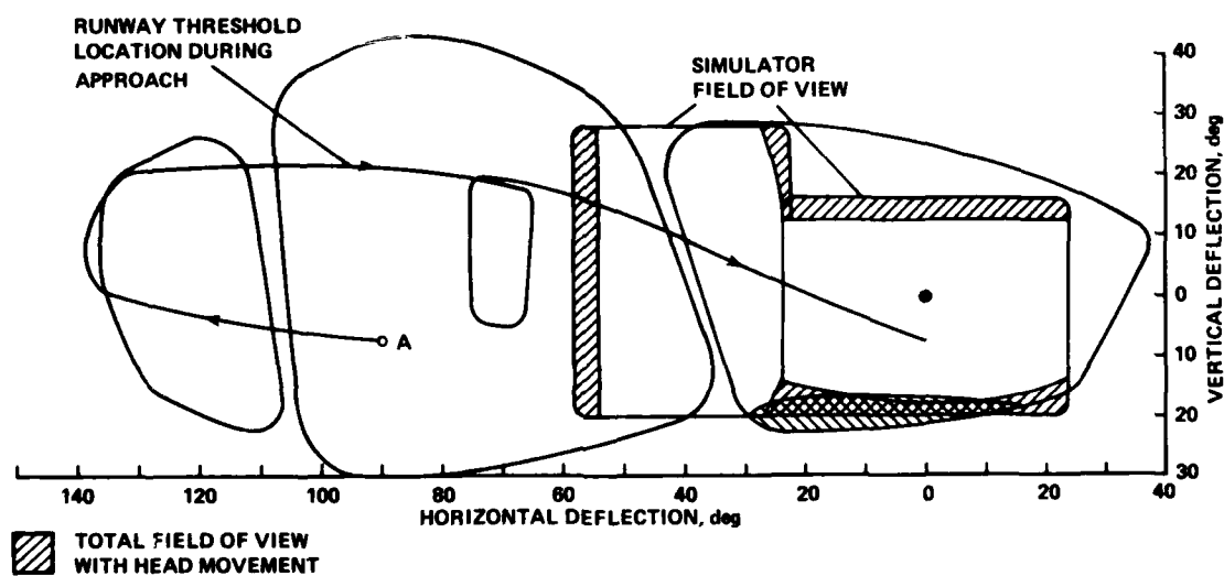
Fig. 69 Small jet transport (Falcon 20C)
