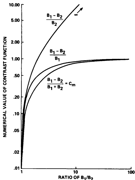
Fig. 16 Differences among commonly used contrast functions; B_1 = target luminance, B_2 = background luminance
