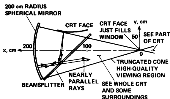
Fig. 4 Spherical mirror beam-splitter viewing region.
