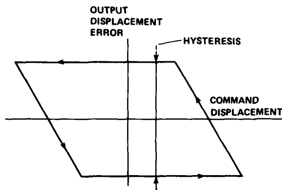
Fig. 52 Hysteresis plot
