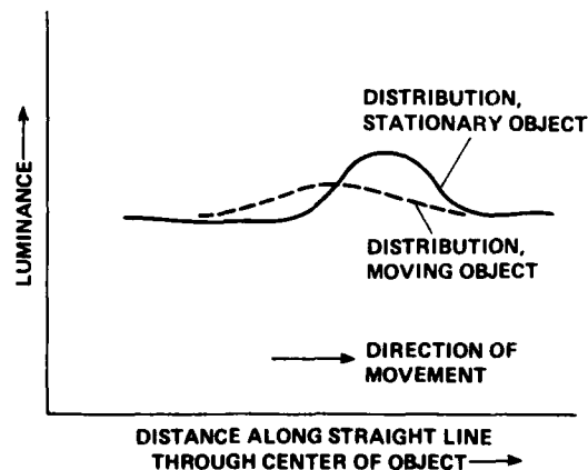
Fig. 20 Luminance distribution of moving object
