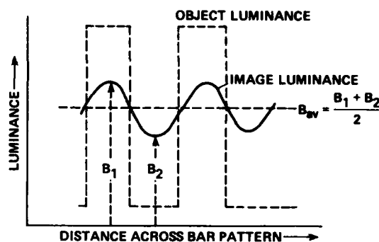
Fig. 17 Displayed modulation of typical bar pattern
