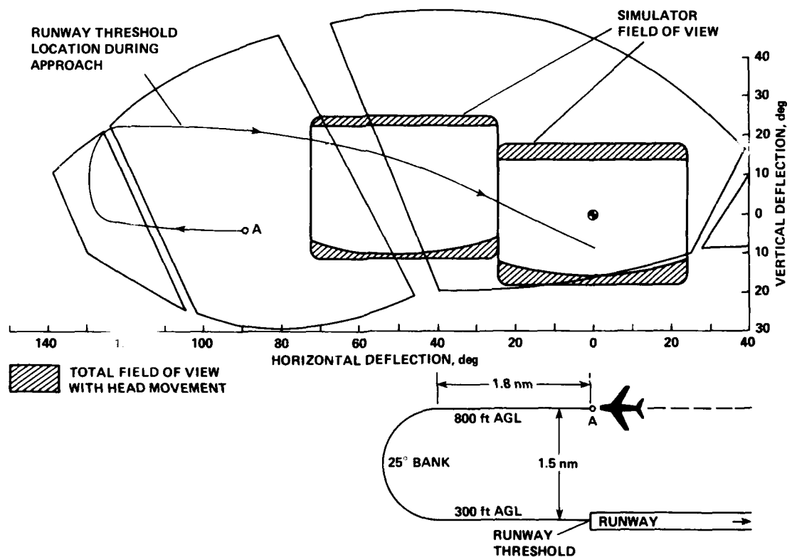
Fig. 73 Captain's vision envelope: DC-10
