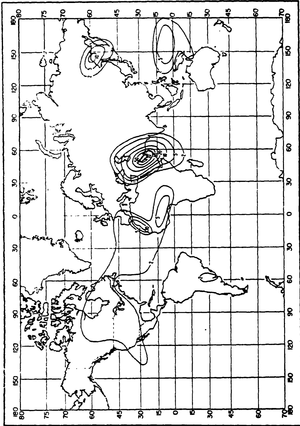
Figure II-18. Percent of Time Trapping Frequency is Less Than 300 MHz, August
