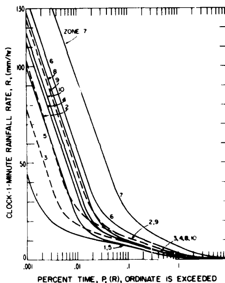
Figure 2. Estimated distribution of rainfall rates for one-minute periods, P_1(R) , for the European rainfall climatic zones.
