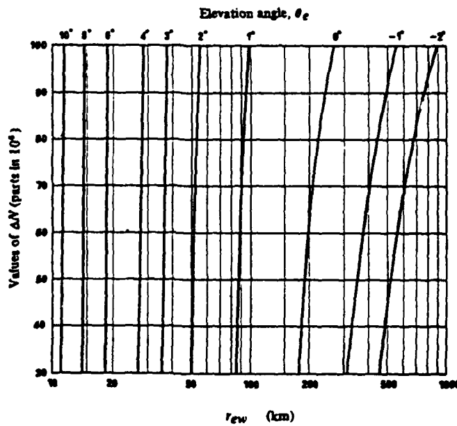
Figure II-49. Effective Path Distance (km) for Water Vapor Absorption
