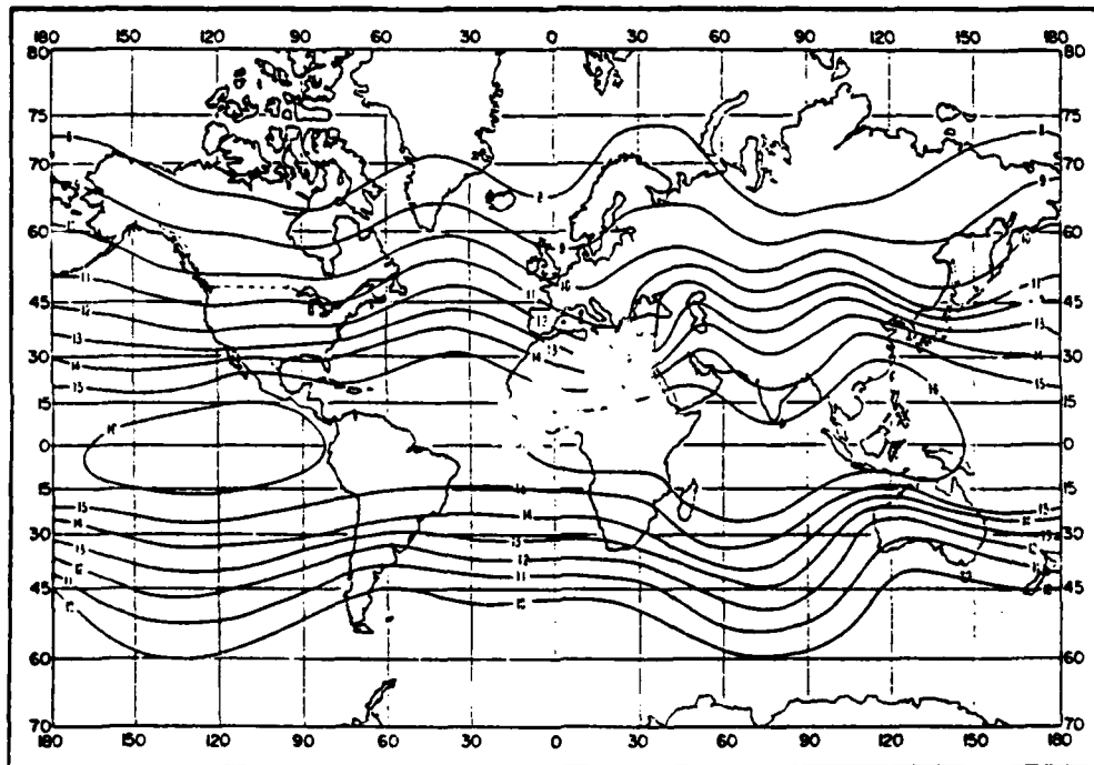
Figure II-3. Mean Altitude (km) of the Topopause, May
