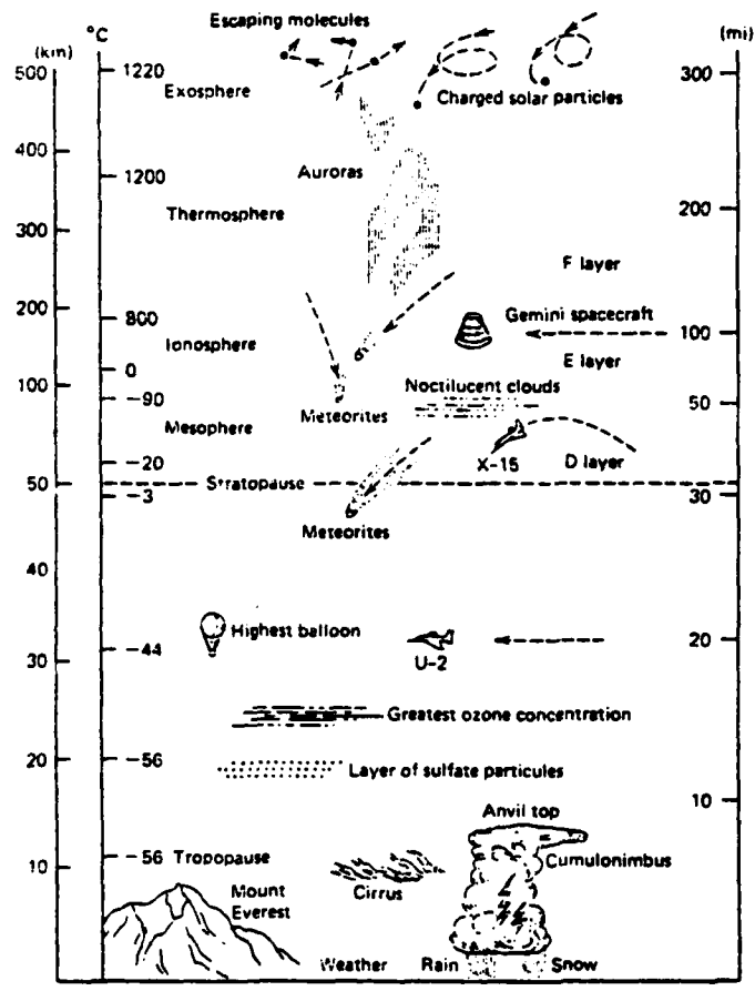
Figure II-1. Stratification of the Earth's Atmosphere
