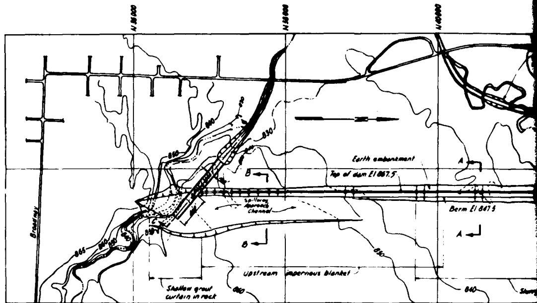
PLAN Scale 0 400 800 feet
