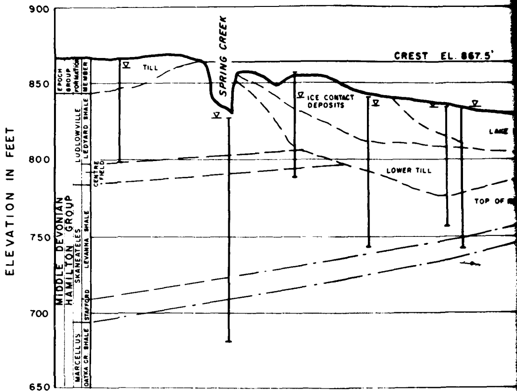
PROFILE ALONG AXIS
