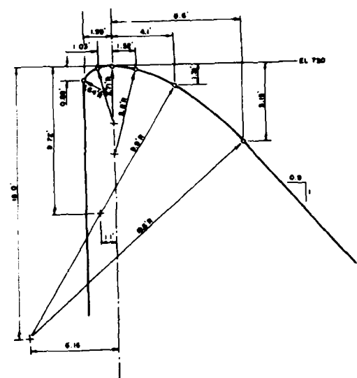
SPILLWAY CREST GEOMETRY SCALE 0 1 2 3 4 5 FEET
