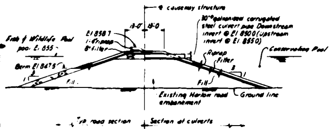
HARLOW ROAD (Overflow Section)
