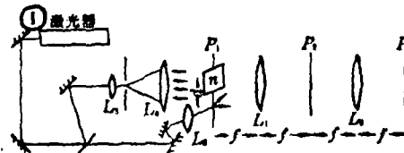
Fig. 3 Arrangement of experimental devices. Key: 1-Laser
