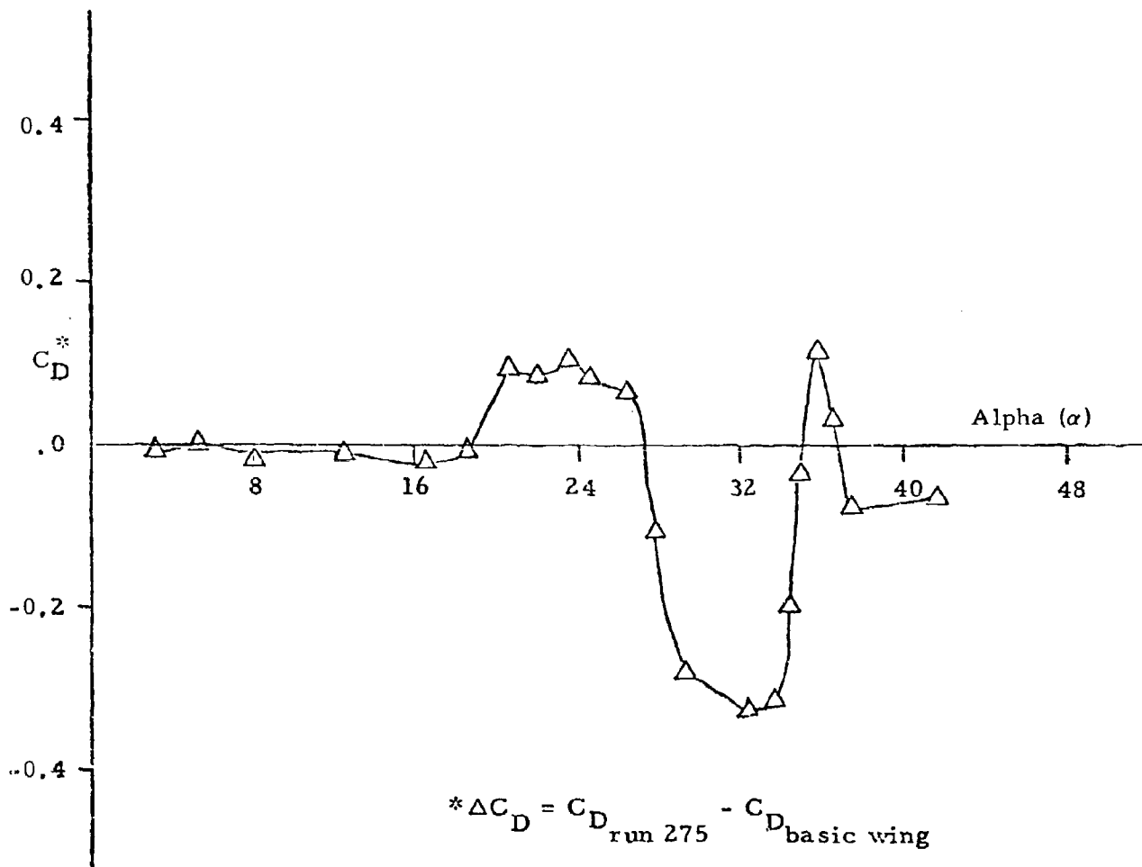
Figure 16. Change in Drag Associated with Leading Edge Modification Configuration of Test Run #275
