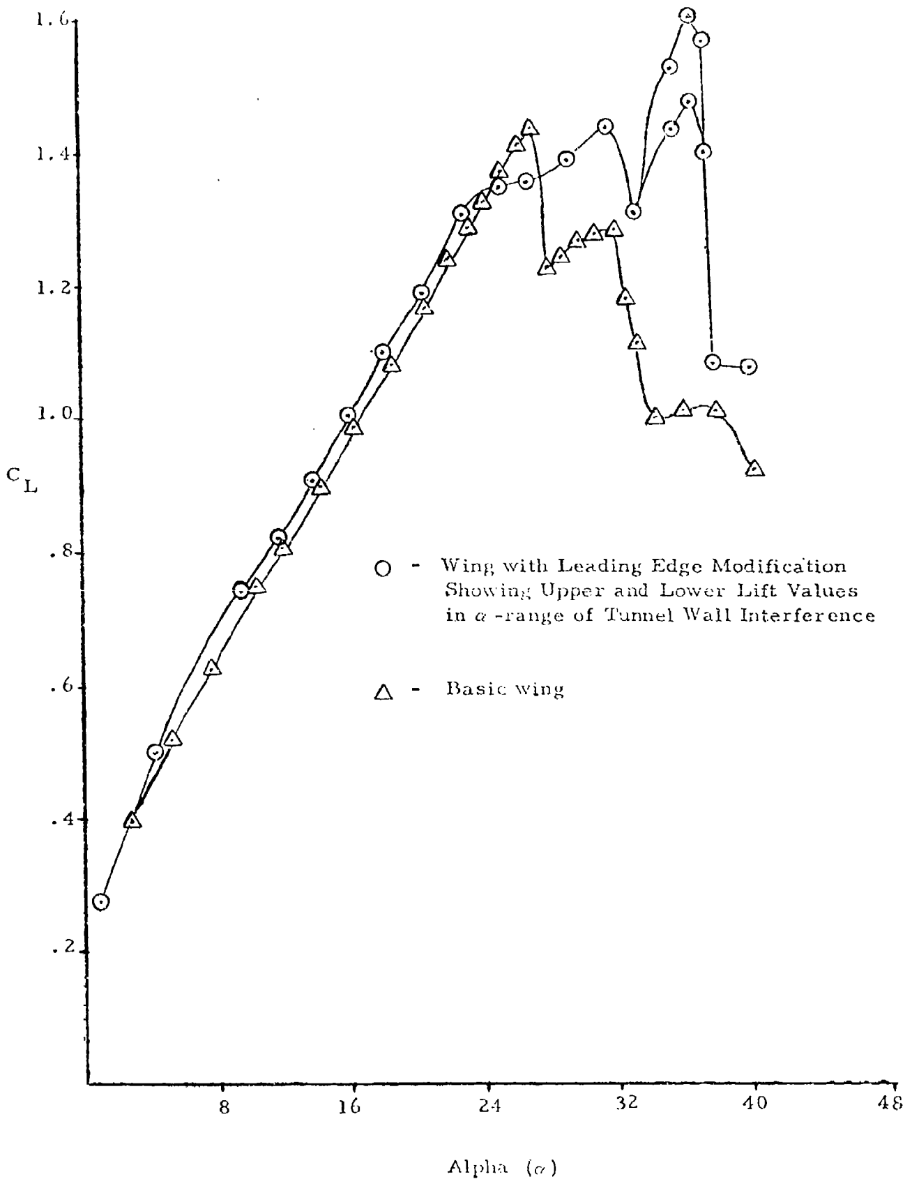
Figure 18. Comparison of Lift Characteristics between Modified and Basic 30° Swept Wing and Upper and Lower Lift Readings on the \alpha -range of Tunnel Wall Interference
