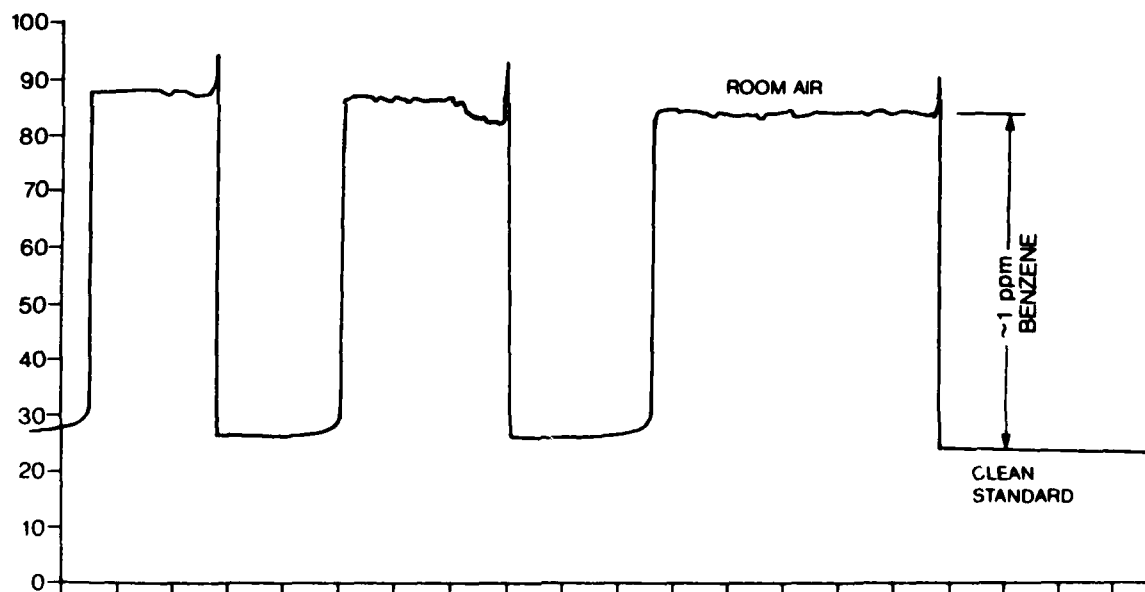
Fig.12 Results pertinent to Aircan instrument being used in the Total Ionizables Present (TIP) mode. The scan shows the difference between a clean air standard and an environment having a contamination comparable to 1 ppm benzene
