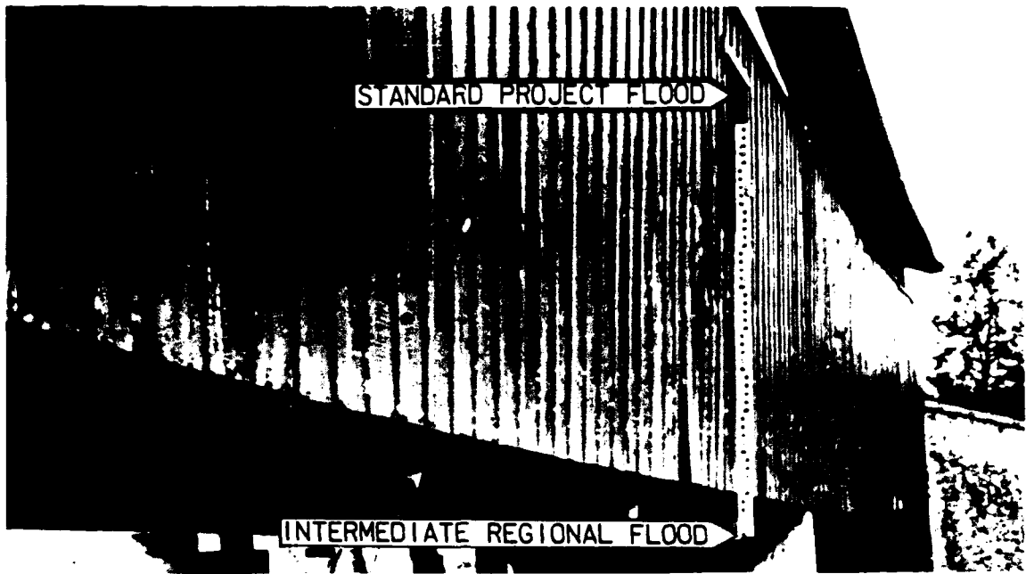
FIGURE 15 - Future flood heights at Bogert's Bridge.
