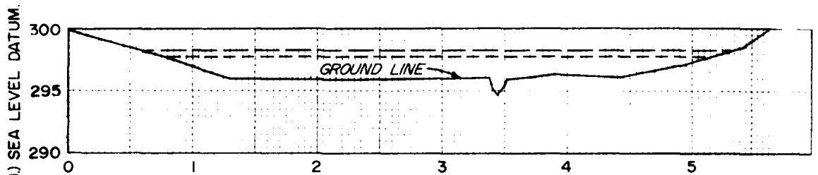
CROSS SECTION NO. 2 MILE 0.26
