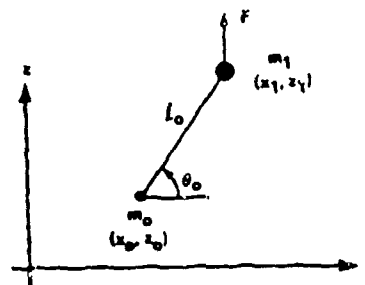
Figure 2. Geometry and Definition of Variables for Example
