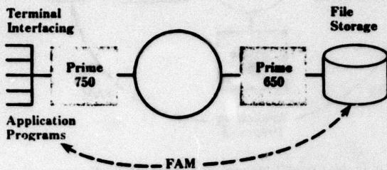
Figure 7: When a program requires little access to the file system, yet has many exchanges with terminal users, it is advantageous to use FAM to access remote files because it minimizes network traffic.
