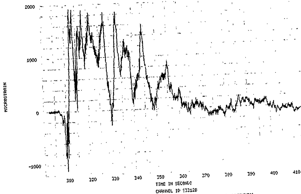
FIGURE 372. SPECIMEN 33, EVENT 78-331, STRAIN TIME HISTORY CHANNEL ID 233128
