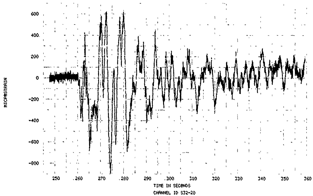
FIGURE 297. SPECIMEN 32, EVENT 78-348, STRAIN TIME HISTORY
