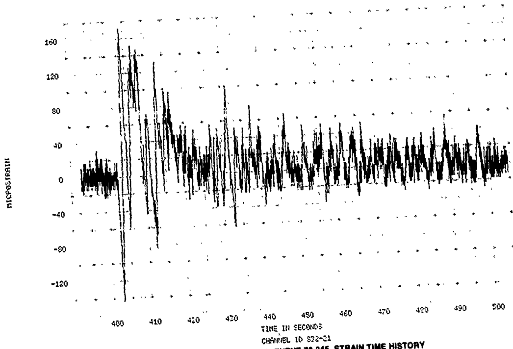
FIGURE 238. SPECIMEN 32, EVENT 78-345, STRAIN TIME HISTORY
