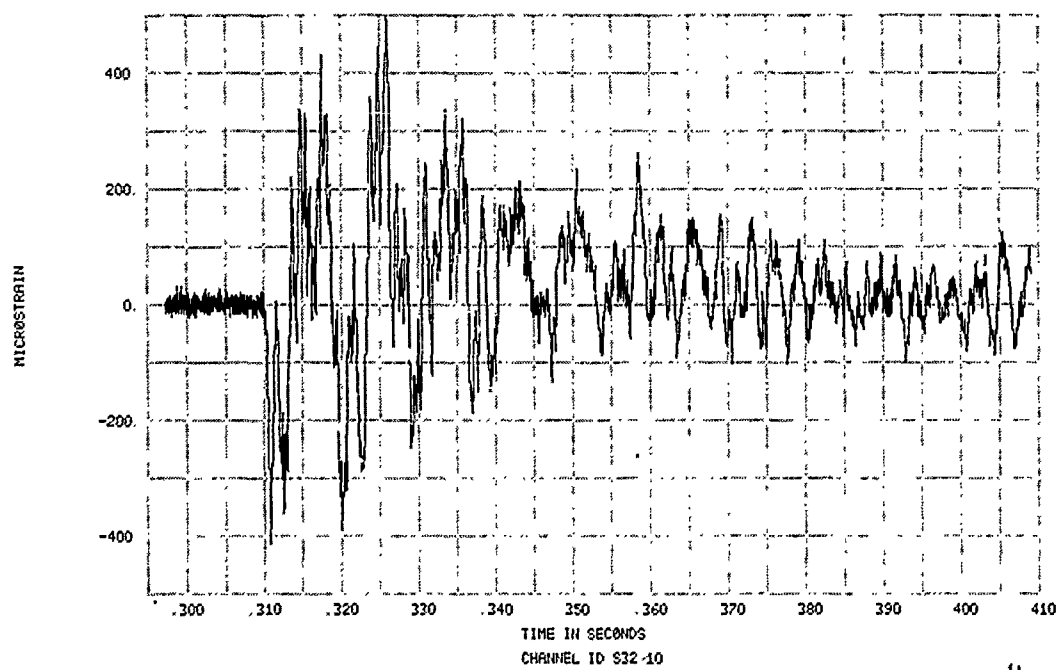
FIGURE 257. SPECIMEN 32, EVENT 78-347, STRAIN TIME HISTORY
