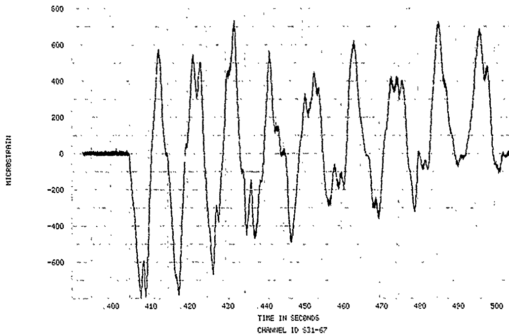
FIGURE 182. SPECIMEN 31, EVENT 78-342, STRAIN TIME HISTORY
