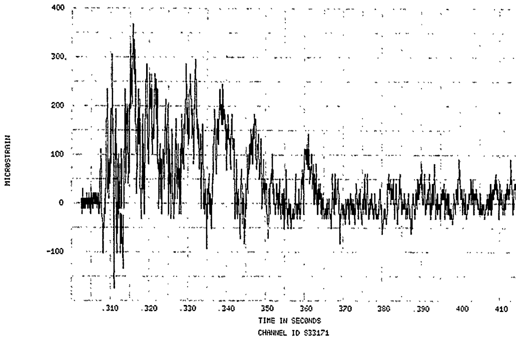
FIGURE 377. SPECIMEN 33, EVENT 78-331, STRAIN TIME HISTORY
