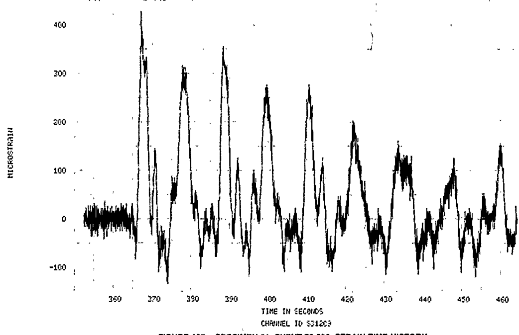
FIGURE 167. SPECIMEN 31, EVENT 79-339, STRAIN TIME HISTORY
