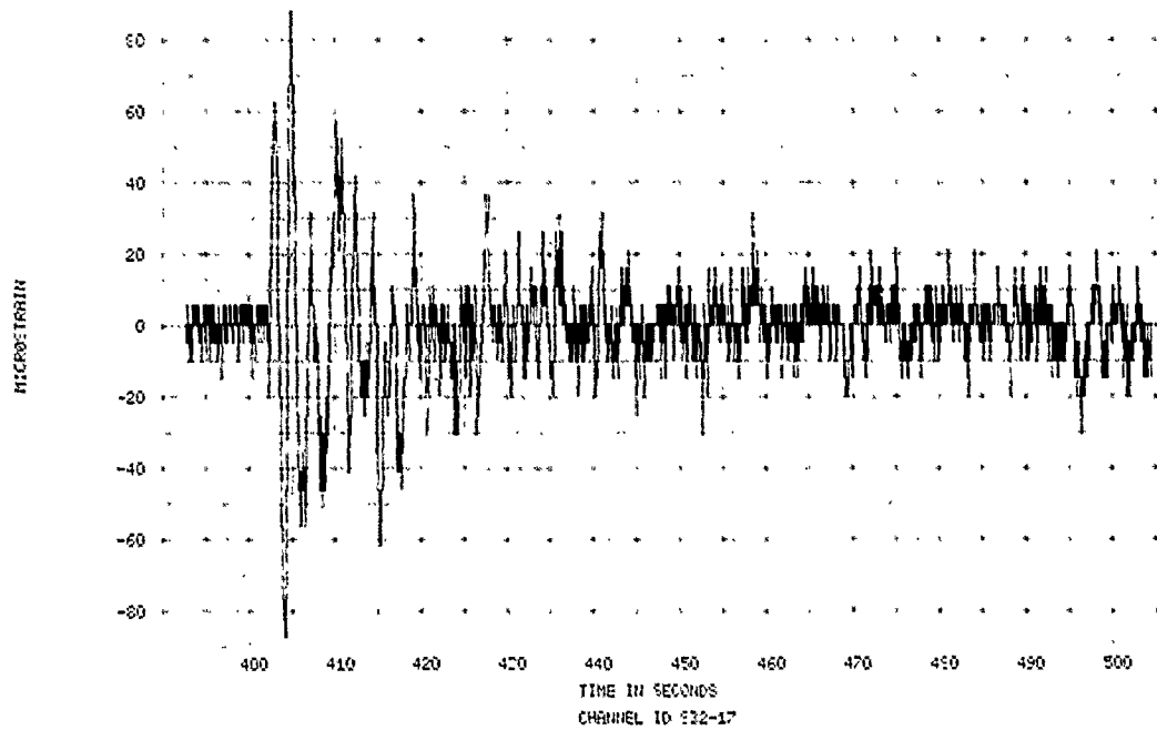
FIGURE 234. SPECIMEN 32, EVENT 78-345, STRAIN TIME HISTORY
