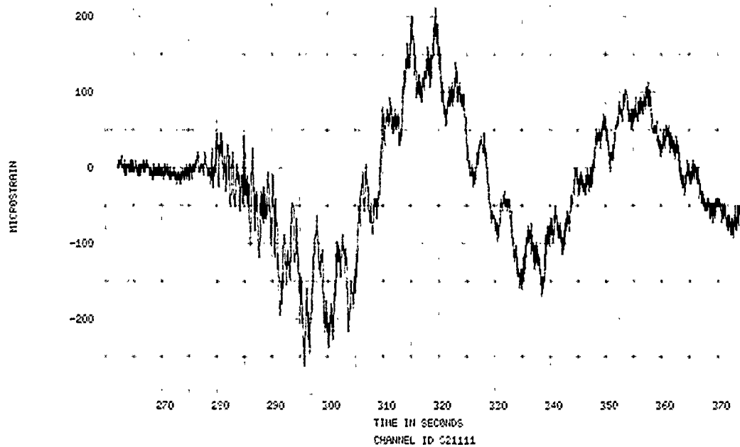
FIGURE 12. SPECIMEN 21, EVENT 78-296, STRAIN TIME HISTORY
