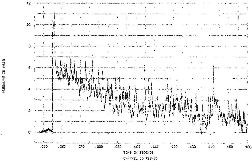
FIGURE 90. SPECIMENS 28-29, EVENT 78-355, SPECIMEN REFLECTED OVERPRESSURE TIME HISTORY
