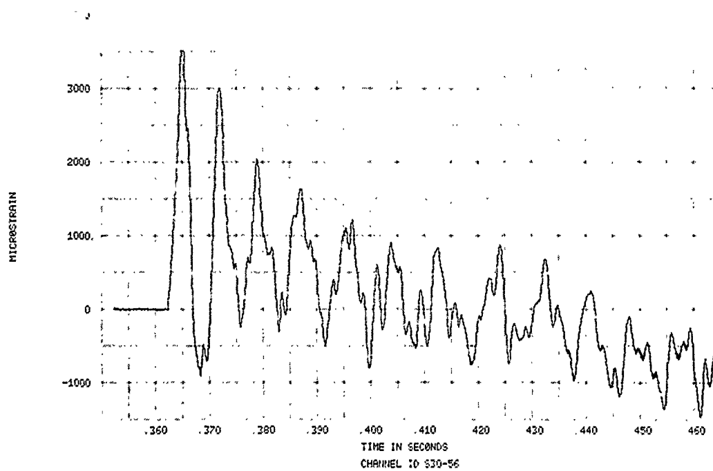
FIGURE 144. SPECIMEN 30, EVENT 78-336, STRAIN TIME HISTORY
