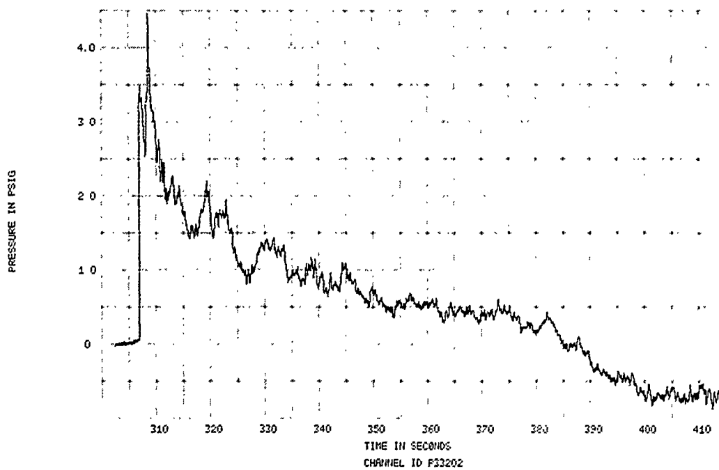
FIGURE 356. SPECIMEN 33, EVENT 78-331, SPECIMEN REFLECTED OVERPRESSURE TIME HISTORY
