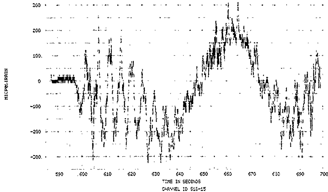
FIGURE 18. SPECIMEN 18, EVENT 78-382, STRAIN TIME HISTORY
