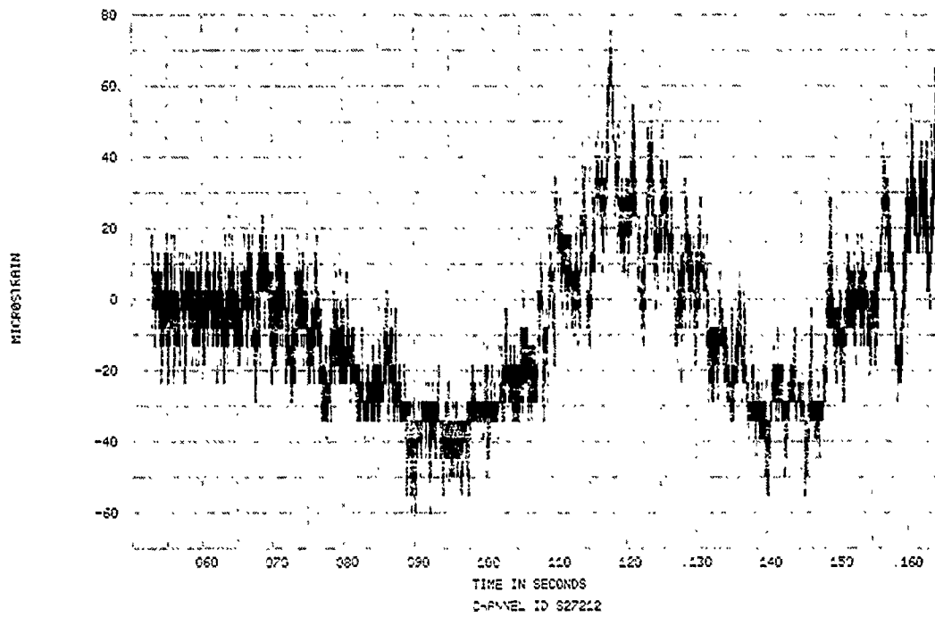
FIGURE 85. SPECIMEN 27, EVENT 78-349, STRAIN TIME HISTORY
