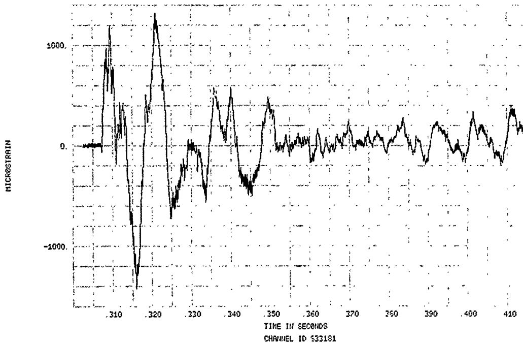
FIGURE 378. SPECIMEN 33, EVENT 78-331, STRAIN TIME HISTORY
