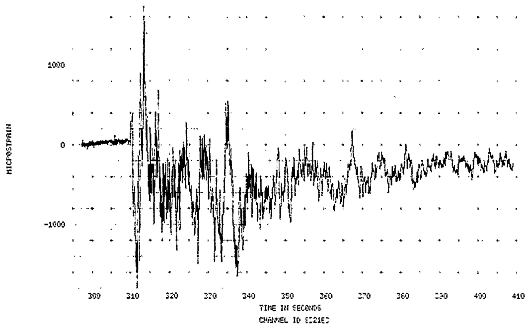
FIGURE 250. SPECIMEN 32, EVENT 70-347, STRAIN TIME HISTORY
