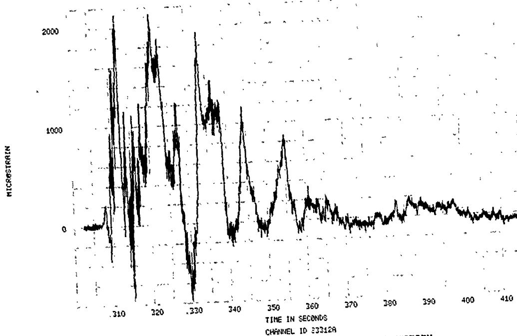
FIGURE 371. SPECIMEN 33, EVENT 78-331, STRAIN TIME HISTORY CHANNEL ID 233128
