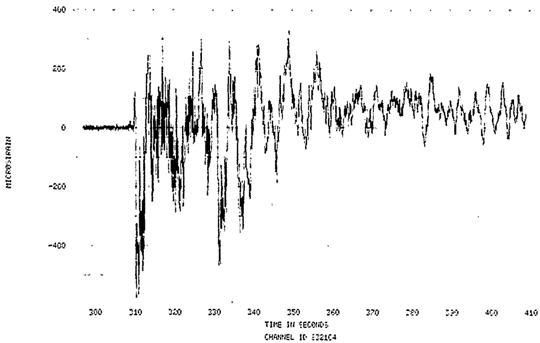
FIGURE 251. SPECIMEN 32, EVENT 70-347, STRAIN TIME HISTORY
