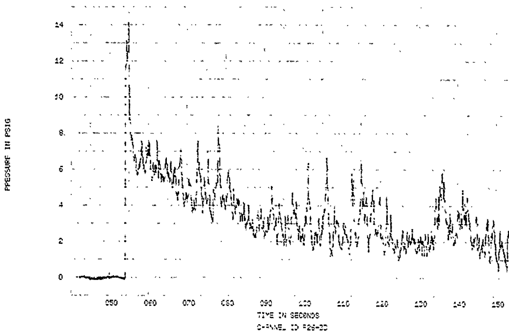
FIGURE 91. SPECIMENS 26-27, EVENT 78-351, SPECIMEN REFLECTED OVERPRESSURE TIME HISTORY
