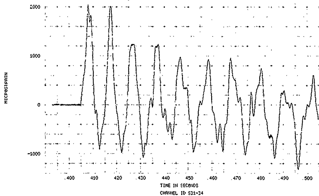
FIGURE 179. SPECIMEN 31, EVENT 78-342, STRAIN TIME HISTORY
