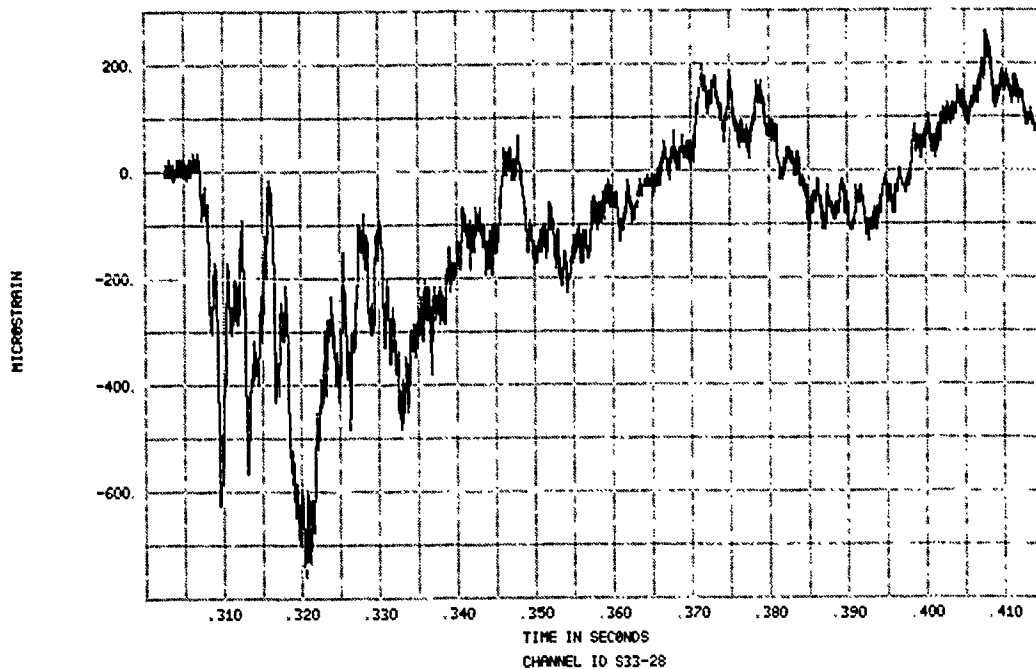
FIGURE 366. SPECIMEN 33, EVENT 78-331, STRAIN TIME HISTORY
