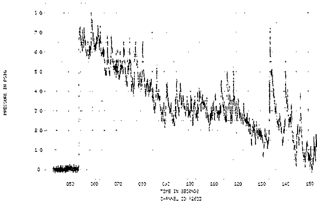
FIGURE 48. SPECIMENS 22-23, EVENT 78-351, TUNNEL WALL INCIDENT OVERPRESSURE TIME HISTORY
