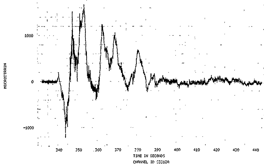
FIGURE 346. SPECIMEN 33, EVENT 78-330, STRAIN TIME HISTORY
