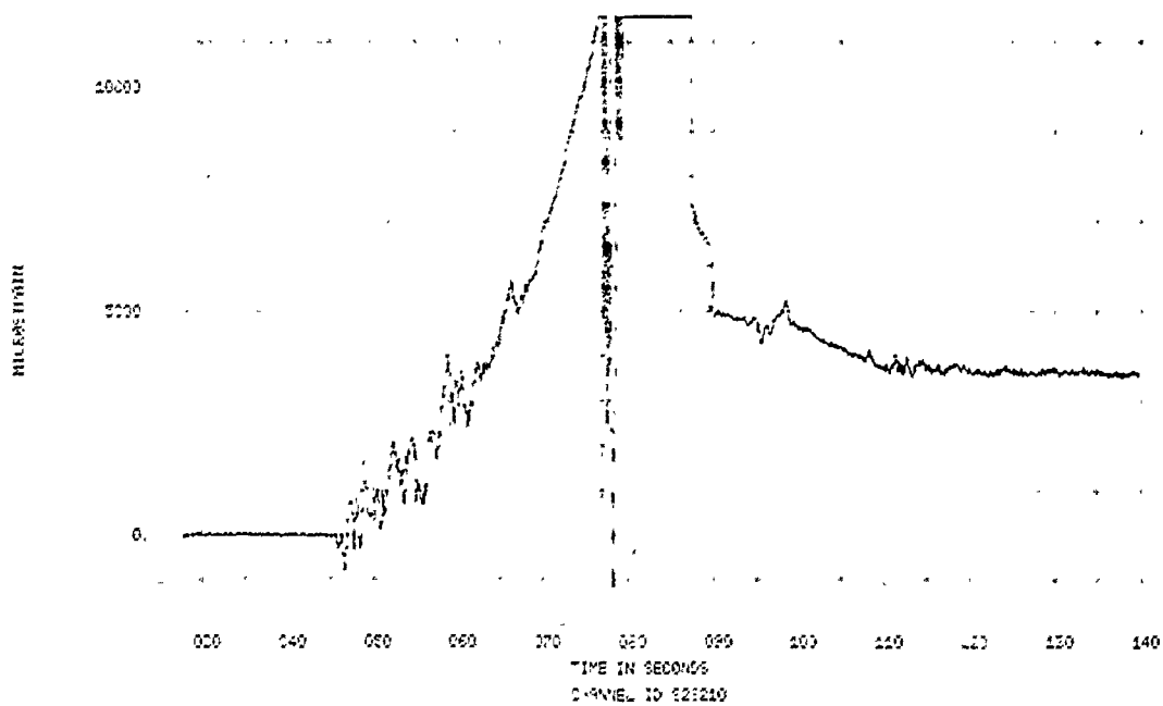
FIGURE 105. SPECIMEN 28, EVENT 78-358, STRAIN TIME HISTORY
