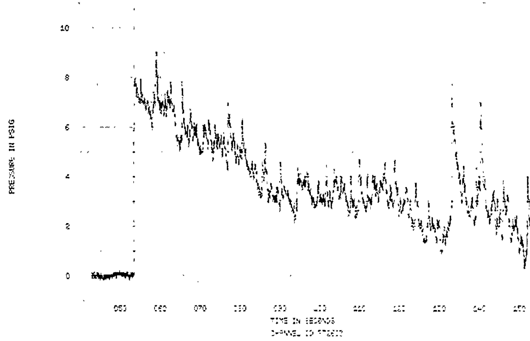
FIGURE 49. SPECIMENS 22-23, EVENT 78-351, TUNNEL WALL REFLECTED OVERPRESSURE TIME HISTORY
