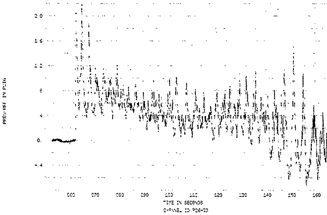
FIGURE 81. SPECIMENS 26-27, EVENT 78-349, SPECIMEN REFLECTED OVERPRESSURE TIME HISTORY
