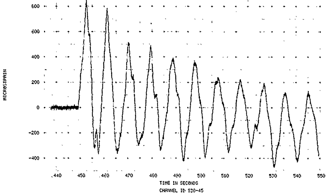
FIGURE 119. SPECIMEN 30, EVENT 78-334, STRAIN TIME HISTORY
