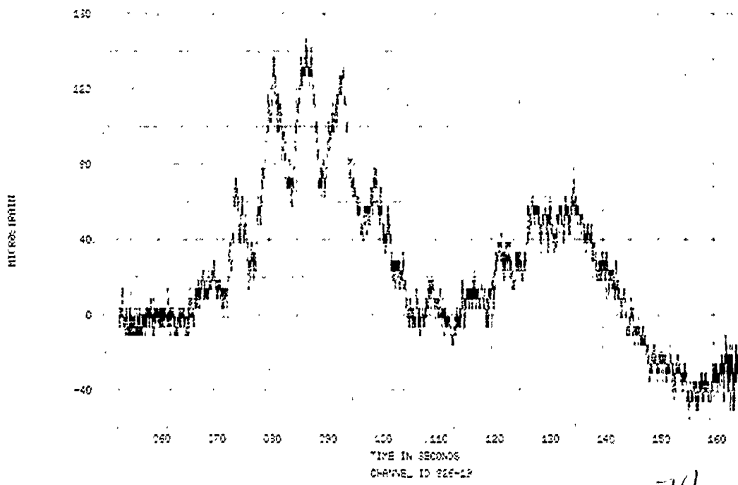
FIGURE 82. SPECIMEN 26, EVENT 78-349, STRAIN TIME HISTORY
