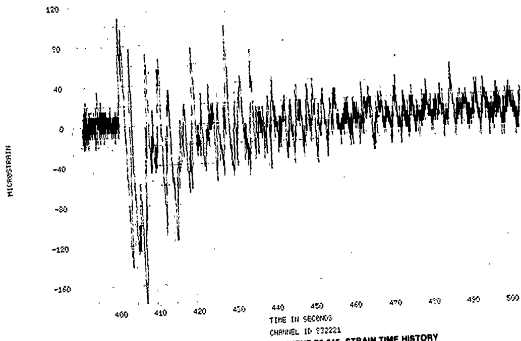
FIGURE 239. SPECIMEN 32, EVENT 78-345, STRAIN TIME HISTORY
