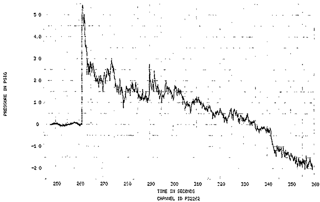
FIGURE 277. SPECIMEN 32, EVENT 78-348, SPECIMEN REFLECTED OVERPRESSURE TIME HISTORY
