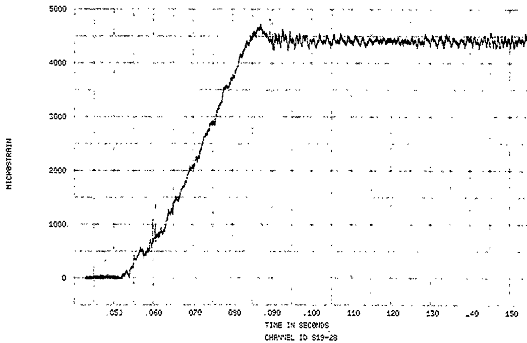
FIGURE 28. SPECIMEN 19, EVENT 78-363, STRAIN TIME HISTORY
