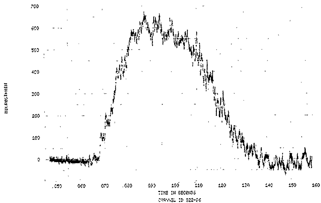
FIGURE 45. SPECIMEN 22, EVENT 78-350, STRAIN TIME HISTORY
