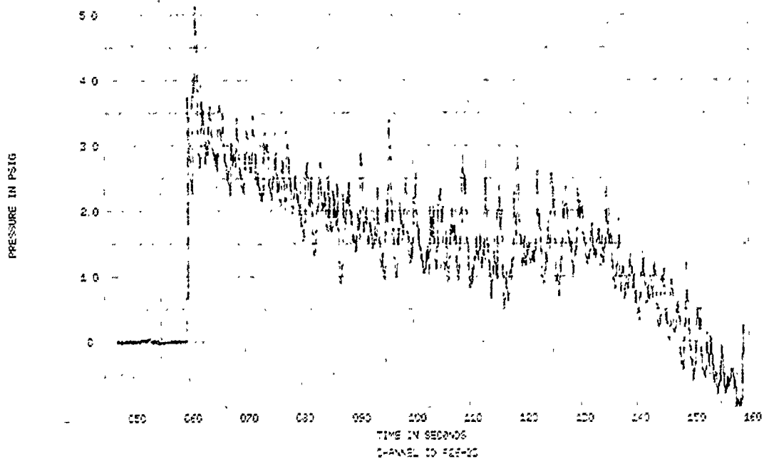
FIGURE 86. SPECIMENS 26-27, EVENT 78-350, SPECIMEN REFLECTED OVERPRESSURE TIME HISTORY
