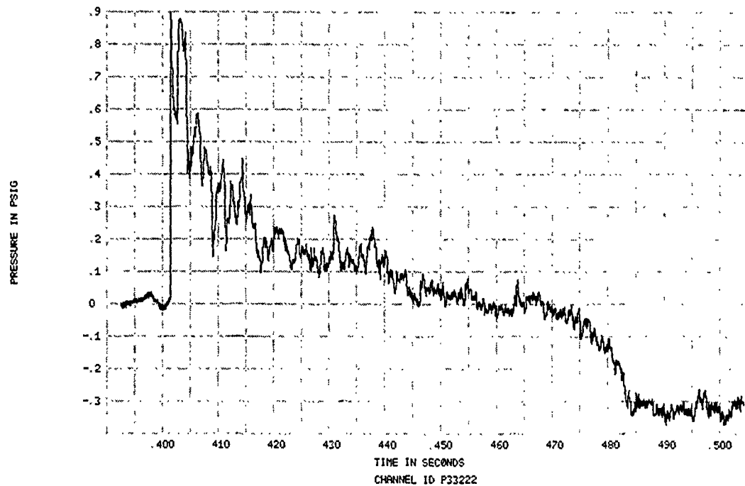
FIGURE 310. SPECIMEN 33, EVENT 78-328, SPECIMEN REFLECTED OVERPRESSURE TIME HISTORY
