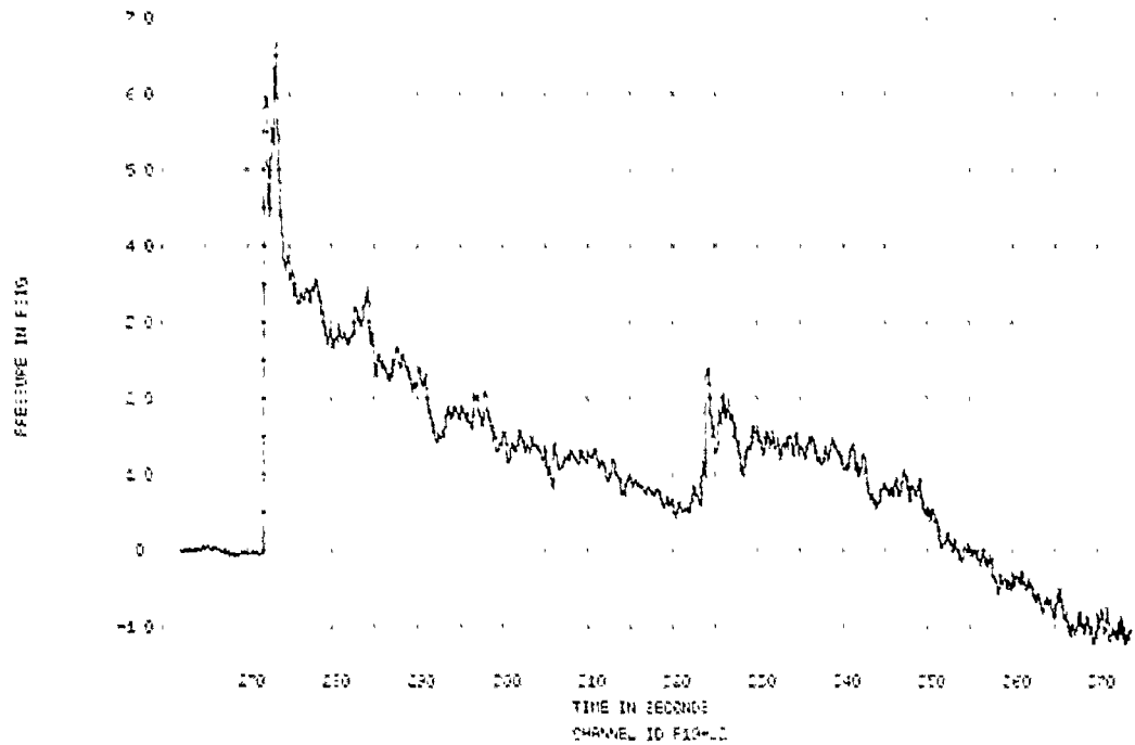
FIGURE 7. SPECIMENS 18-21, EVENT 78-298, SPECIMEN REFLECTED OVERPRESSURE TIME HISTORY
