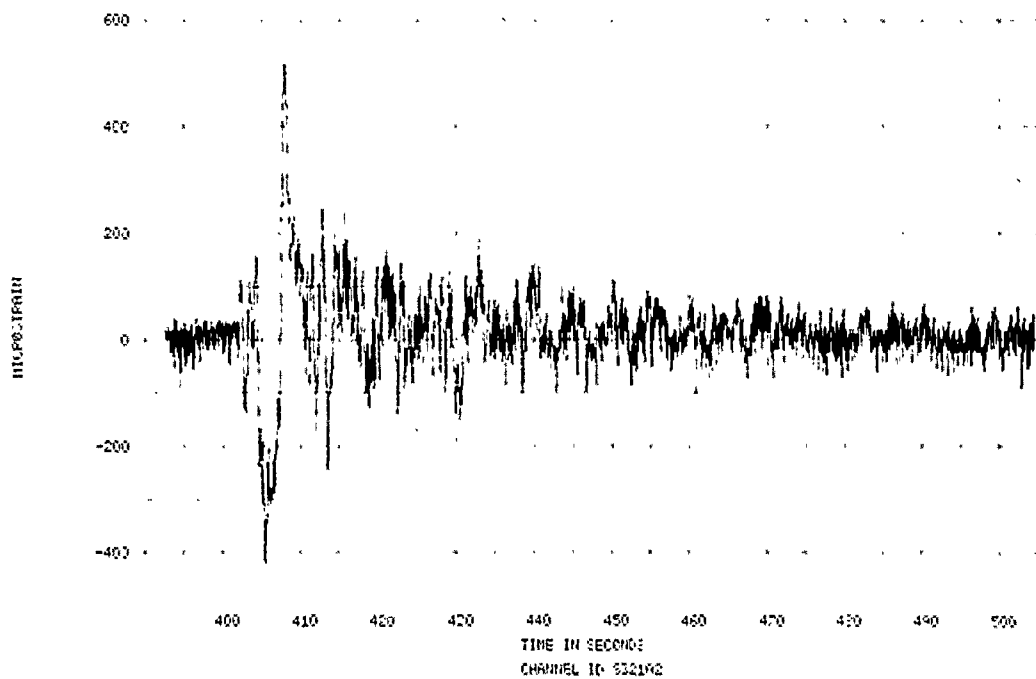
FIGURE 219. SPECIMEN 32, EVENT 78-345, STRAIN TIME HISTORY
