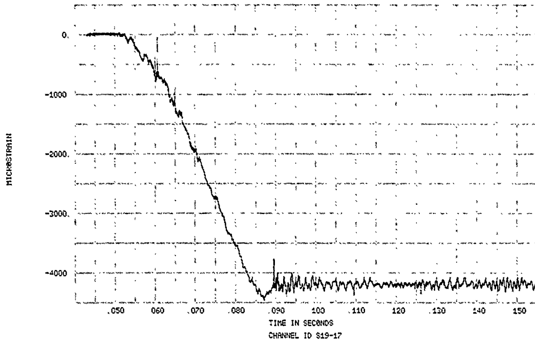
FIGURE 27. SPECIMEN 19, EVENT 78-363, STRAIN TIME HISTORY
