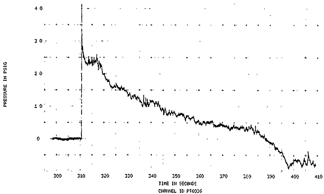
FIGURE 241. SPECIMEN 32, EVENT 78-347, TUNNEL WALL REFLECTED OVERPRESSURE TIME HISTORY
