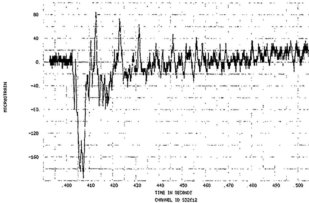
FIGURE 224. SPECIMEN 32, EVENT 78-345, STRAIN TIME HISTORY
