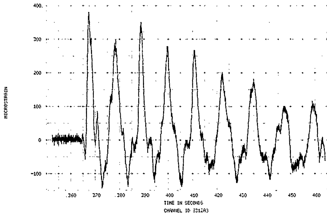
FIGURE 166. SPECIMEN 31, EVENT 78-339, STRAIN TIME HISTORY
