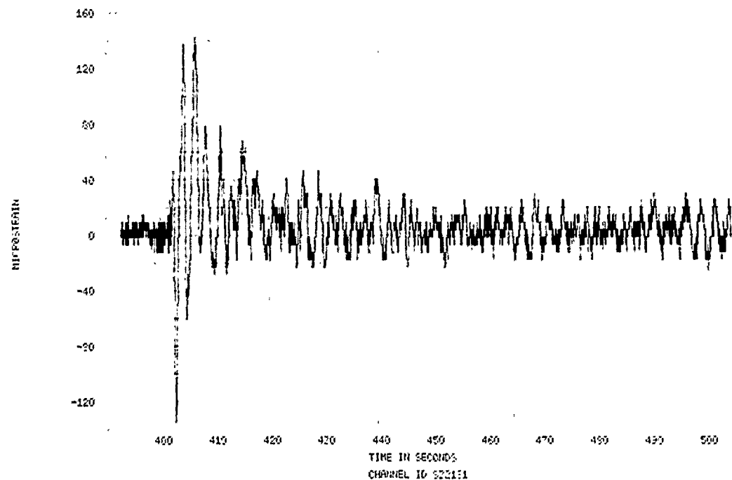
FIGURE 235. SPECIMEN 32, EVENT 78-345, STRAIN TIME HISTORY
