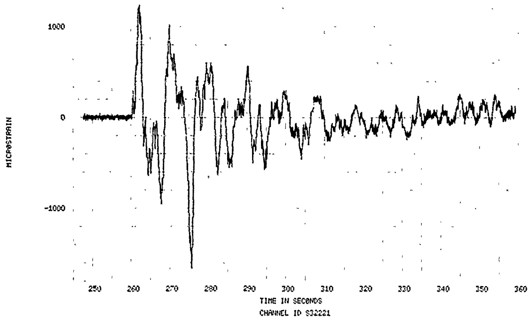
FIGURE 289. SPECIMEN 32, EVENT 78-348, STRAIN TIME HISTORY
