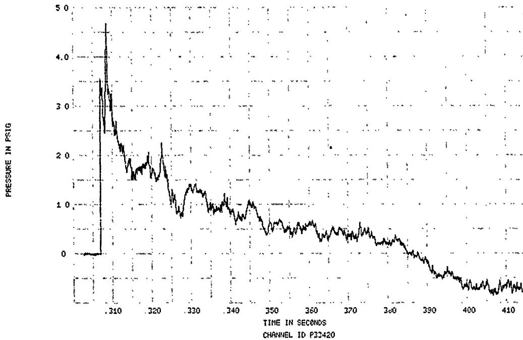
FIGURE 355. SPECIMEN 33, EVENT 78-331, SPECIMEN REFLECTED OVERPRESSURE TIME HISTORY
