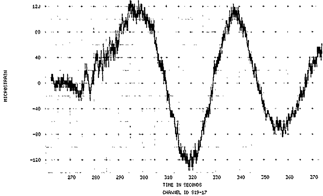
FIGURE 11. SPECIMEN 18, EVENT 78-296, STRAIN TIME HISTORY
