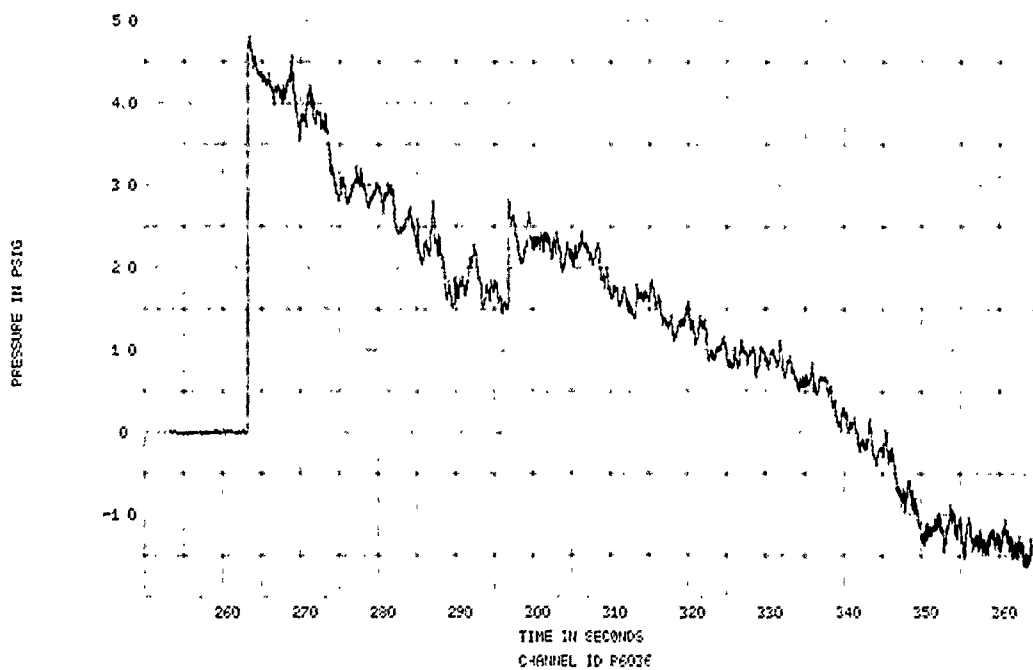
FIGURE 195. SPECIMEN 31, EVENT 78-344, TUNNEL WALL INCIDENT OVERPRESSURE TIME HISTORY
