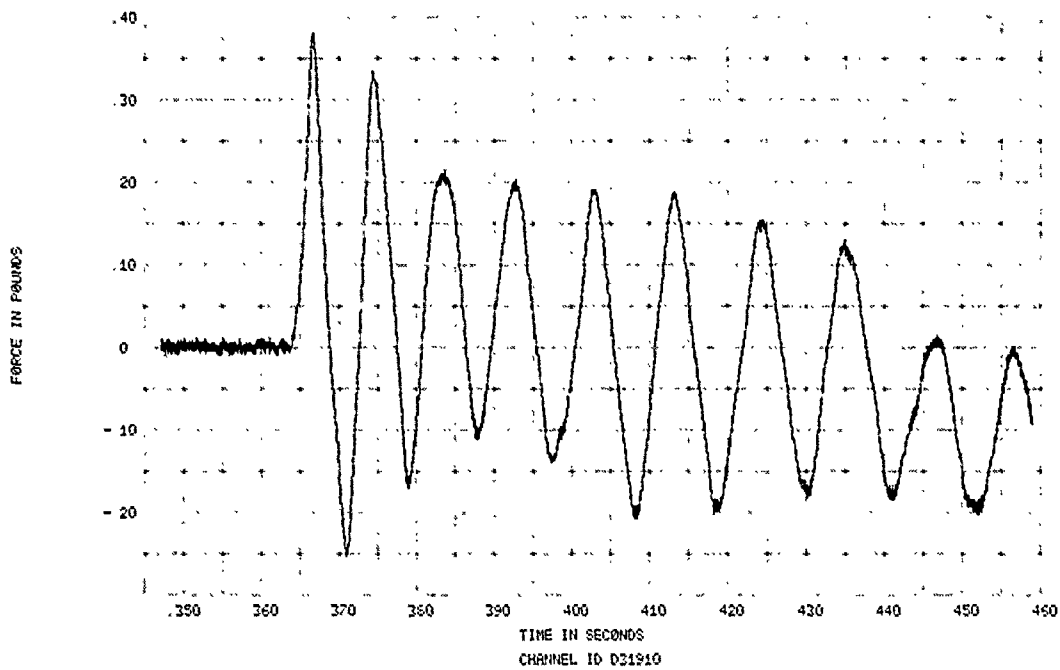
FIGURE 194. SPECIMEN 31, EVENT 78-343, DEFLECTION TIME HISTORY
