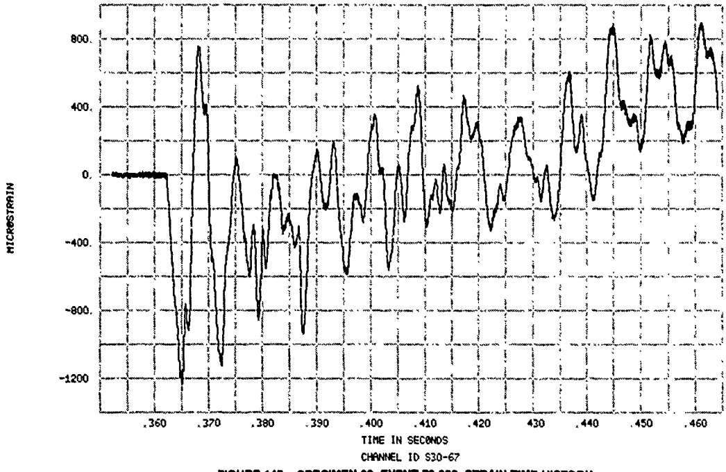
FIGURE 145. SPECIMEN 30, EVENT 70-336, STRAIN TIME HISTORY
