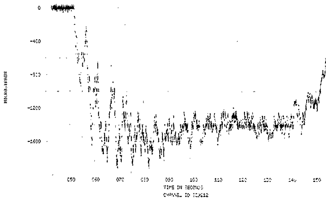
FIGURE 103. SPECIMEN 29, EVENT 78-357, STRAIN TIME HISTORY
