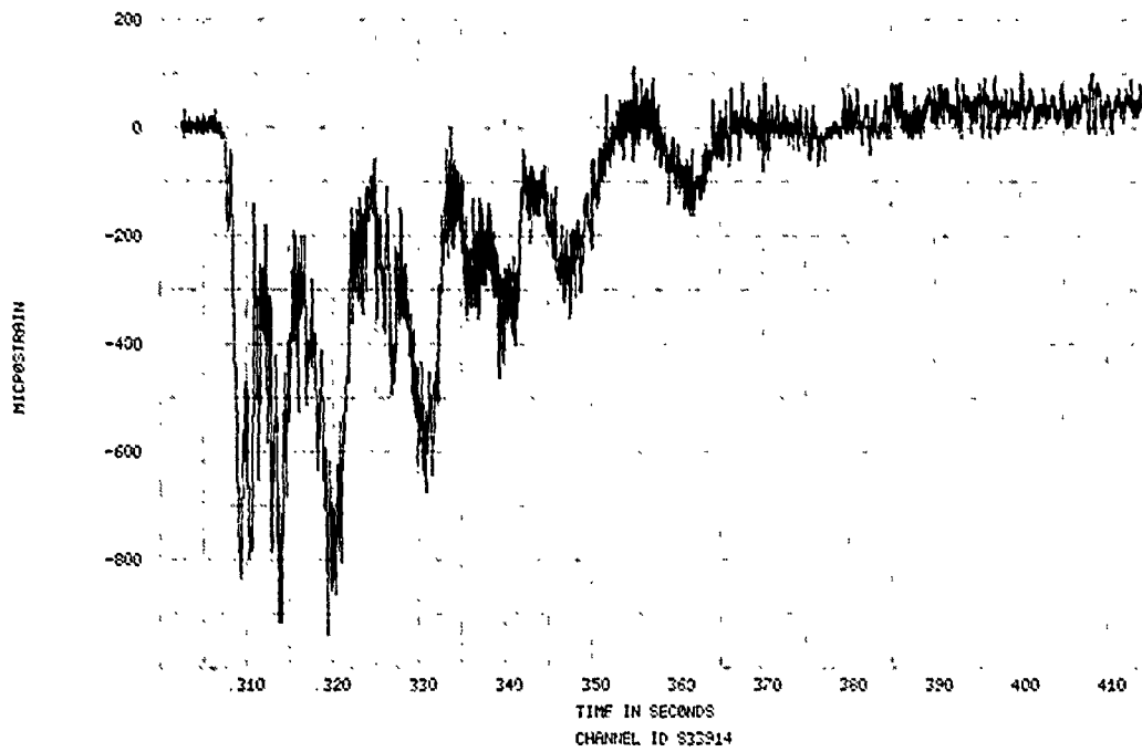
FIGURE 369. SPECIMEN 33, EVENT 78-331, STRAIN TIME HISTORY
