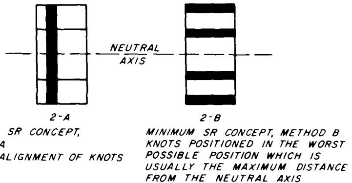
Figure 2.—Two methods to account for the reduction in section modulus due to knots.
