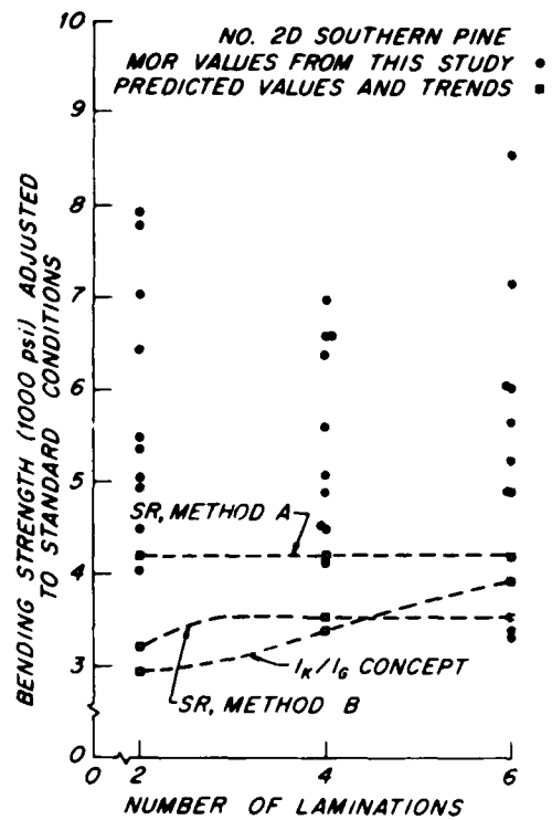
Figure 9.—Individual No. 2D southern pine MOR values from this study are shown along with predicted values and trends.
