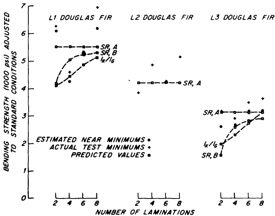
Figure 13.—Comparison of Johnson's results with predicted values. The predicted values shown for the three methods are equal to the predicted design stress values in table 3 times 2.1.
