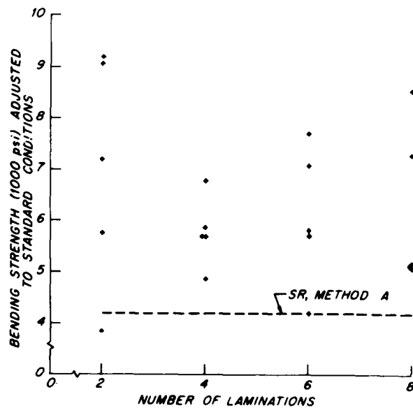
Figure 11.—Individual MOR values for Johnson's beams with knots occupying 0.3 of the cross section are shown along with the predicted values and trends using just one of the three prediction methods
