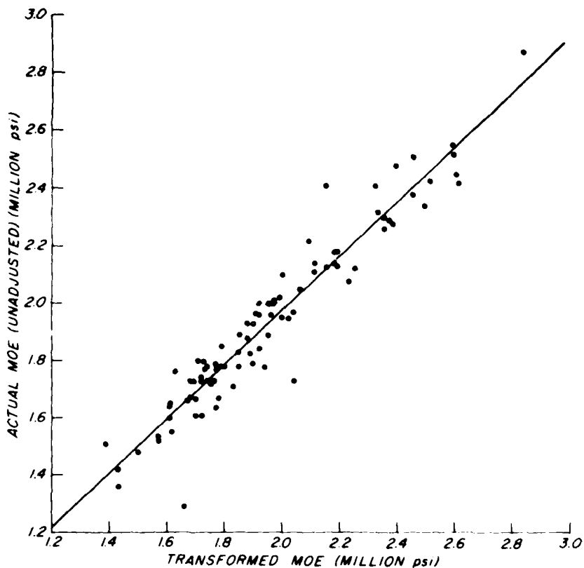
Figure 14.—Comparison of actual and transformed MOE values.
