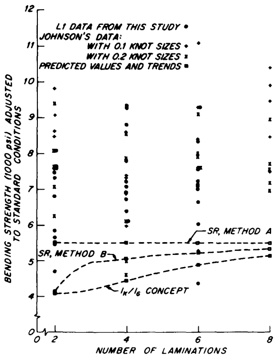
Figure 8.—Individual L1 Douglas-fir MOR values from both this study and Johnson's study are shown along with predicted values and trends.
