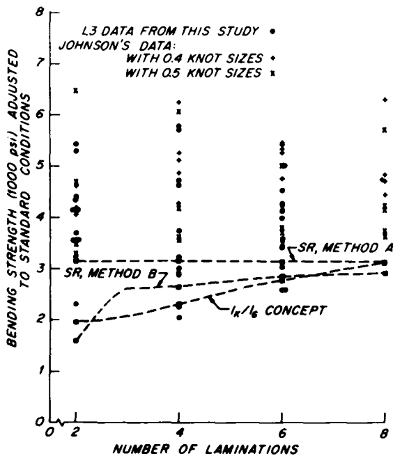
Figure 10.—Individual L3 Douglas-fir MOR values from both this study and Johnson's study are shown along with predicted values and trends.
