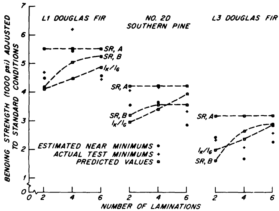
Figure 12.—Comparison of the results of this study with predicted values. The predicted values shown for the three methods are equal to the predicted design stress values in table 3 times 2.1.
