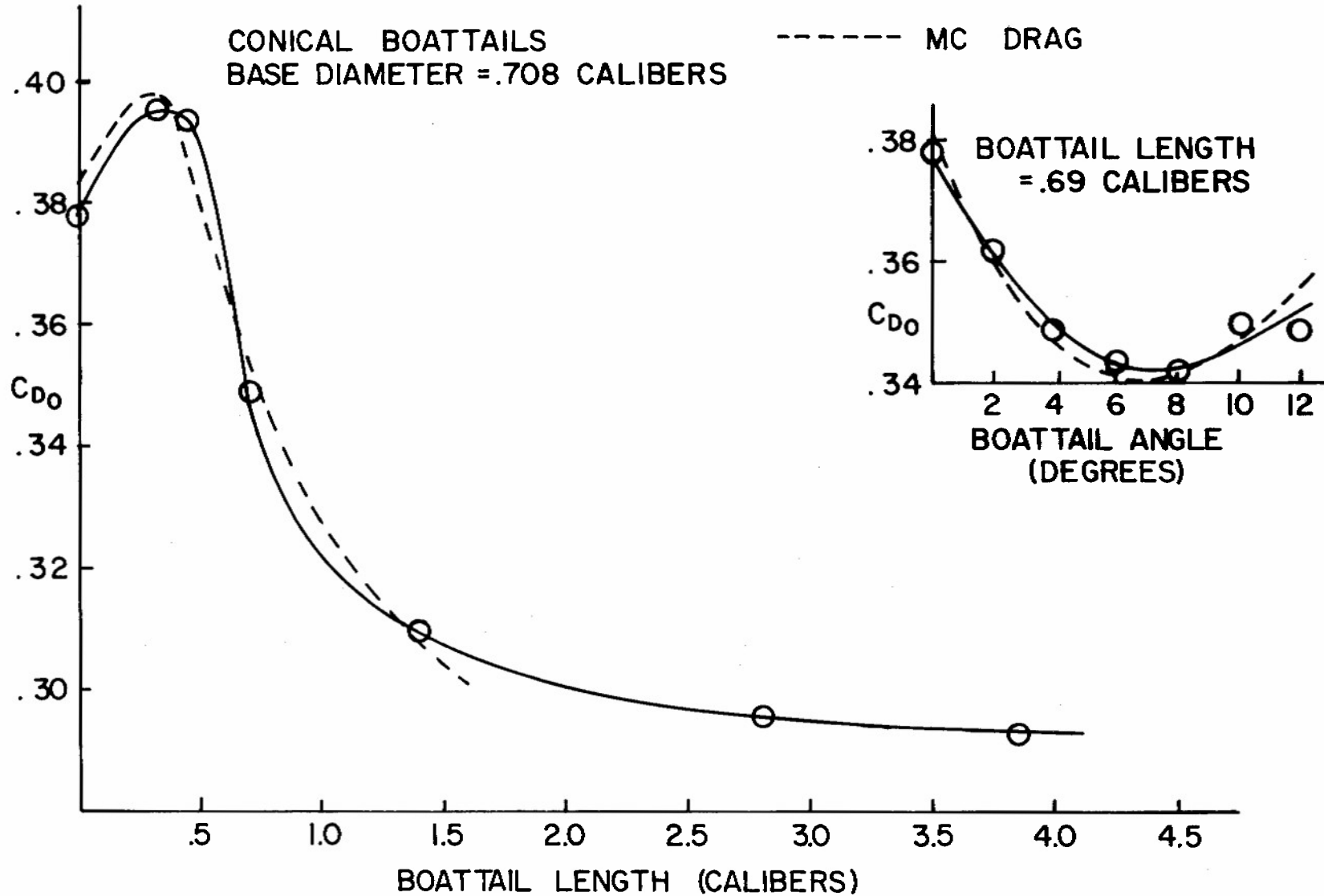
Figure 12. Effect of Boattail Length and Boattail Angle on Drag Coefficient
