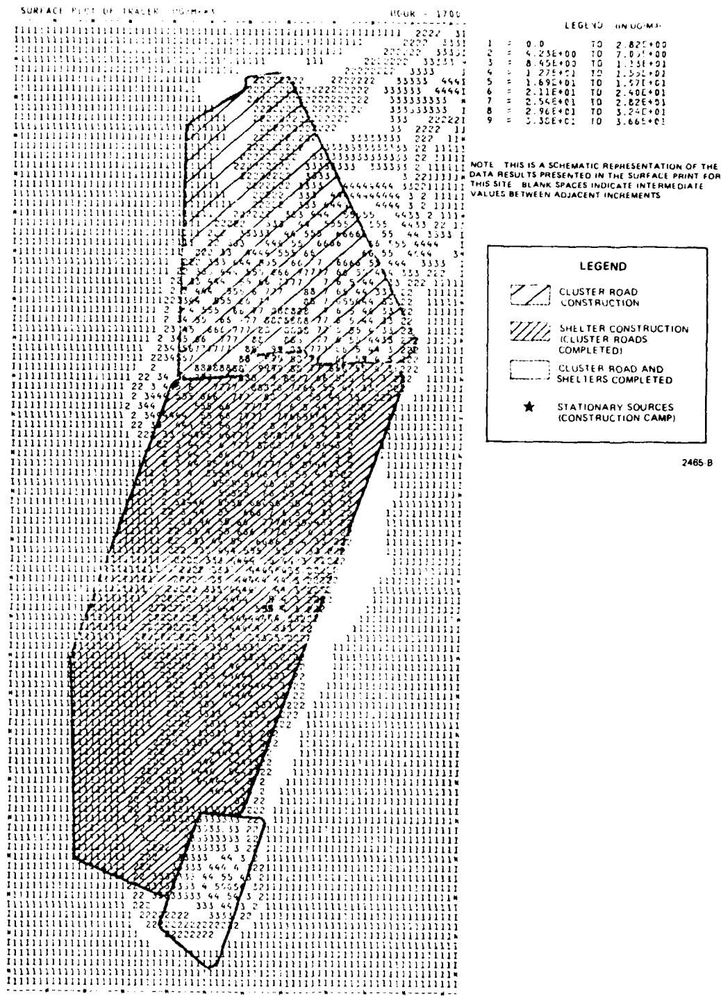
Figure 5.1.5-24. Predicted hourly particulate concentrations due to the construction of shelters and cluster roads for the Dry Lake/Delamar Valleys: mitigated emissions for the loop system.
