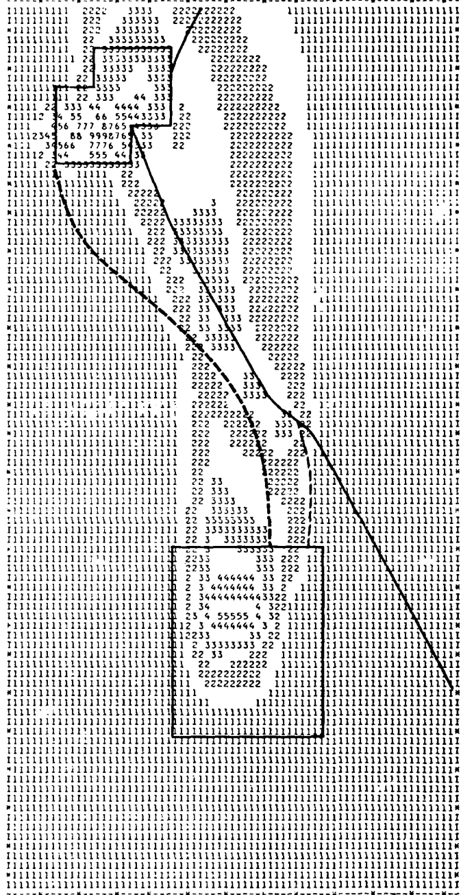
Figure 5.1.5-60. Predicted hourly CO concentrations at the Ely OB site and community.
