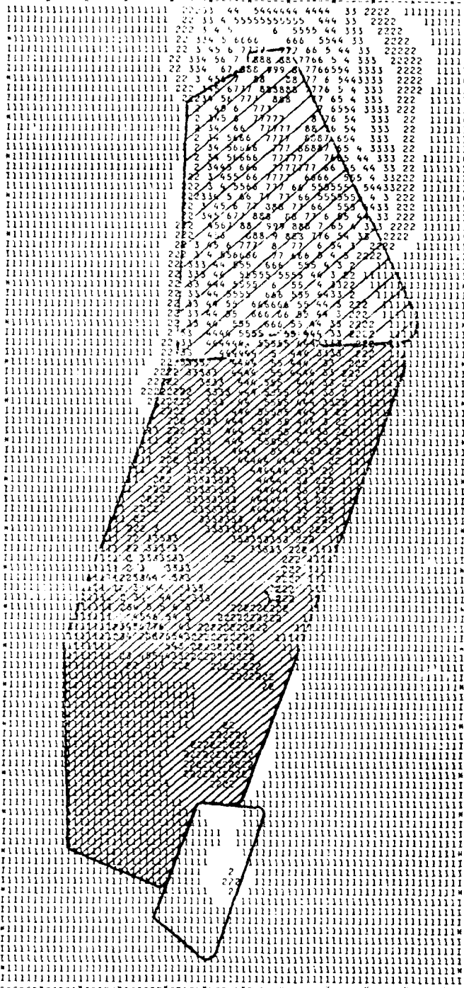
Figure 5.1.5-30. Predicted hourly particulate concentrations due to the construction of shelters and cluster roads in the Dry Lake/Delamar Valleys: unmitigated emissions for the loop system.
