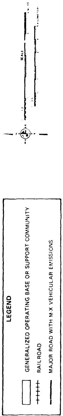
Figure 5.1.1-15 NO x emissions and emissions grid for the Clovis OB site and community (emissions in g/sec.).
