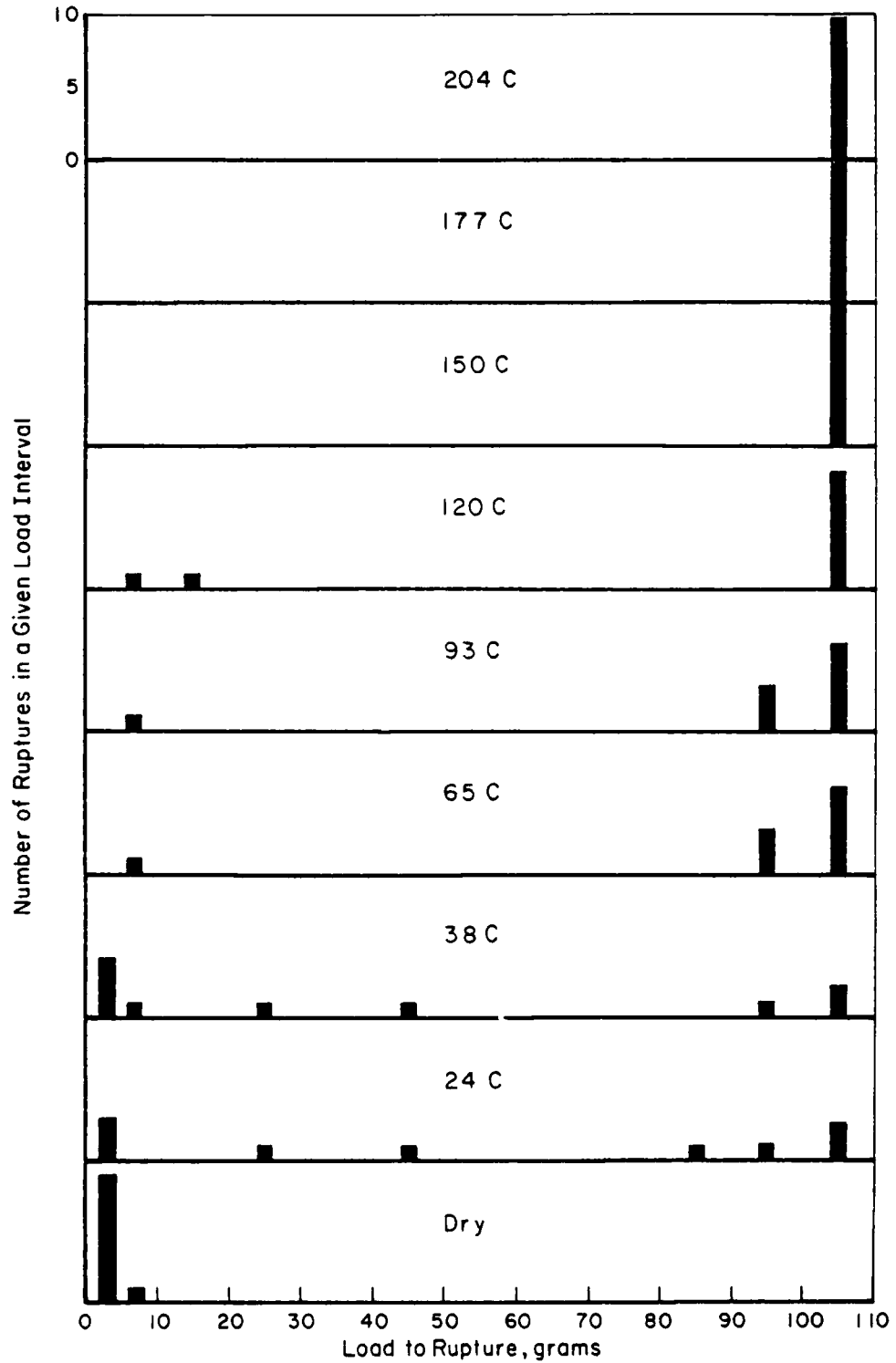
FIGURE 5. DISTRIBUTION OF LOADS-TO-RUPTURE FOR FILMS FORMED FROM E-105 CONTAINING 5 VOLUME PERCENT TCP ON ARMCO IRON AS A FUNCTION OF TEMPERATURE
