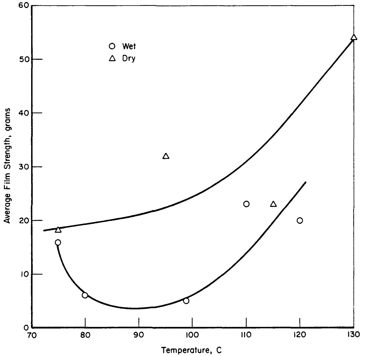
FIGURE 8. MEAN FILM RUPTURE STRENGTHS IN WET VERSUS DRY AIR ENVIRONMENTS FOR PURE E-105 FLUID ON ARMCO IRON (Each Data Point Represents the Mean Value for 20 Determinations.)
