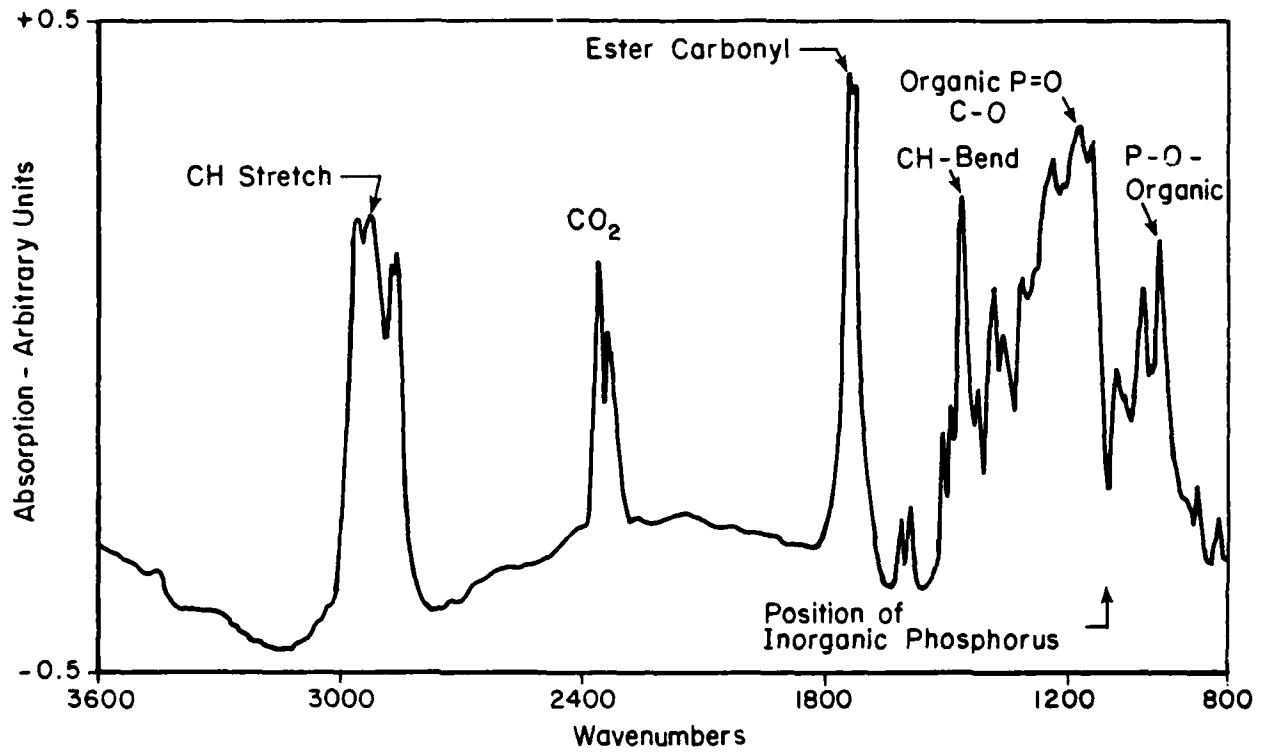
FIGURE 28. EXTERNAL REFLECTION INFRARED SPECTRUM OF ZONE-REFINED IRON PLATE AFTER REACTION WITH TCP/E-105 SOLUTION.
