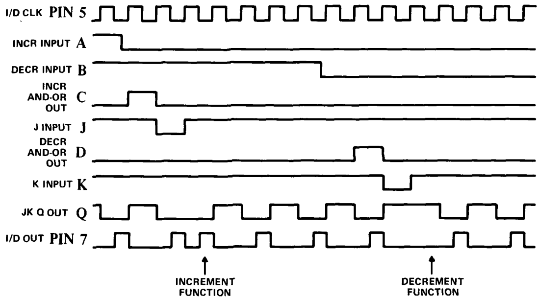
Figure 11. Increment/Decrement Circuit Waveforms
