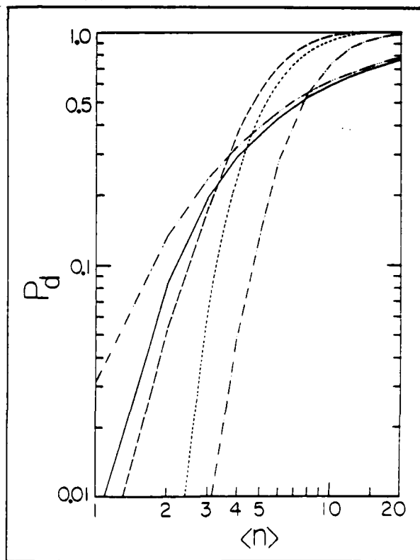
The description probabilities of n^*=5 for Poisson distribution (---), diffusion model with \beta=1 , S=6 (—), Boltzmann distributions with s=6 (---) and S=1 (—), and quantal model with \alpha = S = 1 (---).
