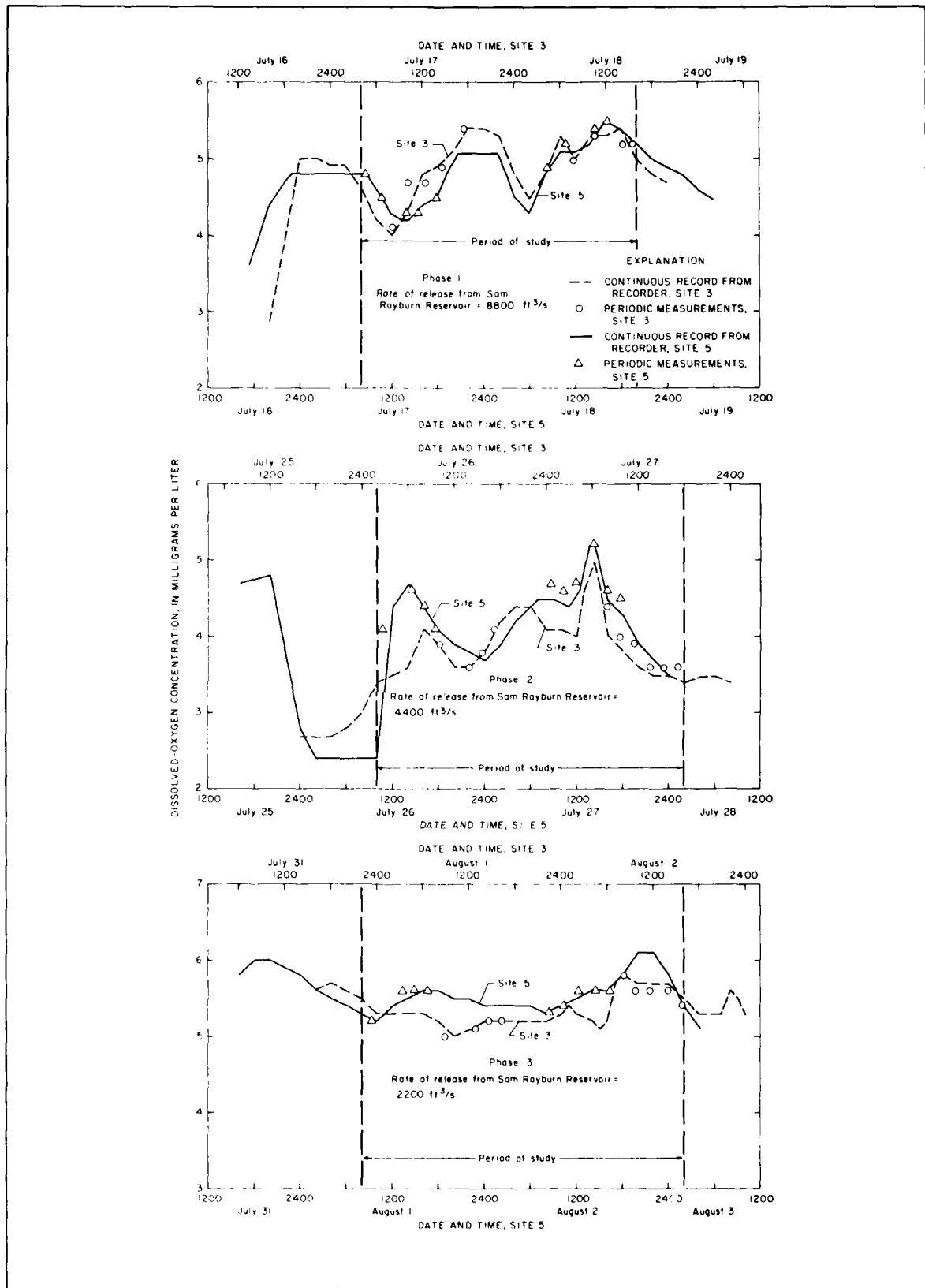
FIGURE 3.-Variations of dissolved-oxygen concentrations at sites 3 and 5 on the Angelina River
