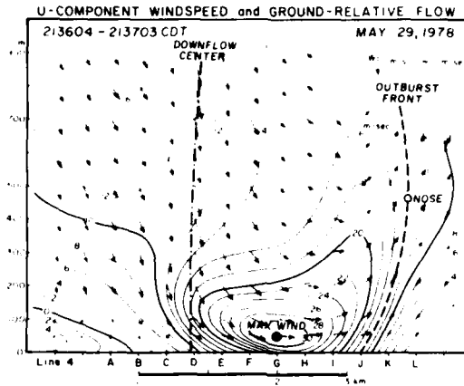
Figure 1. Isotachs of horizontal windspeeds through microburst event which occurred on 29 May 1978 during the NIMROD experiment. Vectors show x-z wind field. Maximum horizontal windspeed of 31 \text{ m s}^{-1} is estimated to occur at 50 m or lower. (Courtesy of Dr. Fujita)
