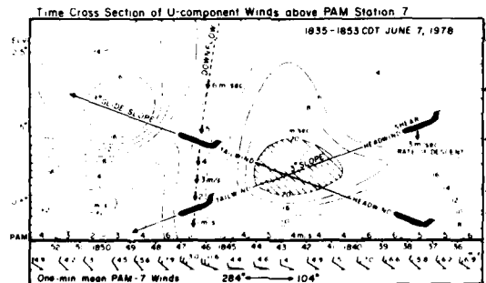
Figure 2. Hypothetical penetration through the maximum-wind core along 3-deg slopes. The headwind shear (headwind increase with time) is experienced during the approach to the core, while the tailwind shear (headwind decrease or tailwind increase with time) is encountered while flying away from the core. A strong tailwind shear results in a loss of airspeed which endangers both landing and takeoff operations. (Courtesy of Dr. Fujita)
