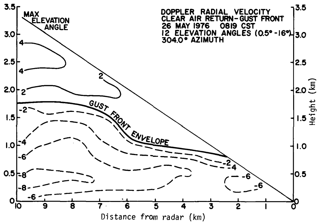
Figure 6. Clear air single Doppler wind cross section of gust front along 304° radial 26 May 1976. Positive (away from radar isotachs, \text{m s}^{-1} ) are solid, negative isotachs, dashed.
