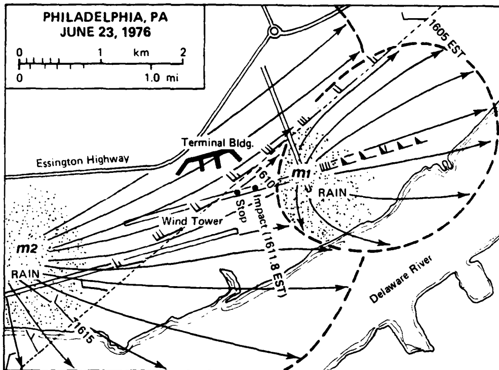
Figure 4. The path of Allegheny Flight 121 in relation to two microbursts, m1 and m2, at Philadelphia International Airport on June 23, 1976.
