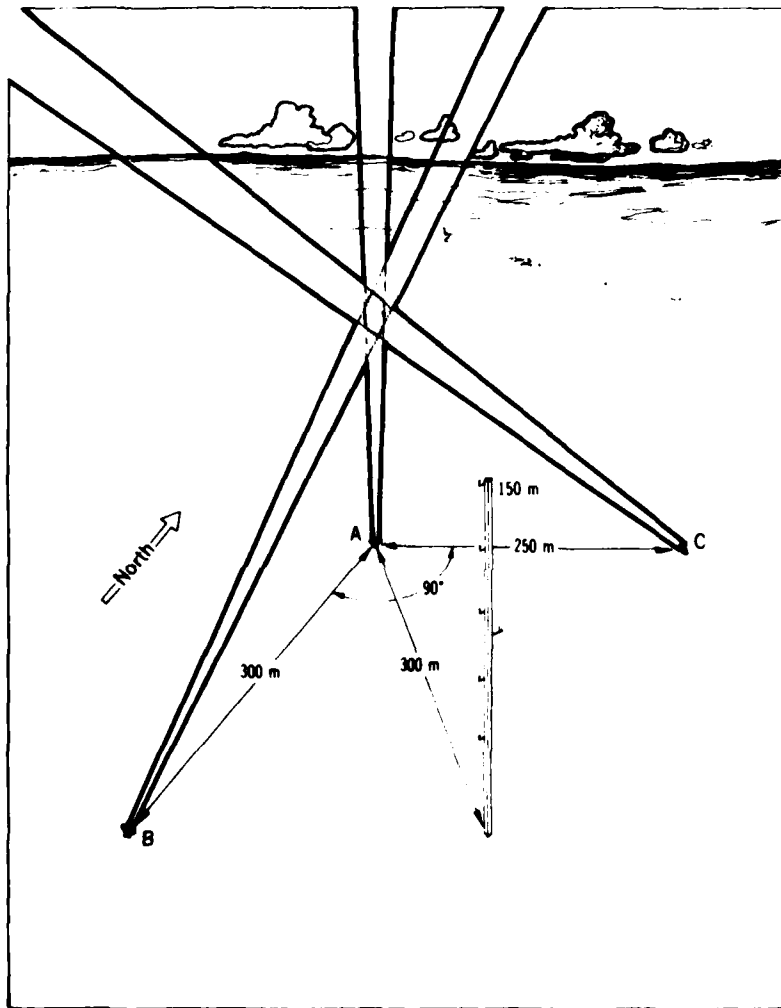
Figure 1. Basic acoustic system schematic (A, transmitter; B and C, receivers). (From Gaynor, 1977)
