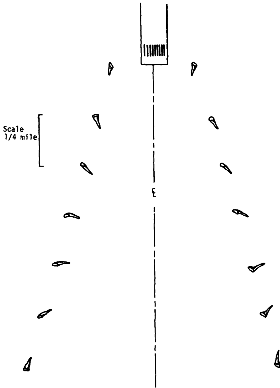
Figure 6. Placement of wind socks for wind shear indication.
