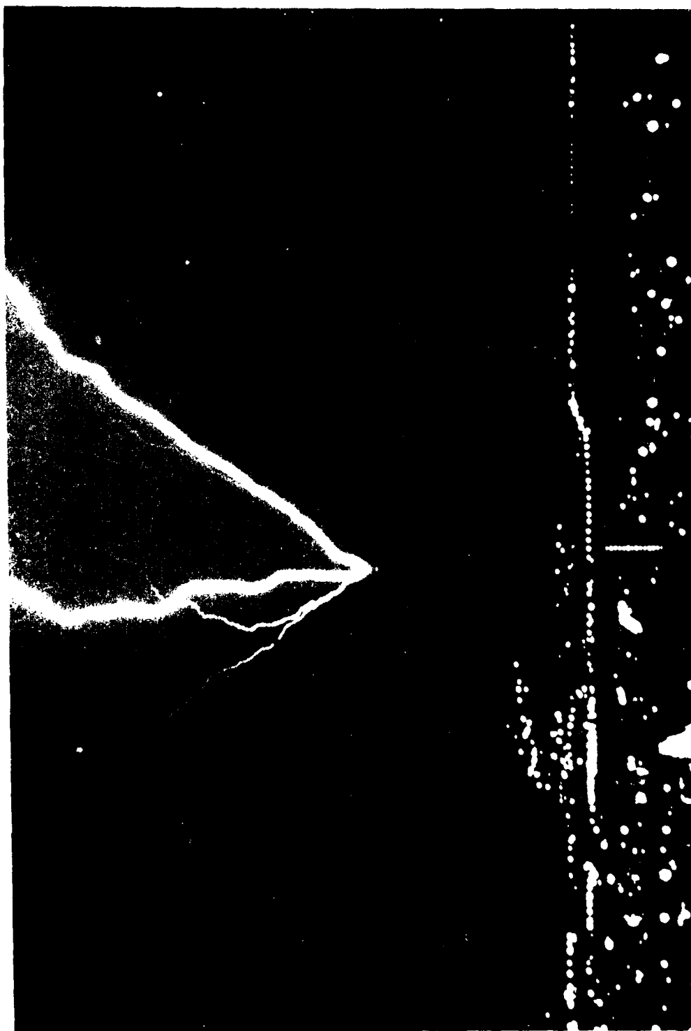
Figure 7. Upward triggered lightning flash from Mt. San Salvatore. (Maras)
