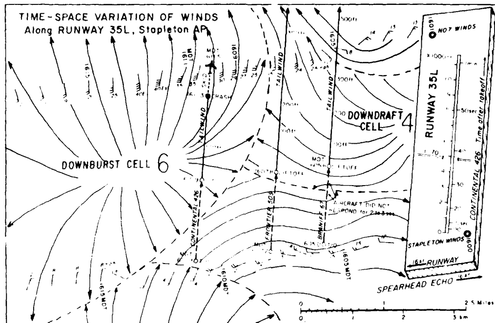
Figure 2. A time-space section by Fujita and Caracena (1977) of the winds across runway 35L of Stapleton International Airport on August 7, 1975, during the crash of Continental Flight 426.
