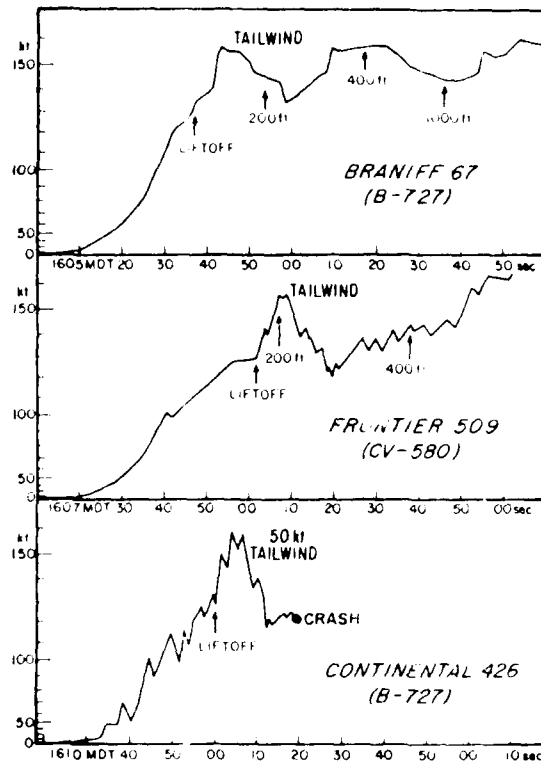
Figure 3. Flight recorder airspeed traces from the three aircraft penetrating the storm that downed Continental Flight 426. The airspeed scale is proportional to the square of the speed to depict energy.
