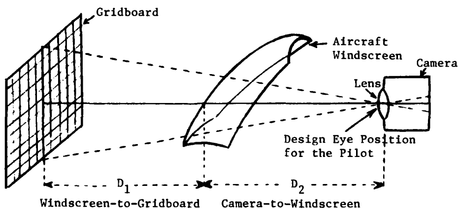
Figure 1. Photographing Geometry for Grid Line Slope Measurements.
