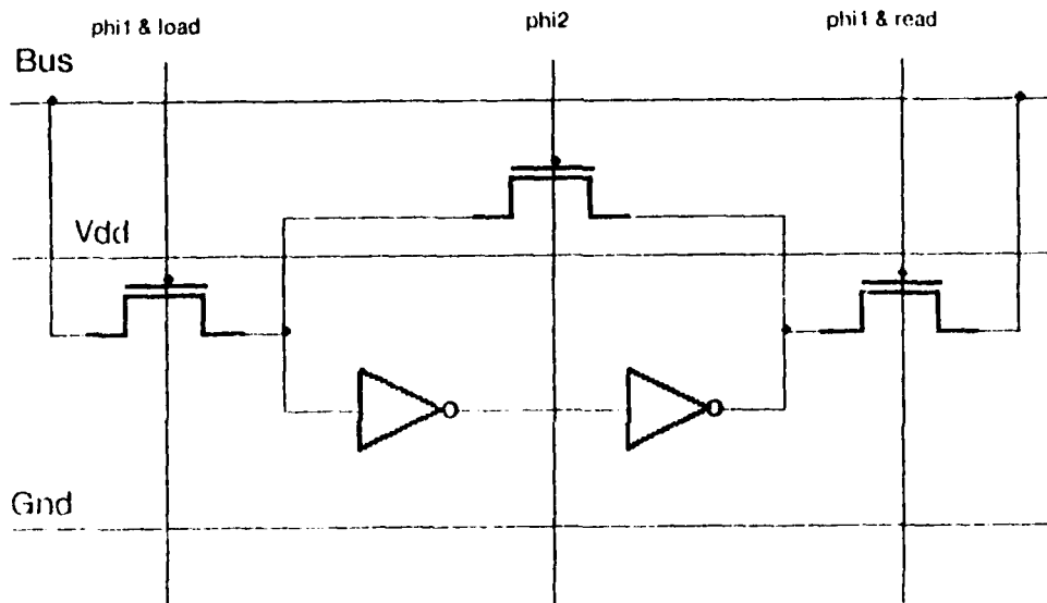
Figure 9 -- Circuit of Regcell
