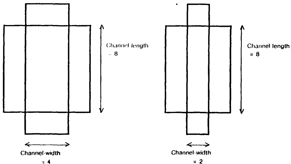
Figure 5 -- Two instances of the type PASS-TRANSISTOR
