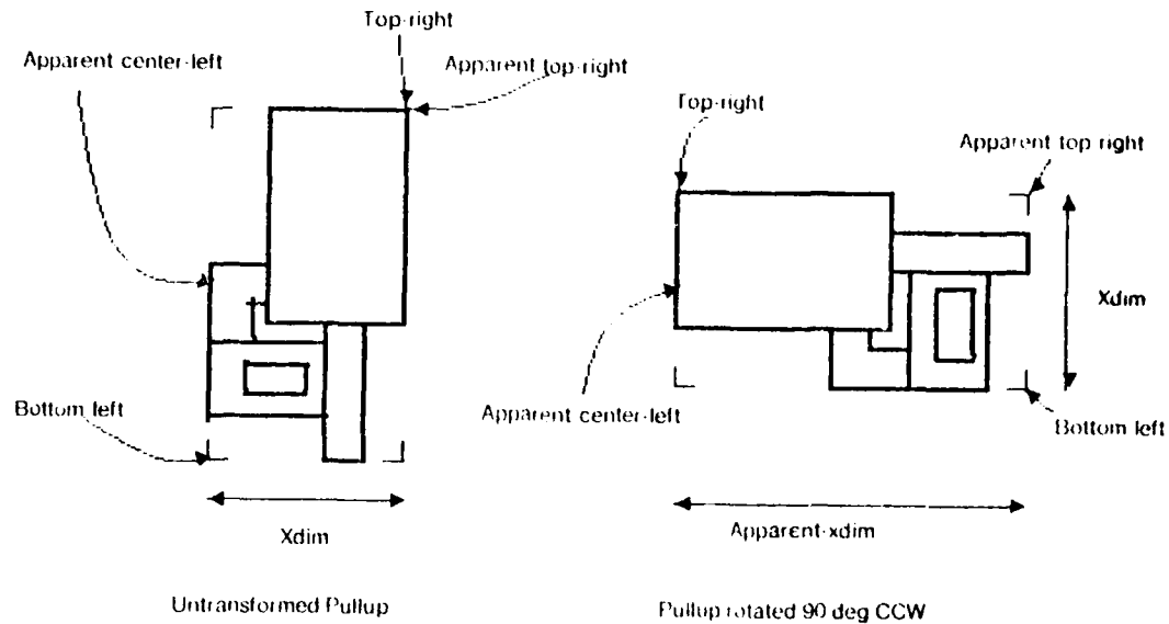
Figure 6 -- Some implicit parameters of an Instance
