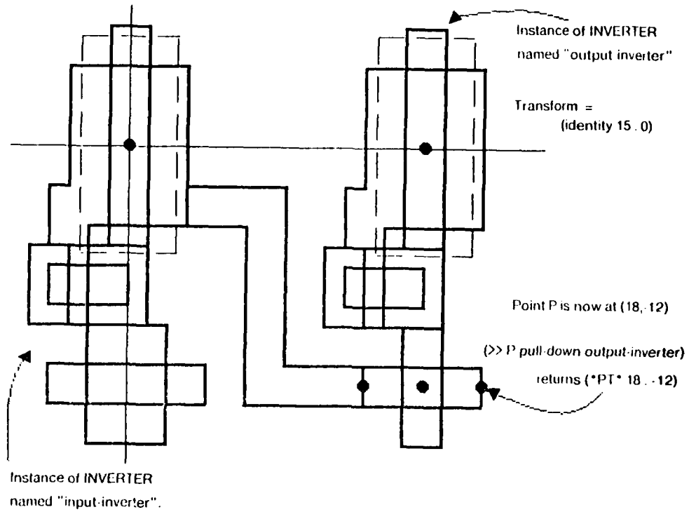
Figure 2C -- Buffer
