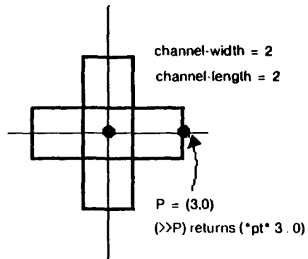
Figure 2A -- pass-transistor
