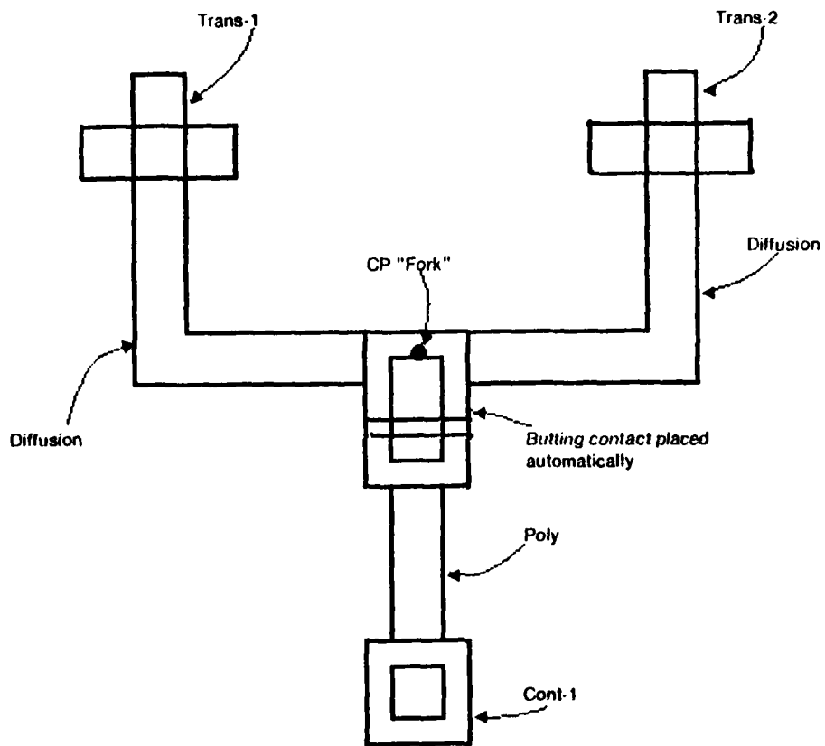
Figure 8 -- Wire System Example
