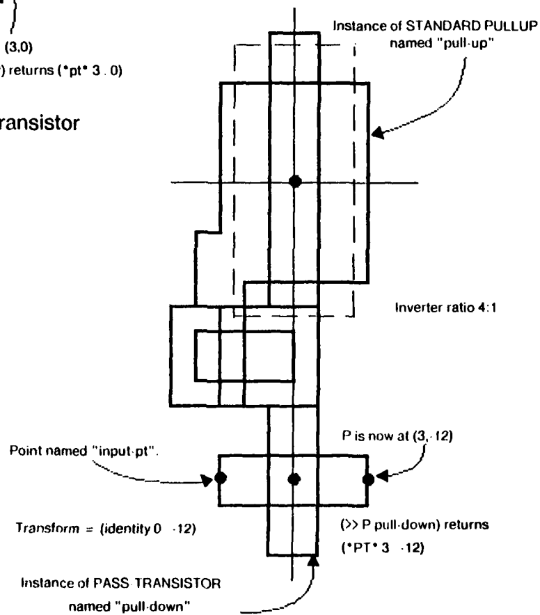
Figure 2B -- Inverter
