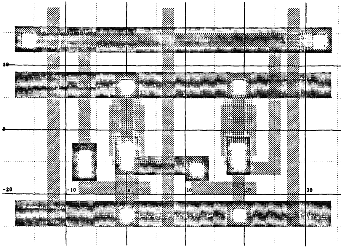
Figure 10 -- The REGCELL
