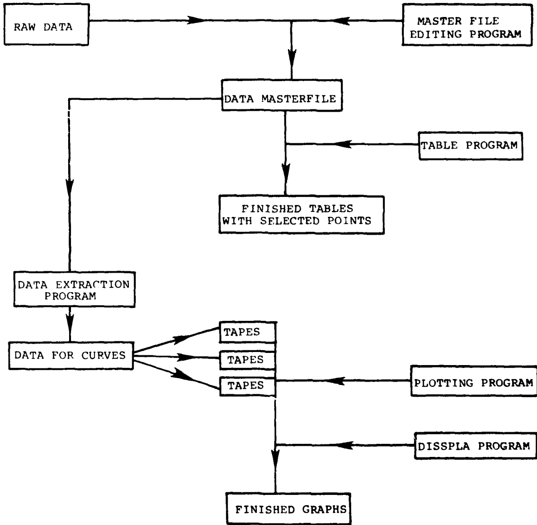
FIGURE 2 DATA FLOW CHART
