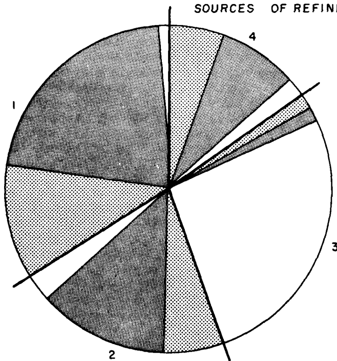
Fig. 14 - Sources of crude petroleum and refined products used in PAD Districts I and V in 1972. Size of circle is proportionate to quantities consumed.
