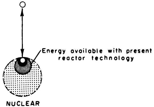
Fig. 16A (opposite) and 16B (above) - Sources of energy considered to have greatest potential. Area of circle is proportional to calculated energy content of the total resource base. Resource base estimates are from Theobald et al. (1972). Conversion to Btu is based on factors shown in table 3.
